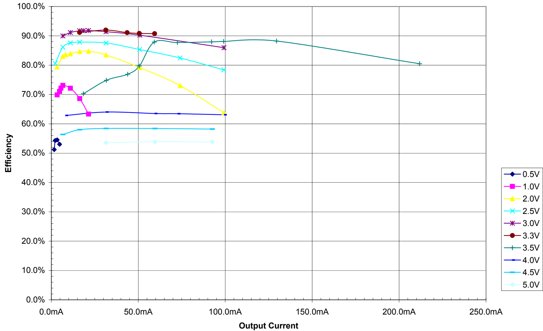
Measured 3.3V out Converter Efficiency vs Output Current for Varying Input Voltages
