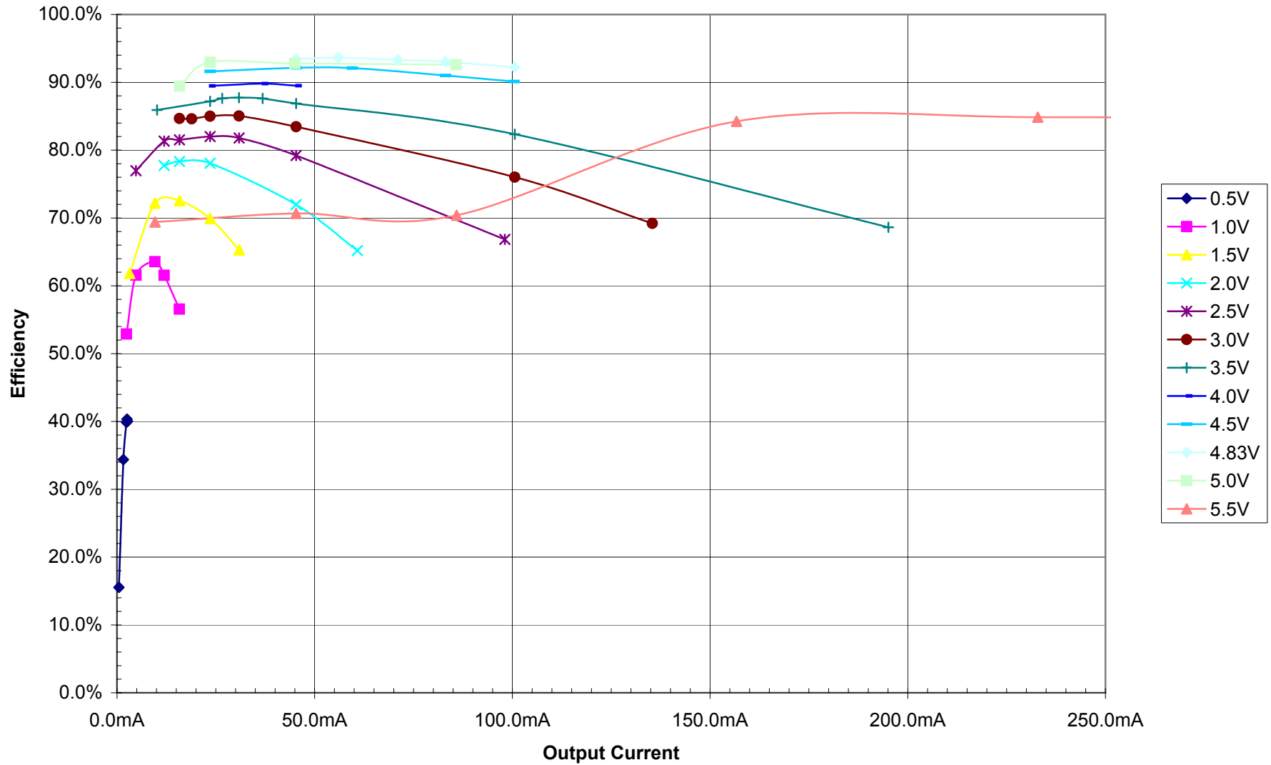
5.0V Measured Converter Efficiency vs. Output Current at Several Input Voltages
