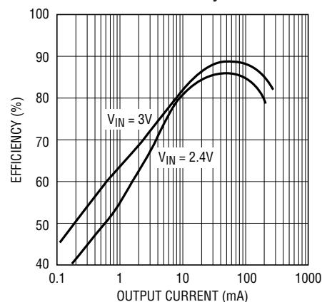
2-Cell to 5V Efficiency
