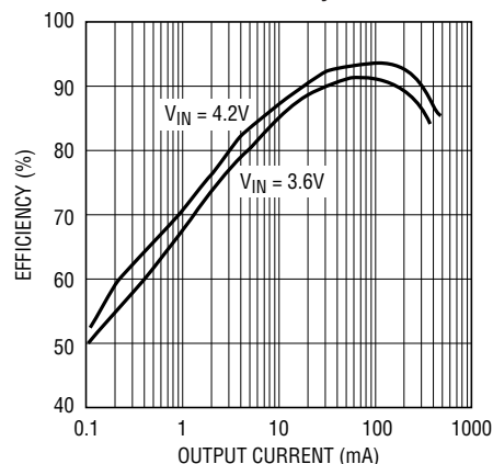
Li-Ion to 5V Efficiency
