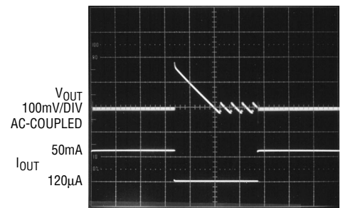
Fixed Frequency and Burst Mode Operation
