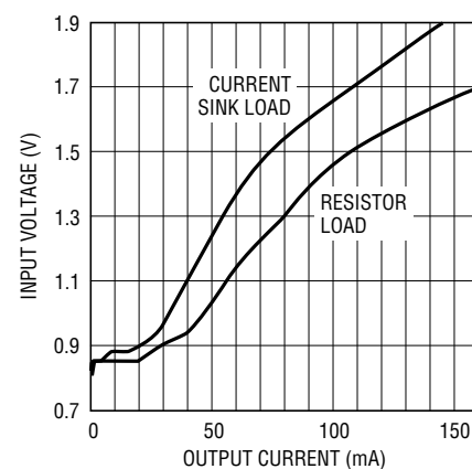
Minimum Start-Up Input Voltage vs Load Current
