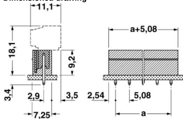
Dimensioned drawing
