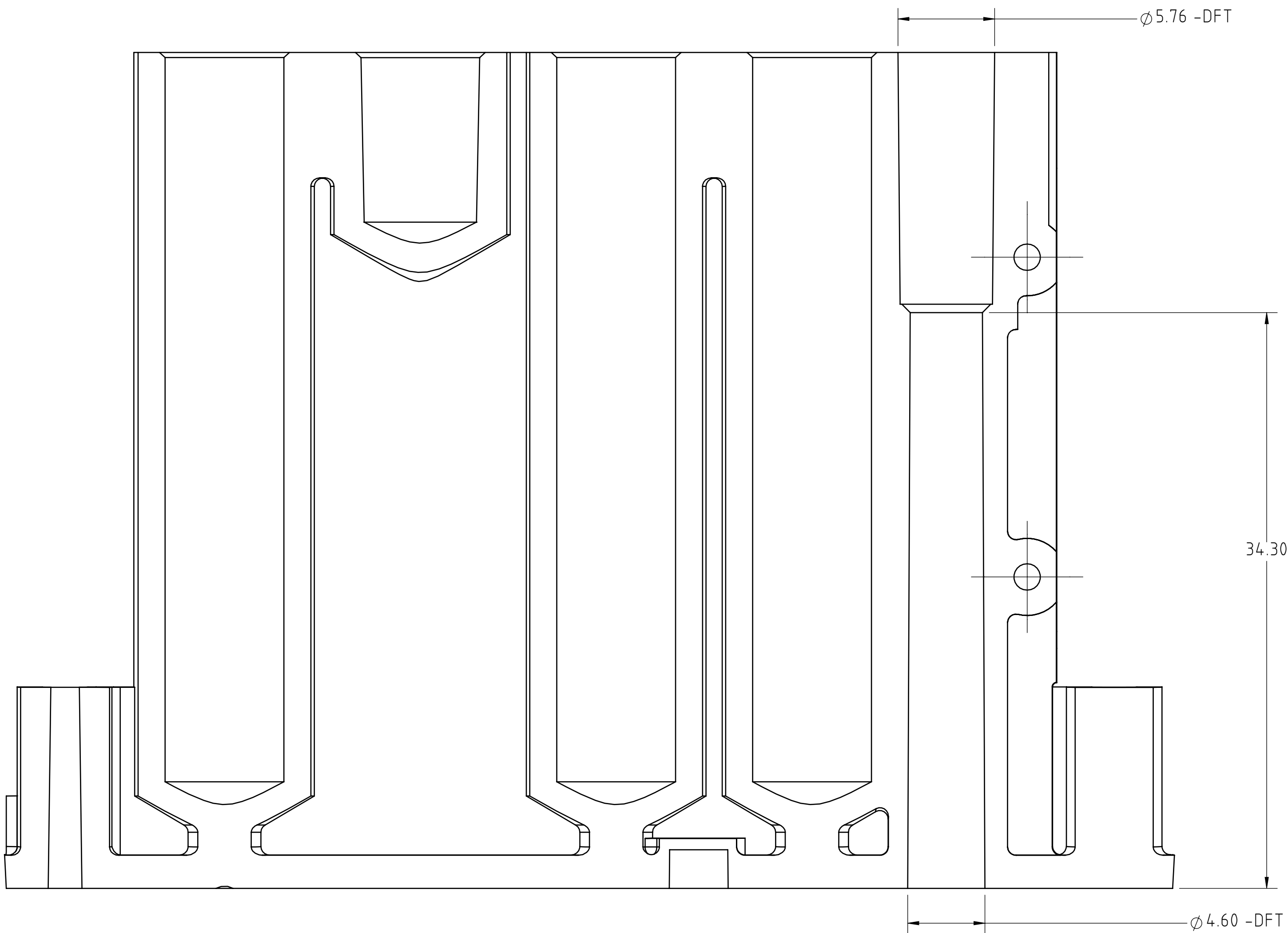
SECTION B-B
