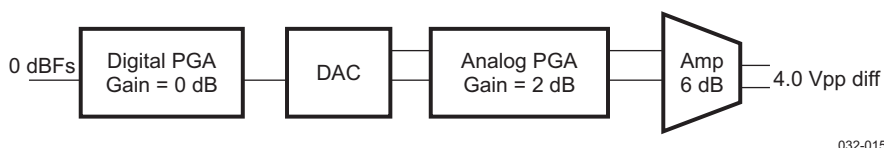
Figure 6-2. Earphone Amplifier
