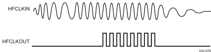
Figure 12-15. HFCLKOUT Behavior
