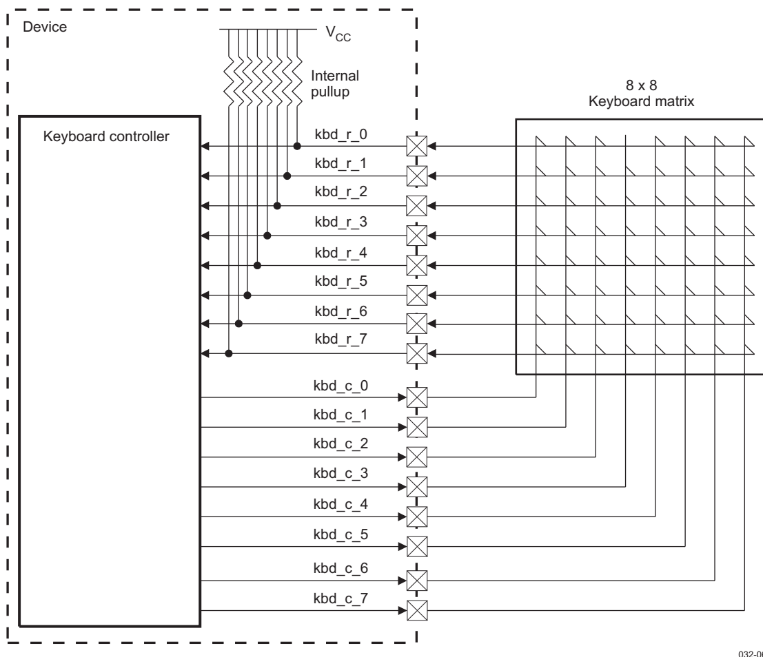
Figure 11-1. Keyboard Connection
