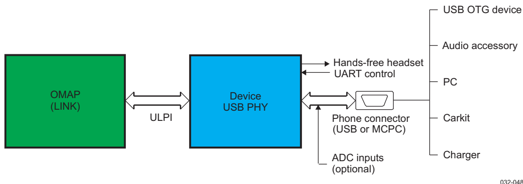
Figure 7-1. USB 2.0 PHY Overview
