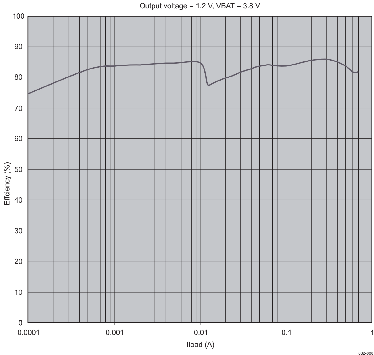
Figure 4-6. VIO dc-dc Regulator Efficiency in Active Mode
