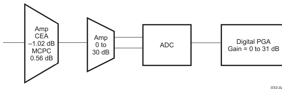
Figure 6-28. Carkit Input Uplink Path Characteristics
