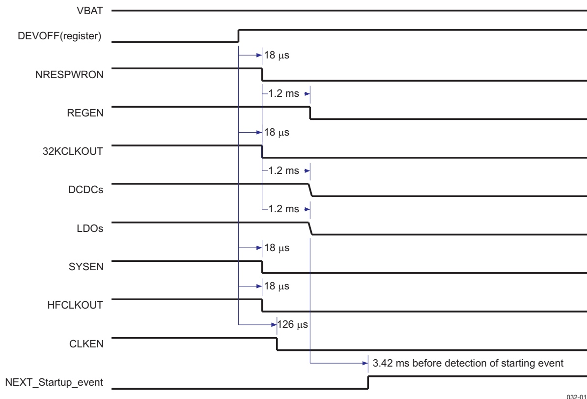
Figure 4-12. Power-Off Sequence in Master Modes
