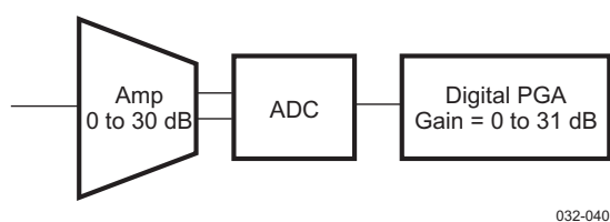
Figure 6-27. Uplink Amplifier
