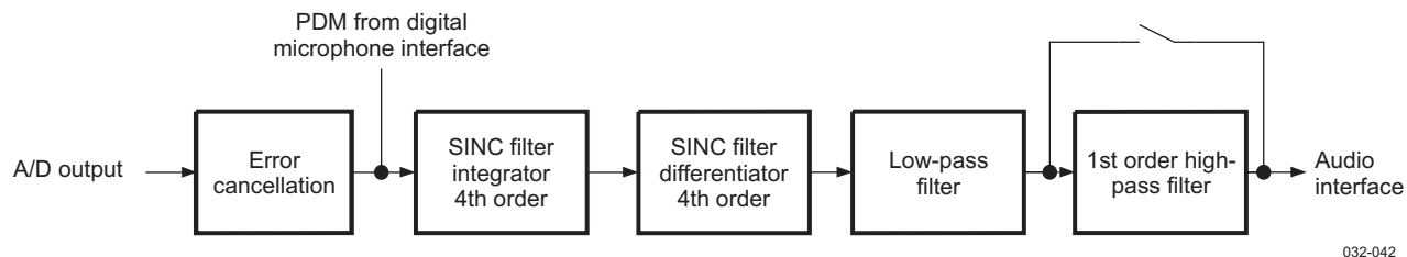
Figure 6-29. Digital Audio Filter Uplink Path Characteristics
