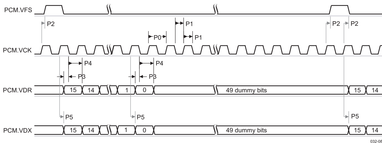
Figure 13-5. Voice/BT PCM Interface—Master Mode (Mode 1)
