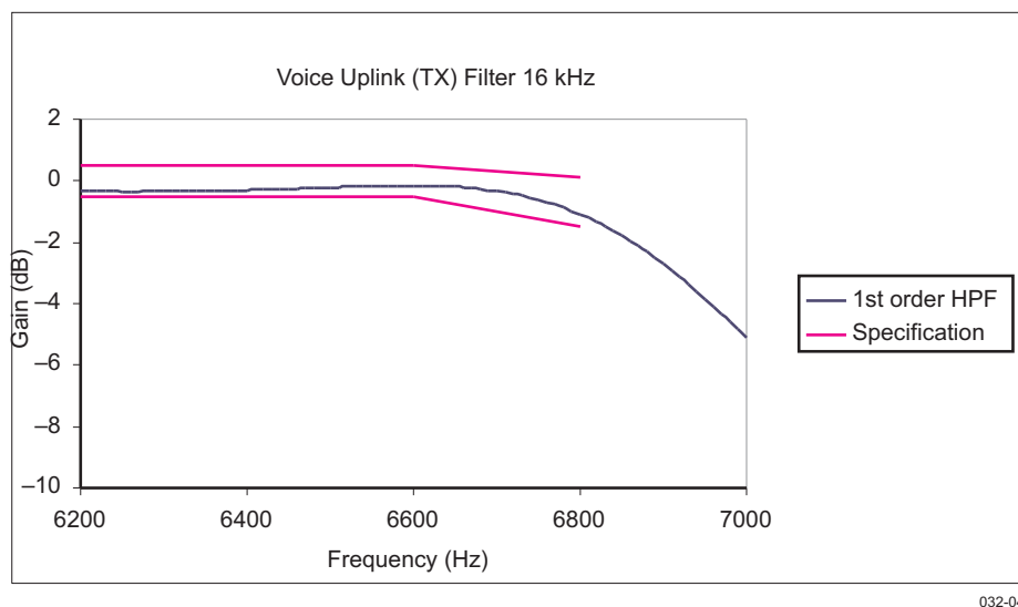
Figure 6-34. Voice Uplink Frequency Response With F_s = 16 kHz (Frequency Range 6200 to 7000 Hz)
