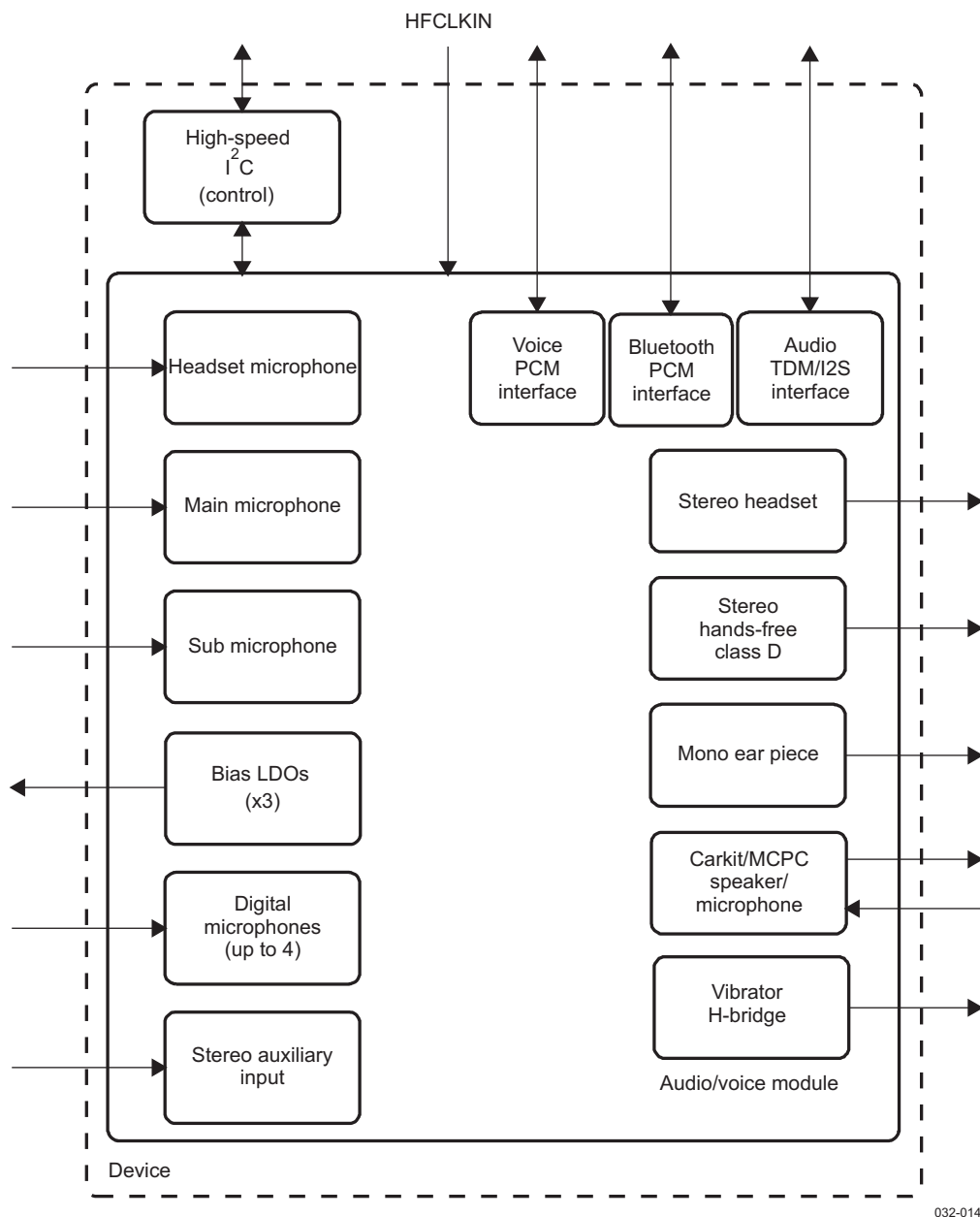
Figure 6-1. Audio/Voice Module Block Diagram
