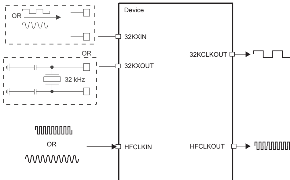
Figure 12-1. Clock Overview
