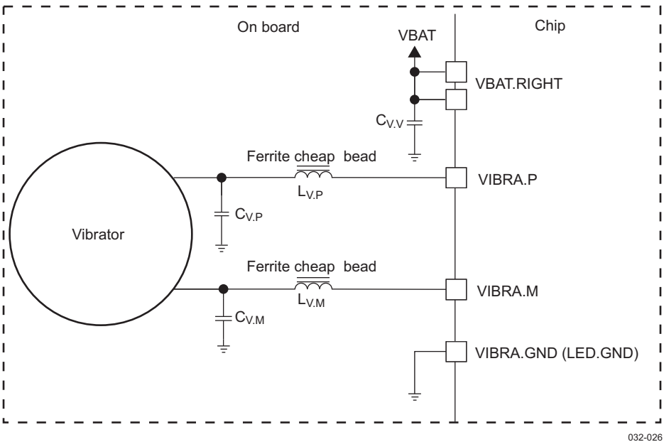
Figure 6-13. Vibrator H-Bridge
