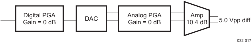
Figure 6-4. 8-Ω Stereo Hands-Free Amplifiers
