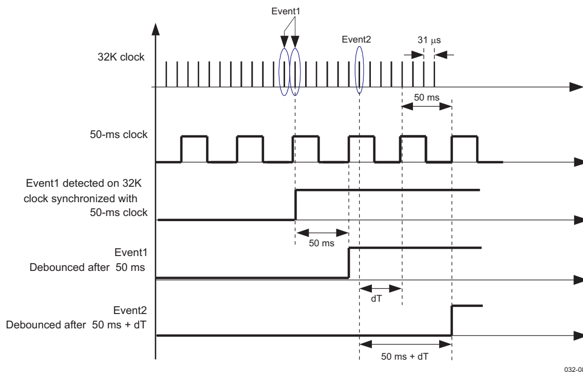
Figure 14-1. Debouncing Sequence Chronogram Example
