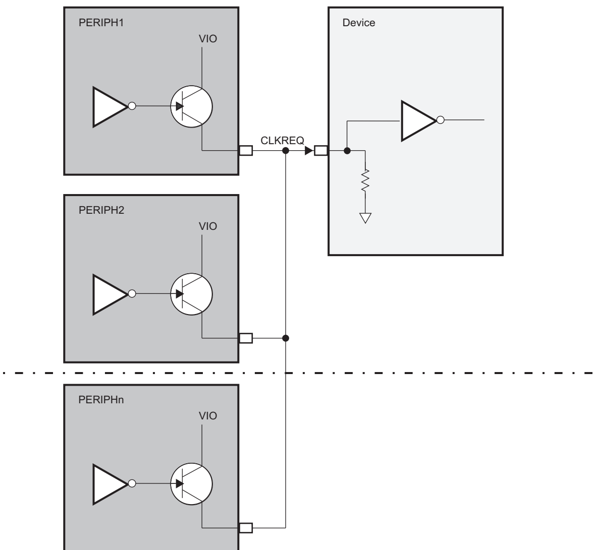
Figure 12-3. Example of Wired-OR Clock Request
