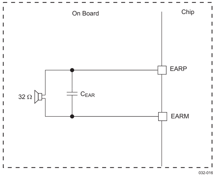
Figure 6-3. Earphone Speaker
