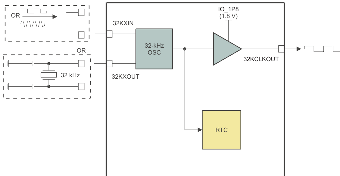
Figure 12-11. 32.768-kHz Clock Output Block Diagram
