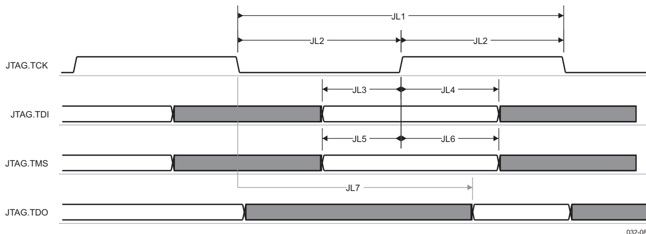
Figure 13-7. JTAG Interface Timing
