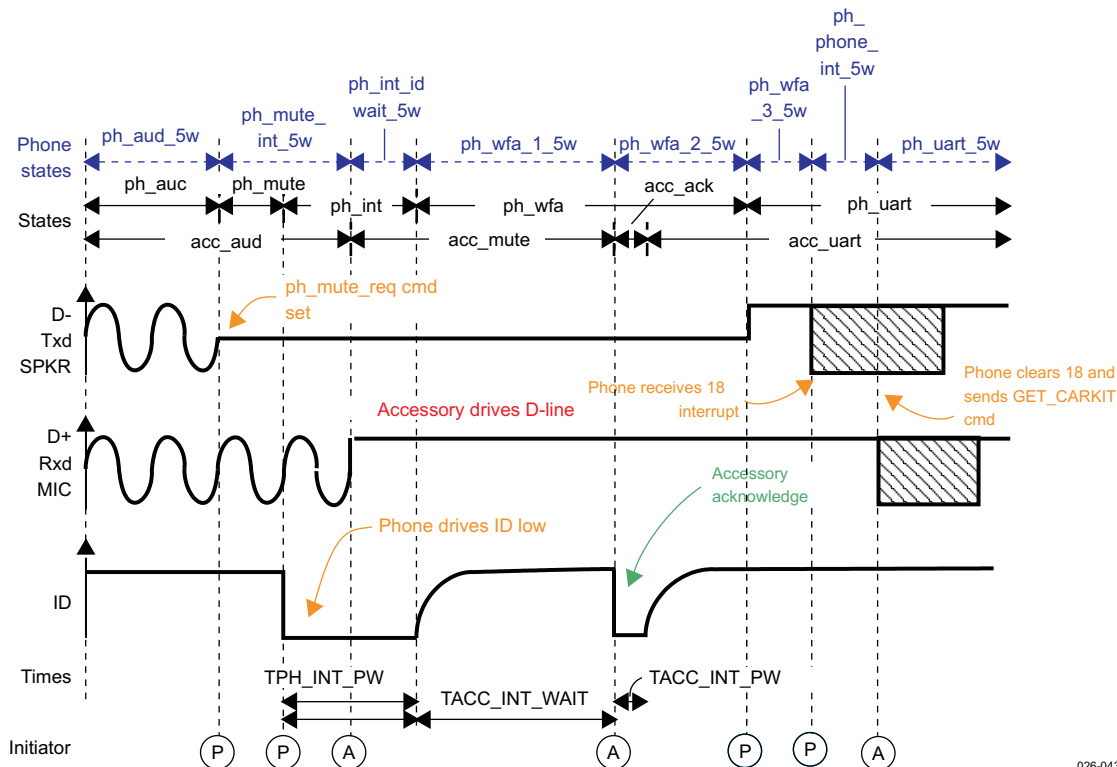
Figure 15-44. CEA Timing Diagram and PSM States: Phone to UART
