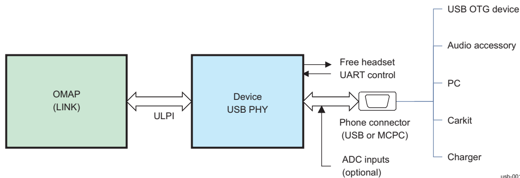
Figure 15-1. USB PHY
