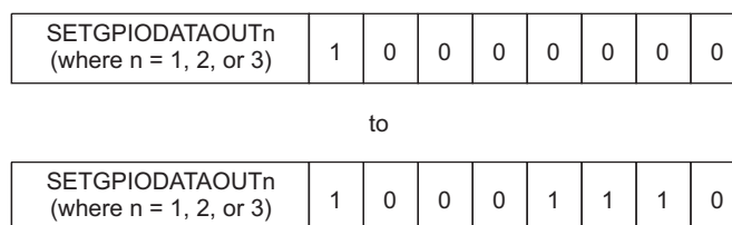
Figure 12-5. Write to SETGPIODATAOUT Register Example
