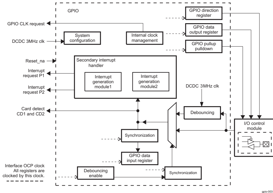
Figure 12-3. GPIO Block Diagram
