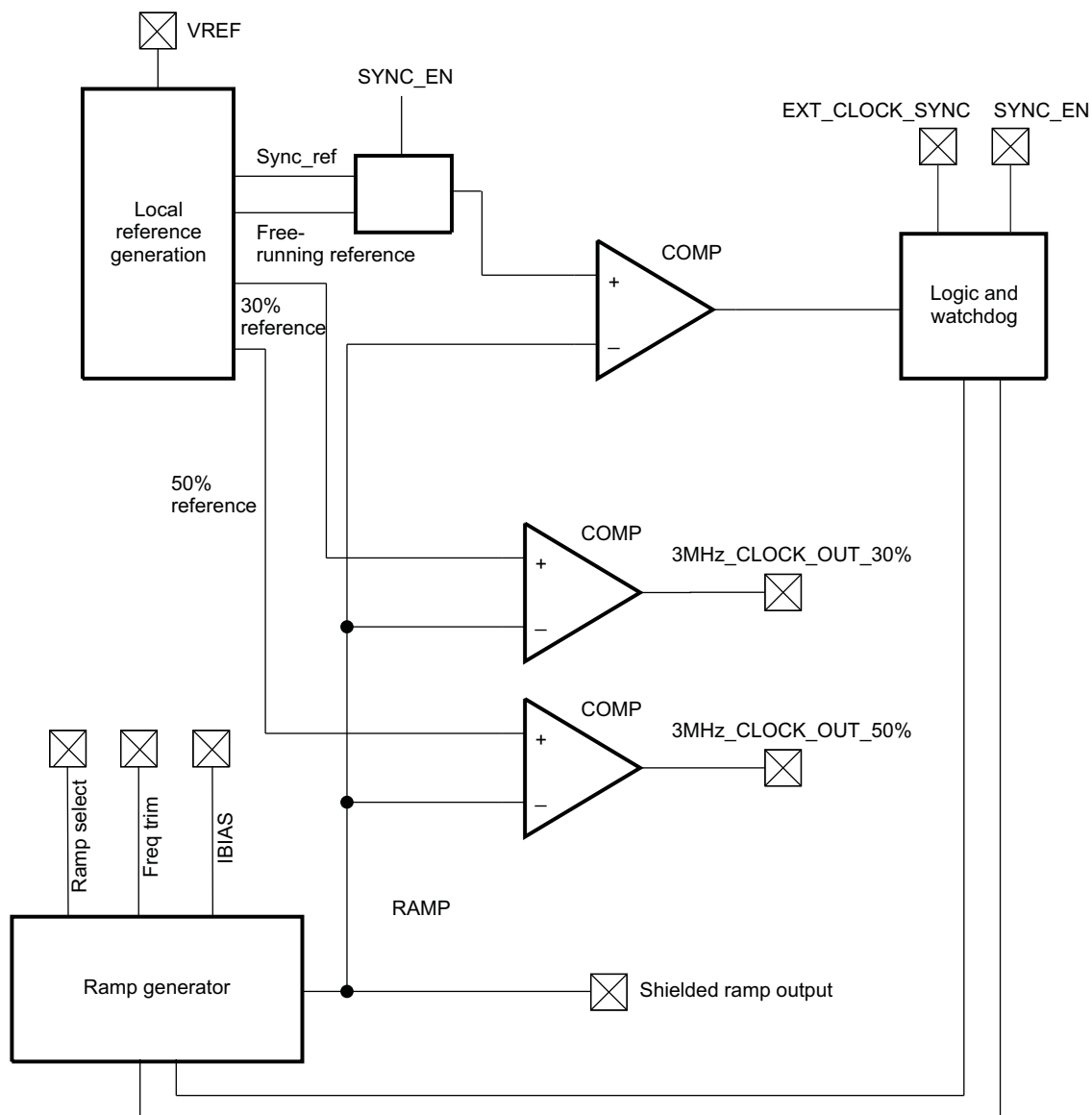
Figure 3-11. Ramp Generator Block Diagram
