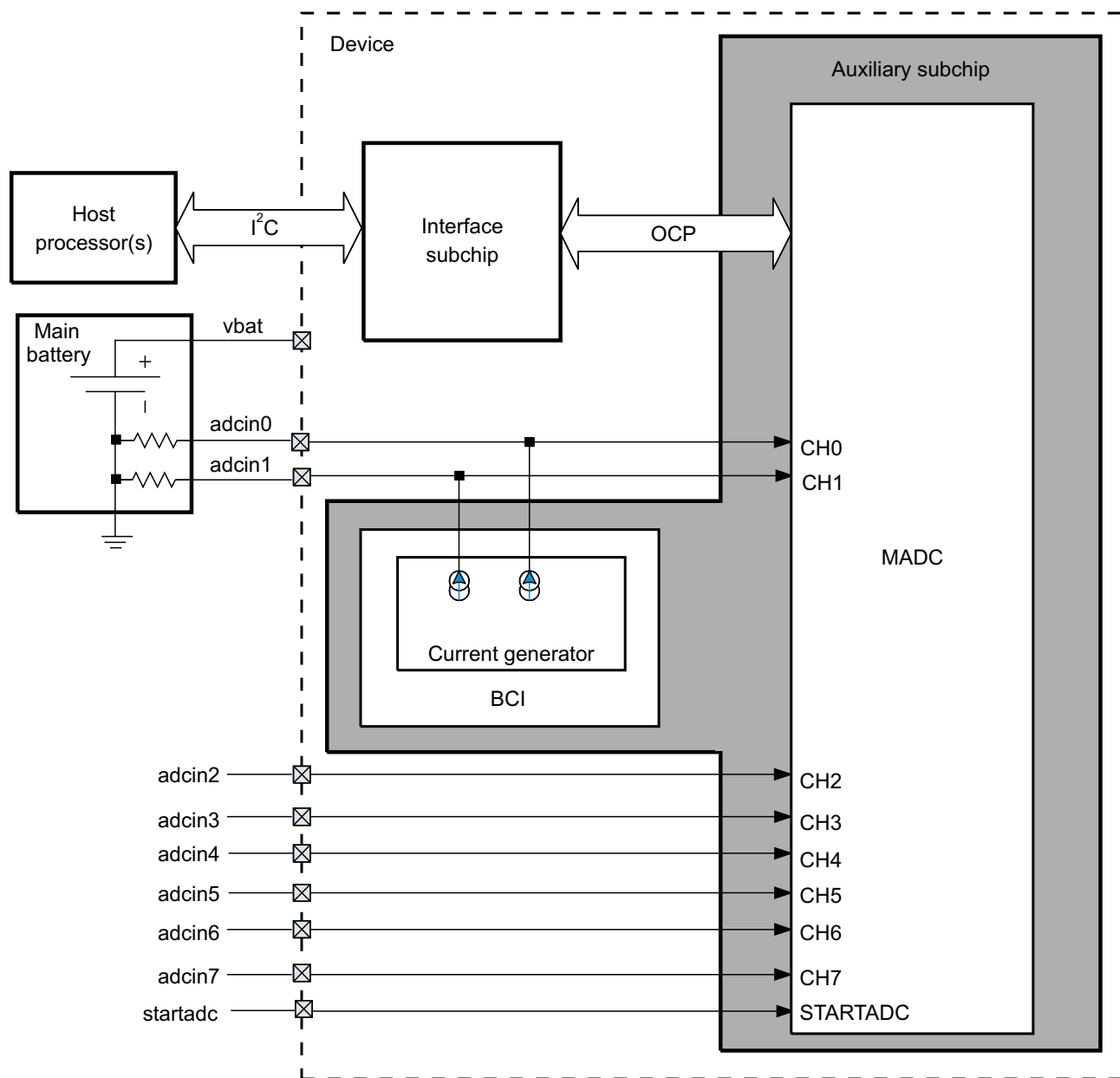
Figure 9-1. MADC Environment
