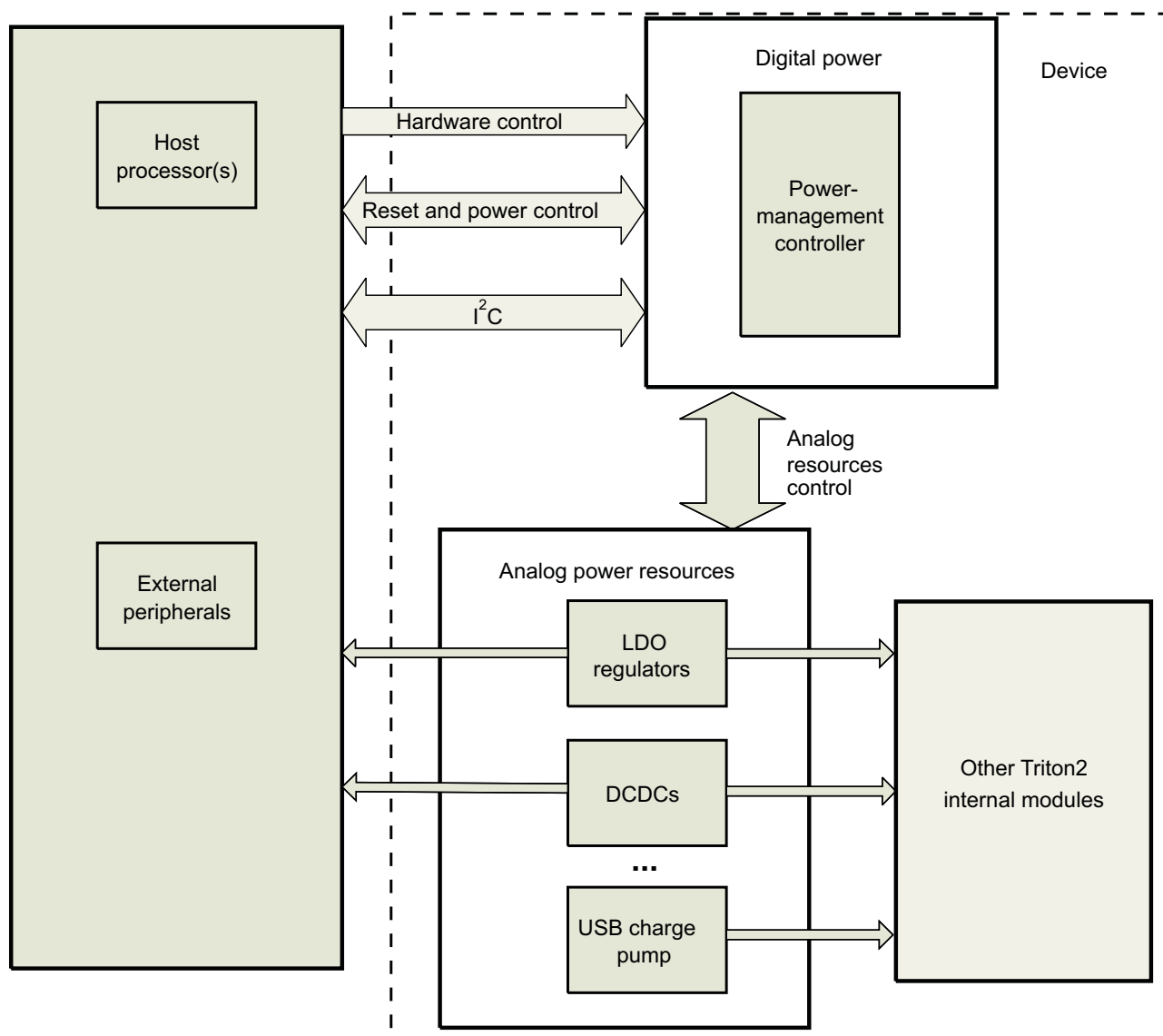
Figure 5-1. Device Power-Management System
