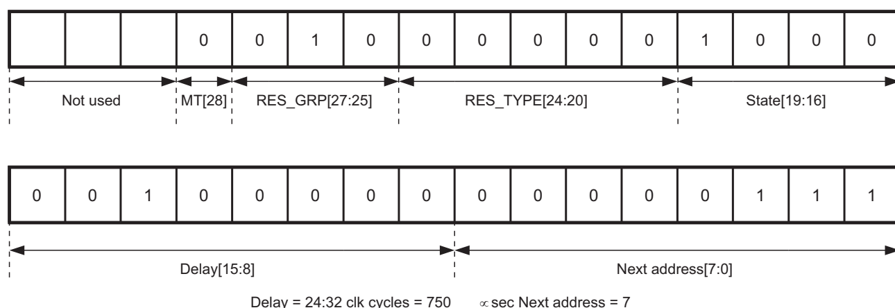
Figure 5-15. Adding a Delay—Modified Delay = 750 μs
