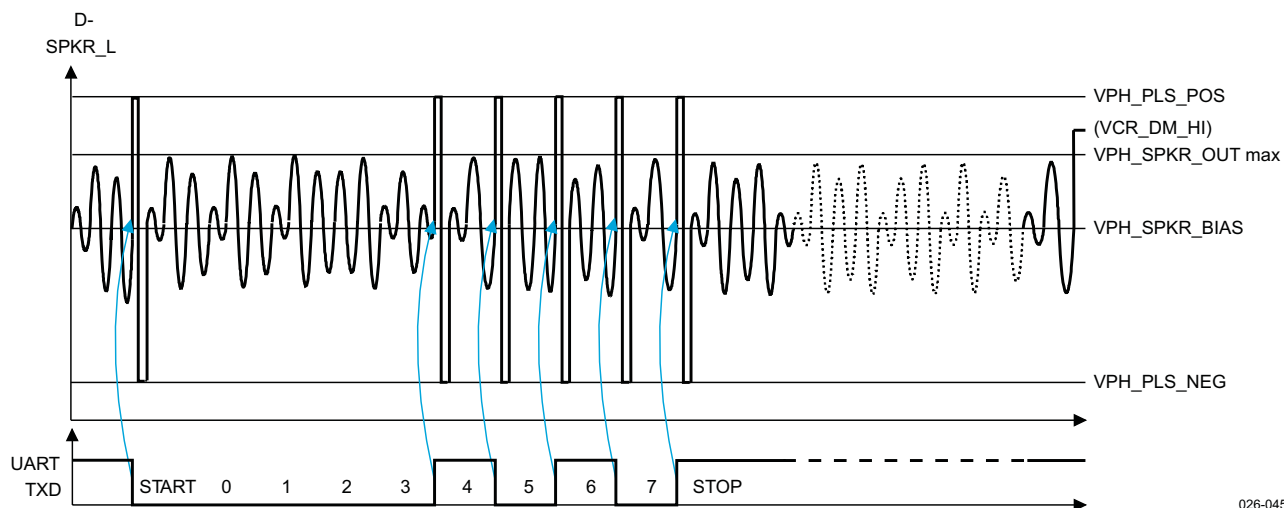
Figure 15-46. UART TX During Audio Signaling
