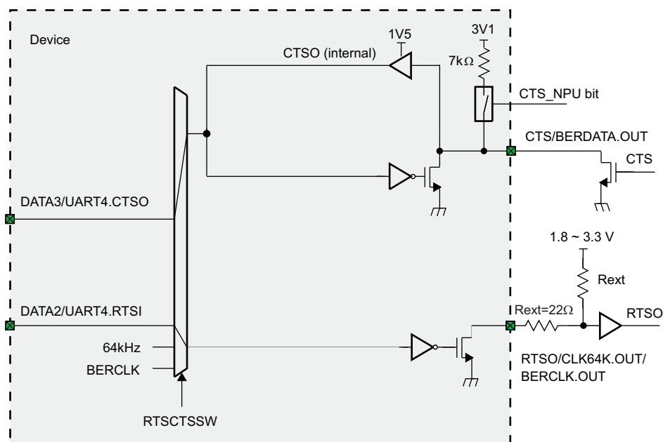
Figure 15-18. MCPC Mode 2: Hardware Handshake on CTSI and RTSO Pins
