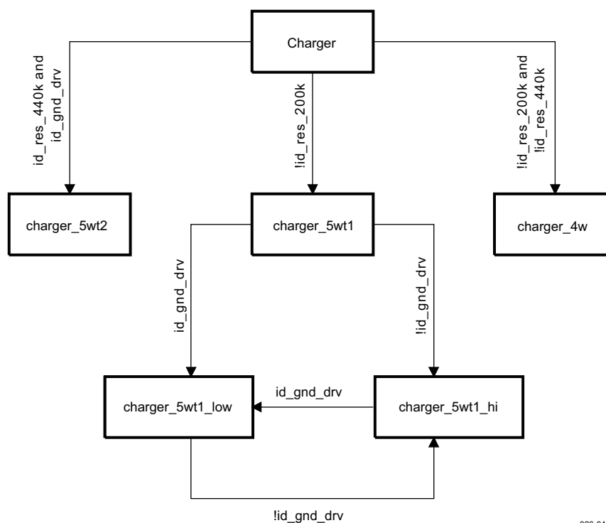
Figure 15-50. Charger State Diagram
