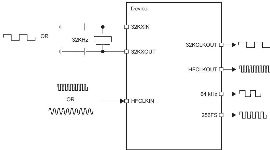
Figure 1-2. Clocks
