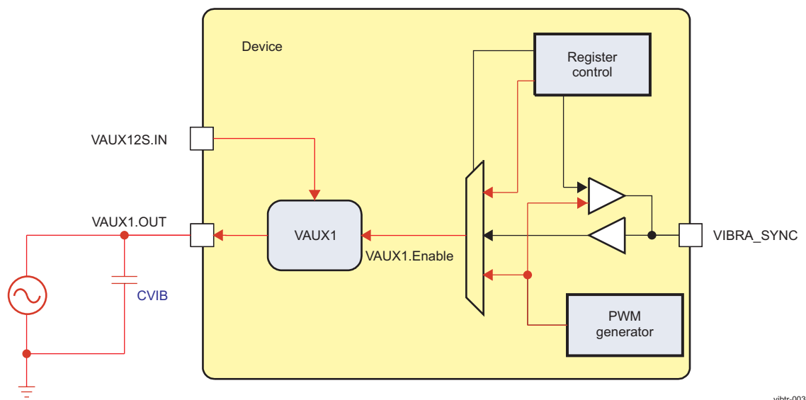
Figure 11-2. Vibrator Using VAUX1 LDO and PWM Control
