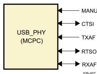
Figure 15-7. MCPC Signals
