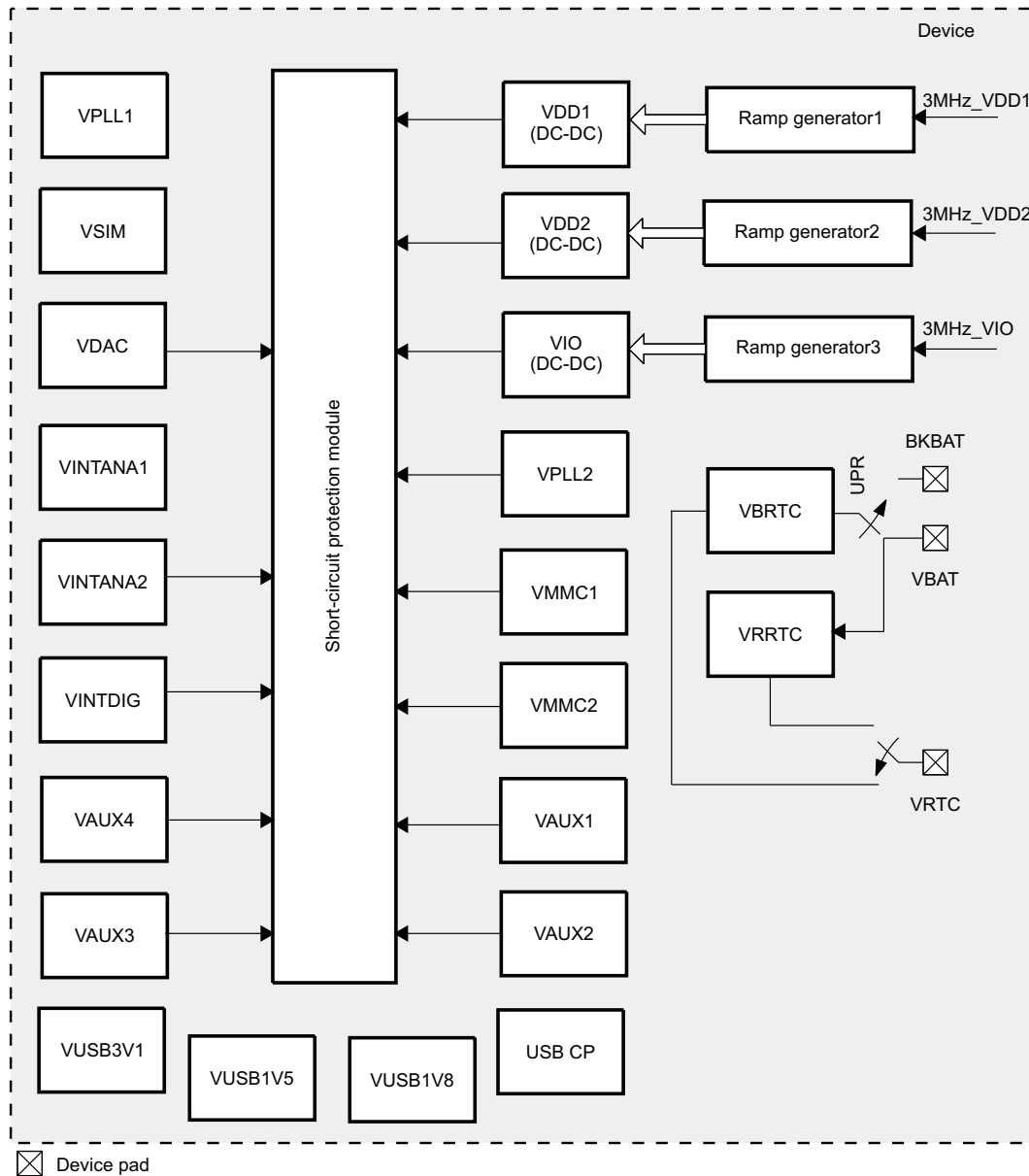
Figure 6-4. Power Resource Functional Description
