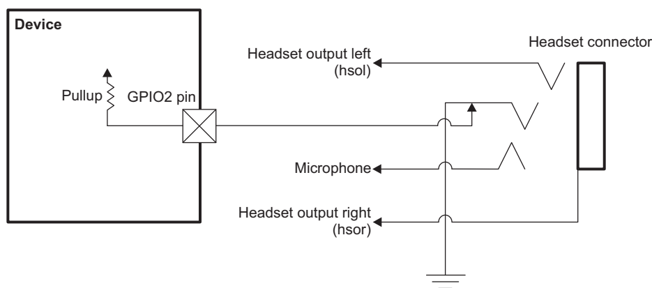
Figure 14-2. Stereo Data Communication With Digital Microphones
