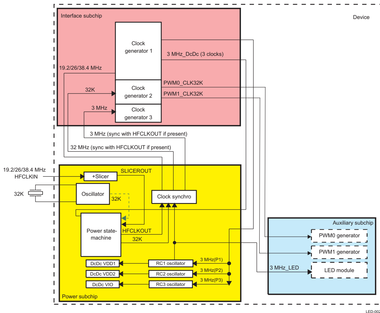
Figure 8-2. LED Driver and PWM Generator Integration
