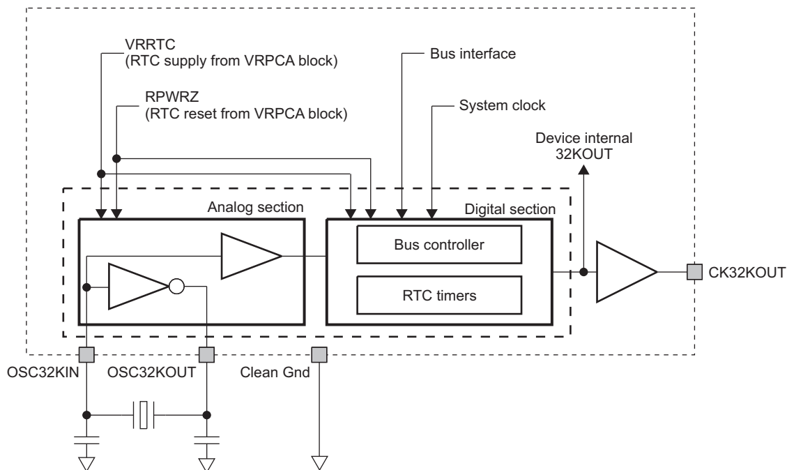
Figure 3-9. RTC
