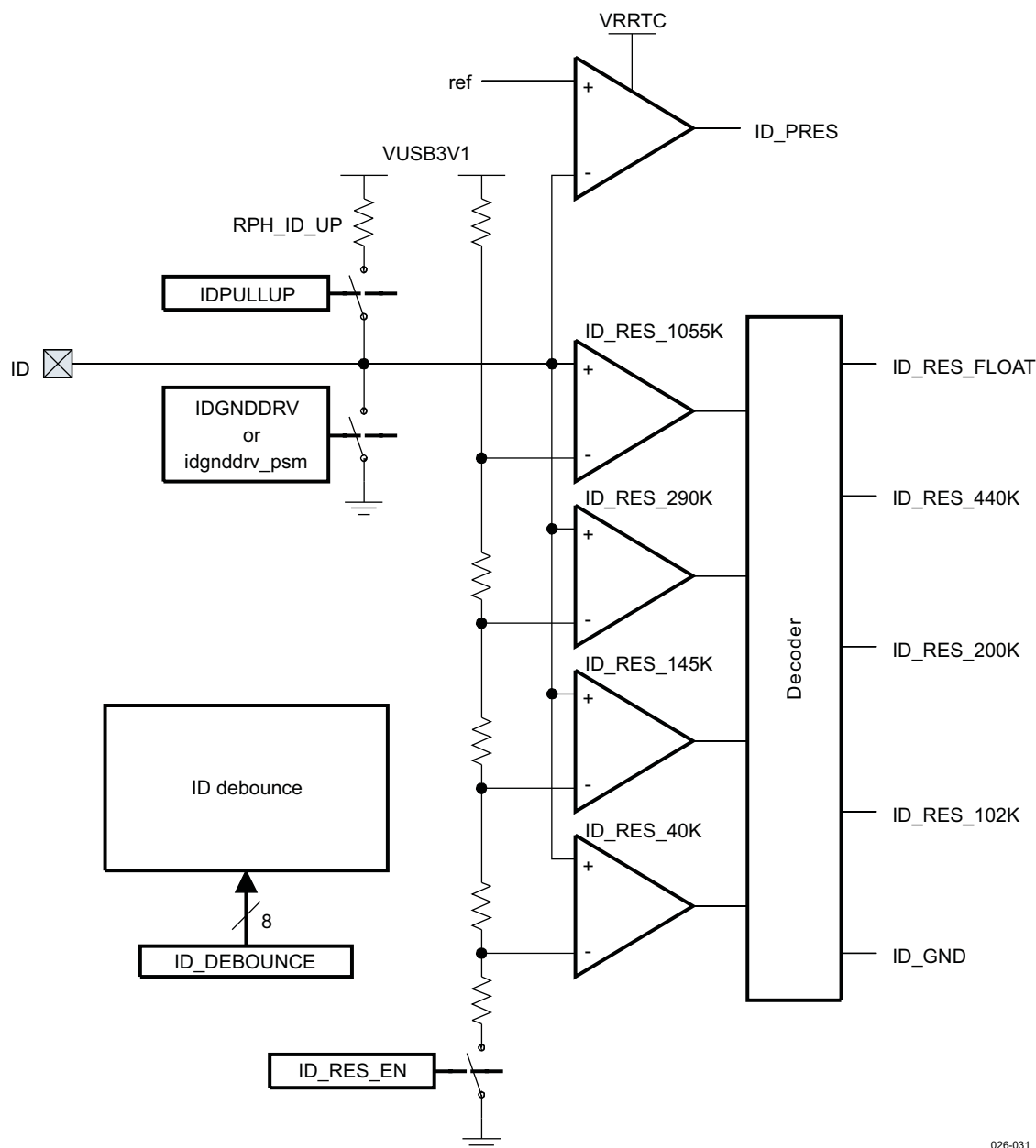
Figure 15-32. ID Control and Detection
