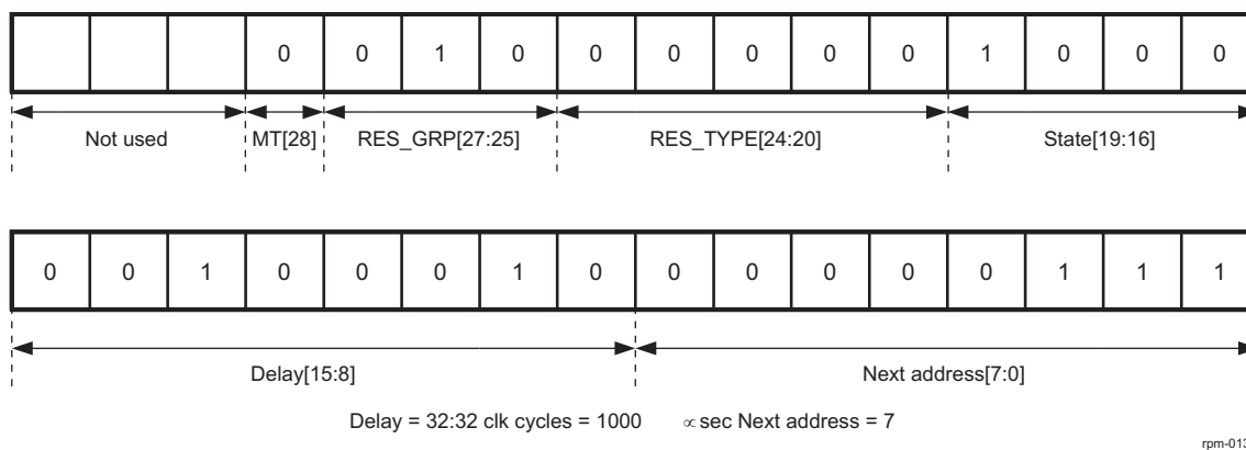
Figure 5-13. Skipping an Address—Modified Value = 7
