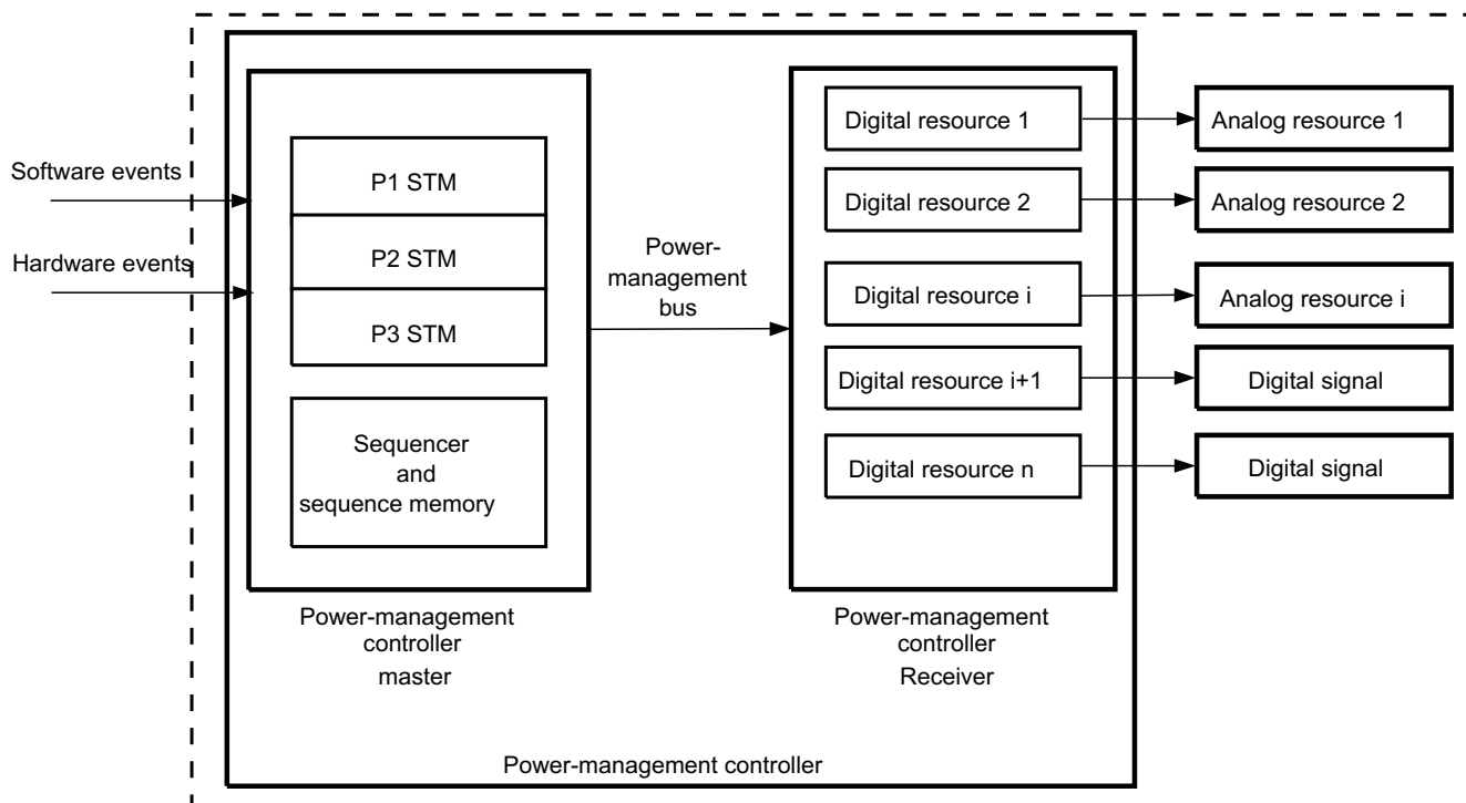
Figure 5-8. Power-Management State-Machine
