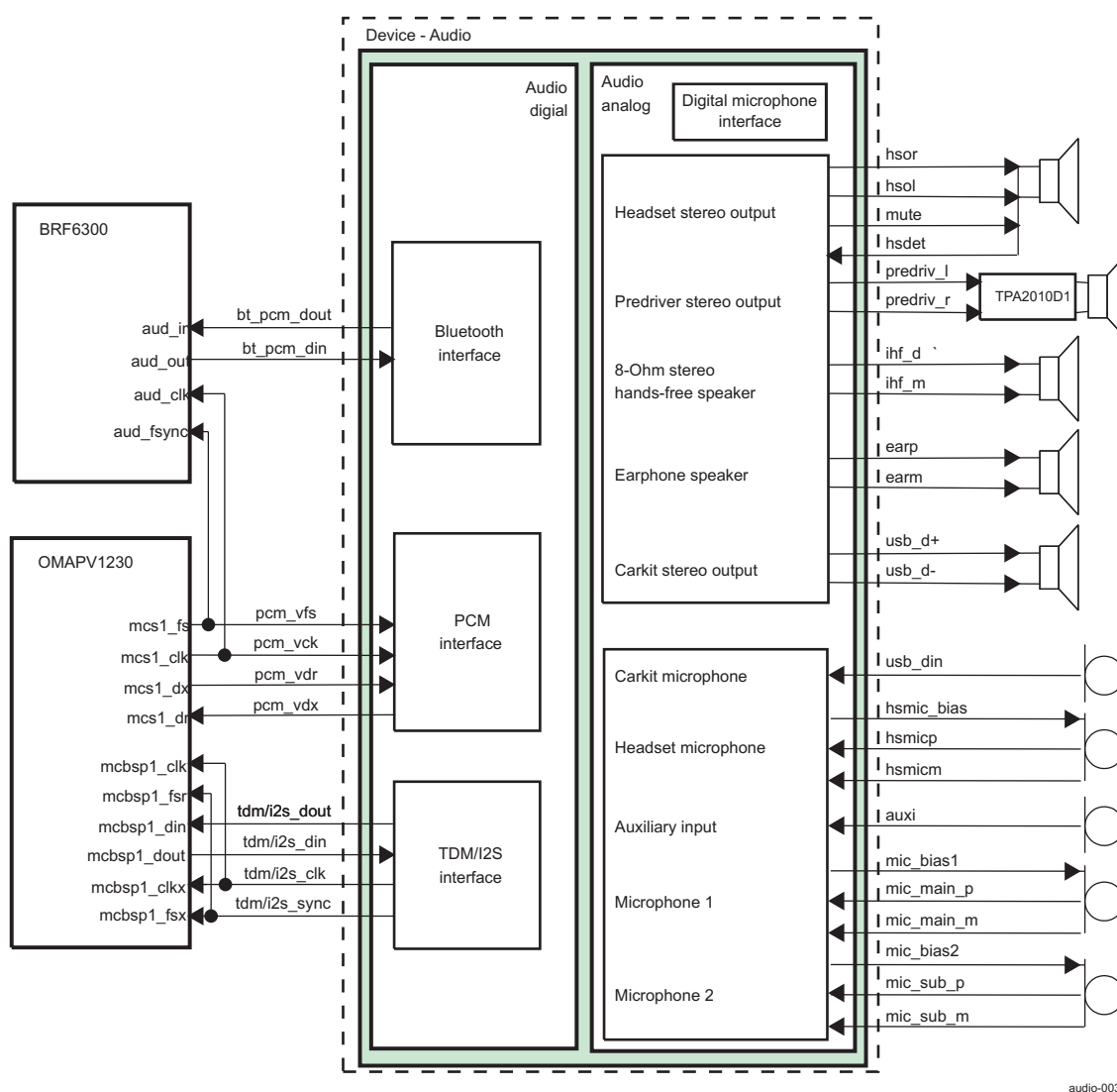
Figure 14-3. External Connections of the Audio Module to OMAPV1230 Application Processor and BRF6300 Bluetooth Radio Transceiver
