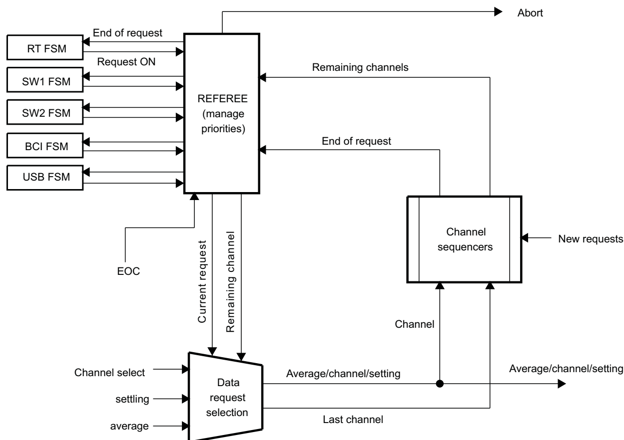
Figure 9-7. MADC REFEREE
