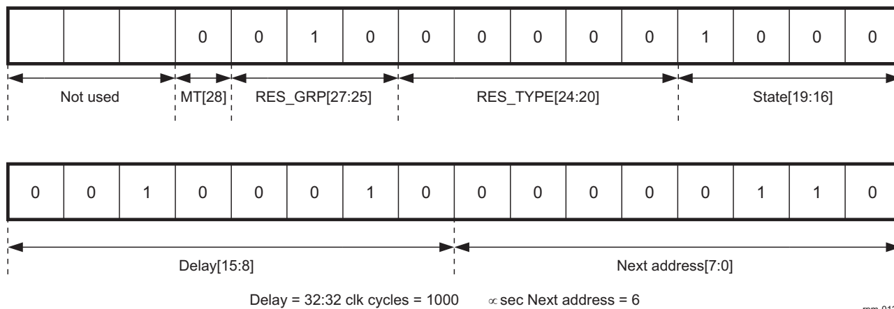
Figure 5-12. Skipping an Address—Original Address = 6
