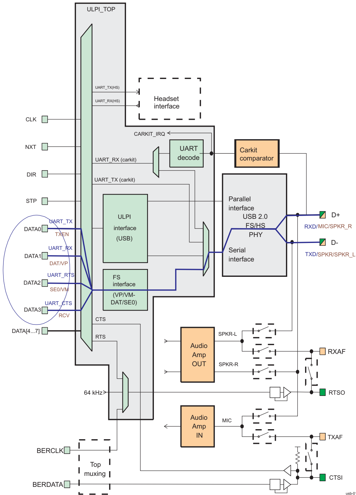
Figure 15-14. USB ULPI and CEA-2011 3-Pin and 4-Pin Serial Modes
