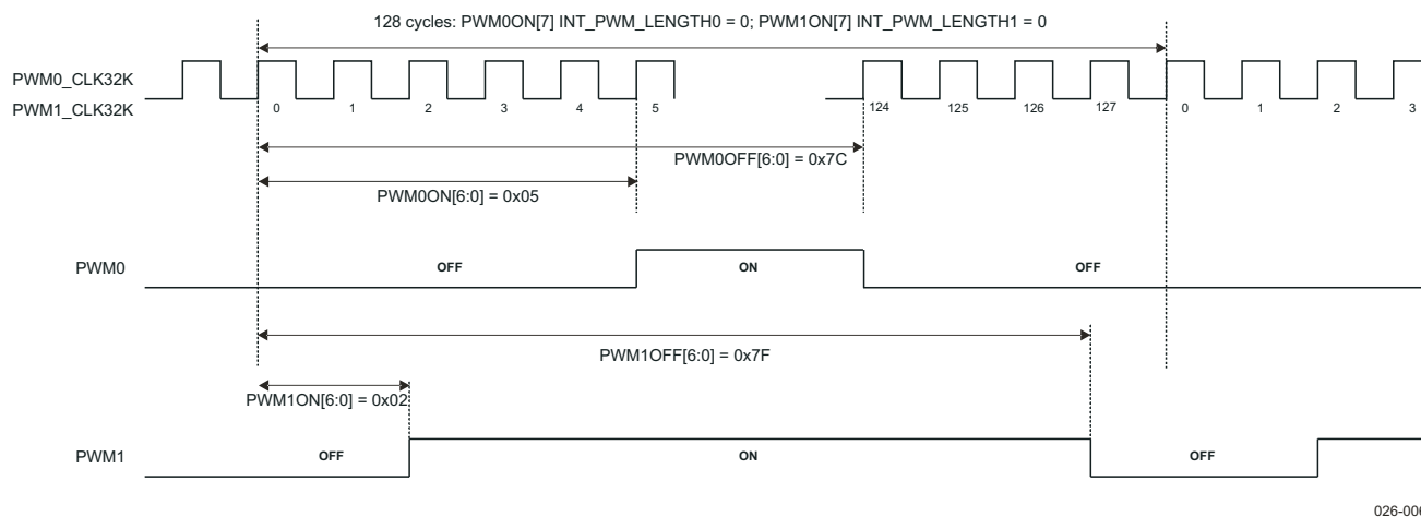
Figure 8-6. PWM Timings
