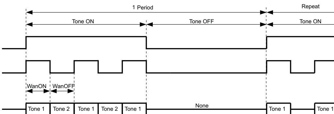
Figure 14-9. DTMF Dual-Tone Mode
