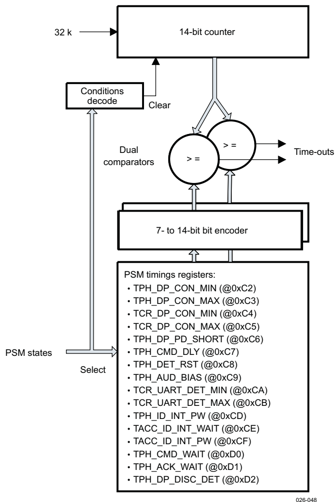
Figure 15-49. CEA Timers in the PSM
