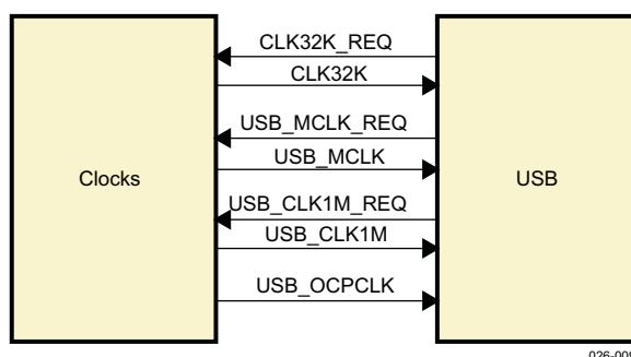
Figure 15-9. Interface With the Clock Module
