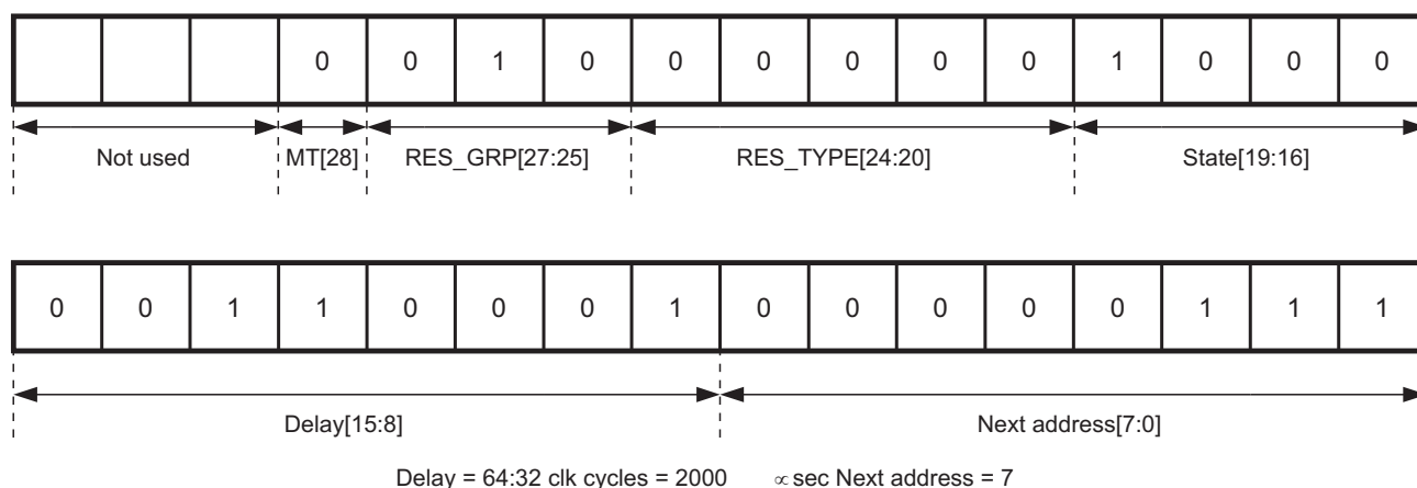
Figure 5-14. Adding a Delay—Original Delay = 2000 μs
