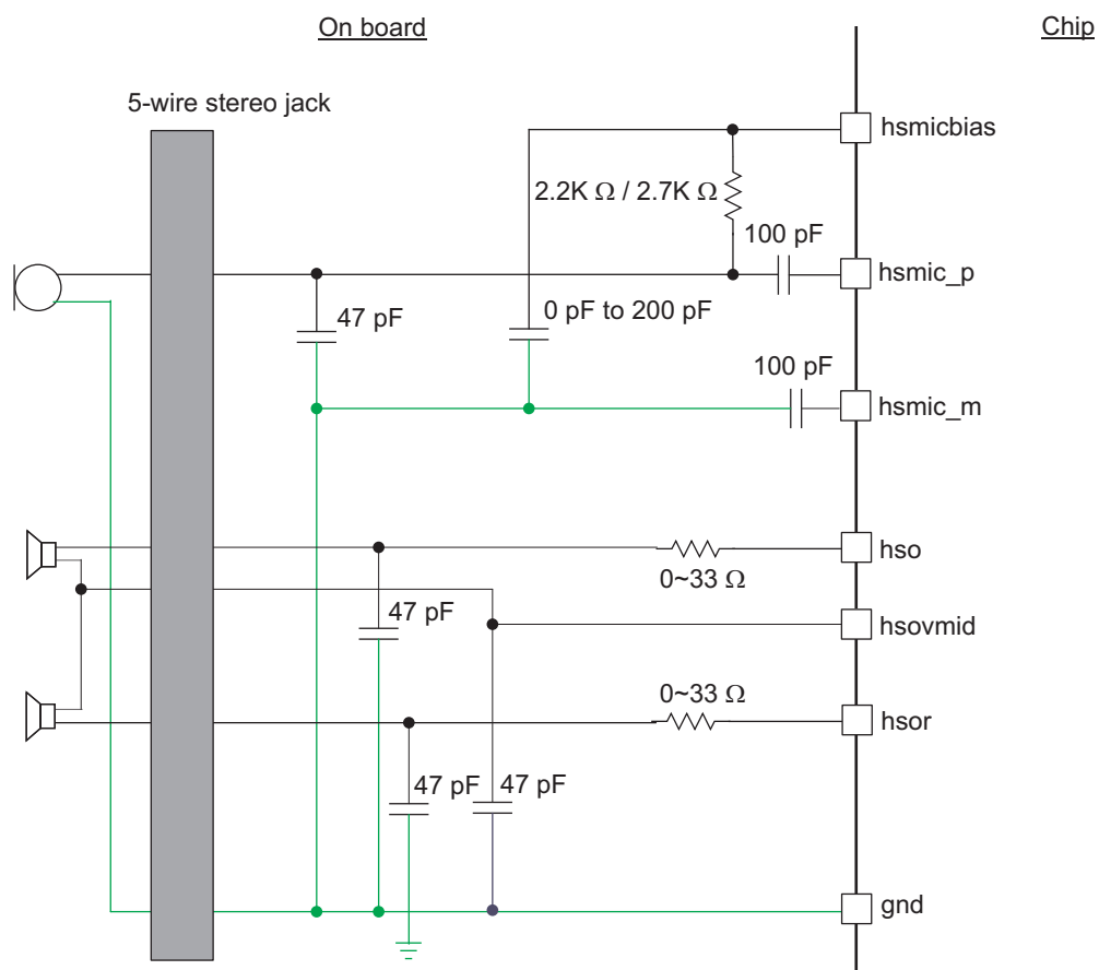
Figure 14-14. 5-Wire Headset Configuration
