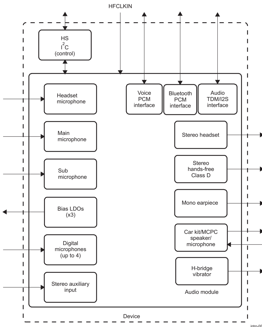
Figure 1-7. Device Audio Subsection
