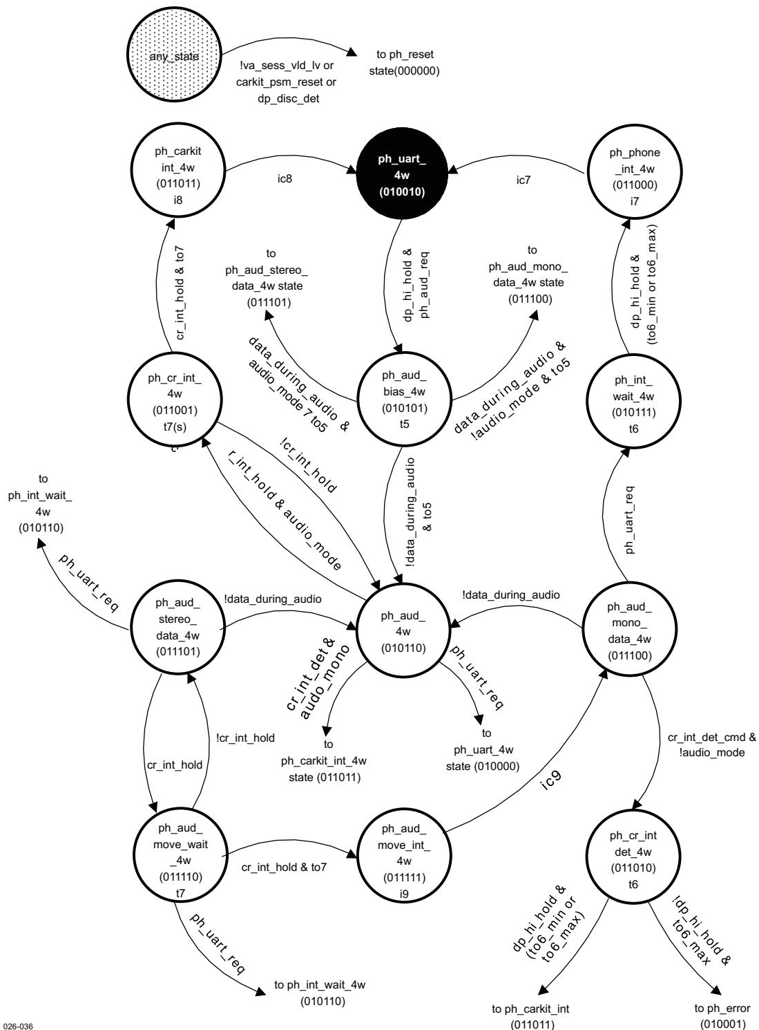
Figure 15-37. 4-Wire State Diagram
