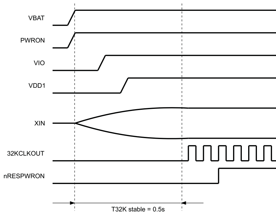
Figure 3-5. 32-kHz Oscillator Stabilization
