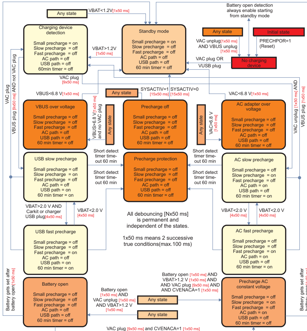
Figure 7-4. Precharge State-Machine
