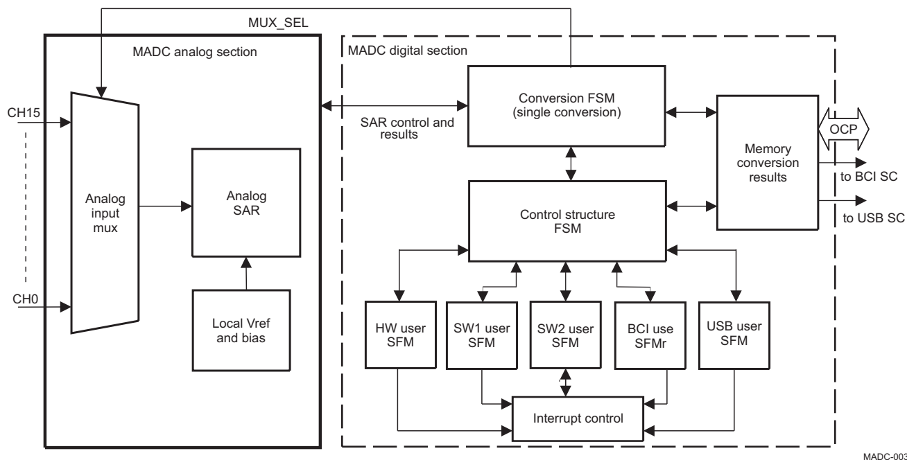
Figure 9-3. MADC Analog and Digital Sections
