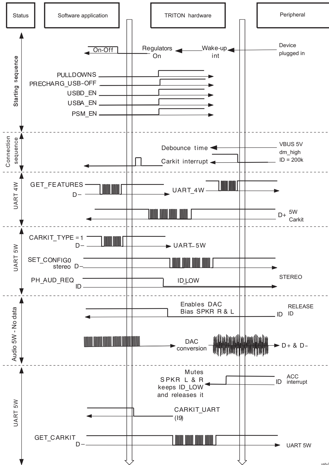
Figure 15-48. Programming Model
