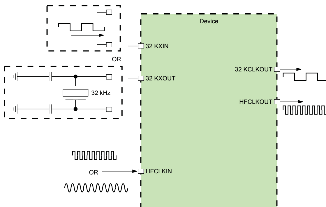
Figure 3-1. Clock Sources
