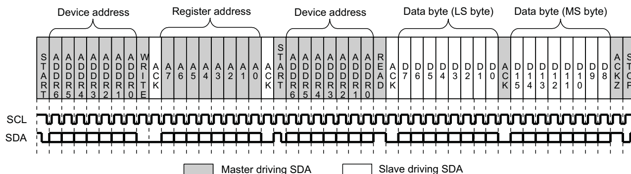
Figure 2-7. I 2 C 16-Bit Read Access
