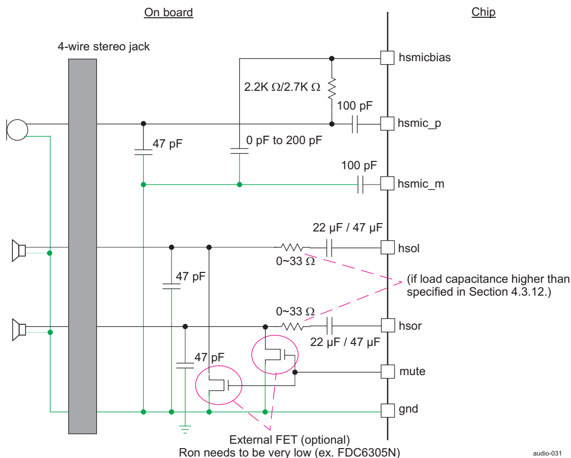
Figure 14-12. 4-Wire Headset Configuration
