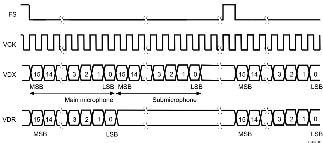
Figure 14-20. PCM Mode 1, 16 Bits, Stereo TX, Mono RX
