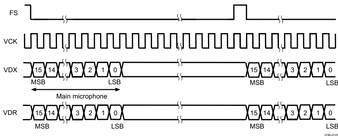
Figure 14-19. PCM Mode 1, 16 Bits, Mono TX, Mono RX
