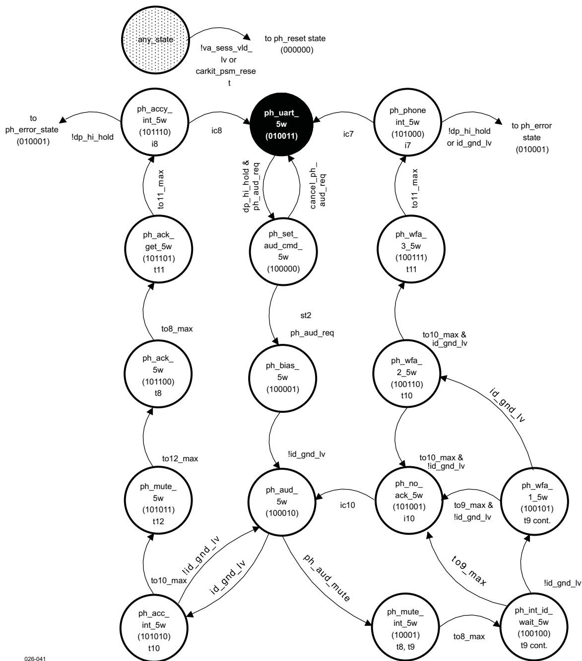
Figure 15-42. 5-Wire State Diagram
