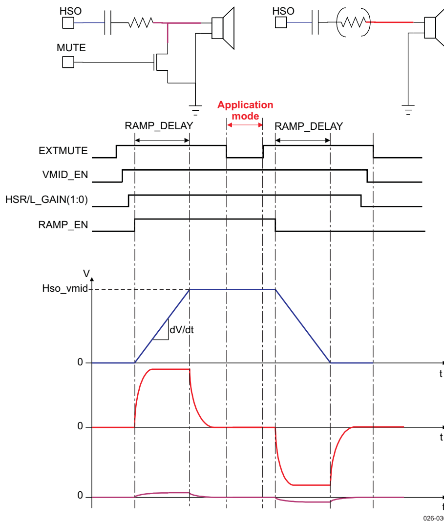
Figure 14-11. Headset Pop-Noise Attenuation Diagram
