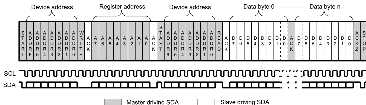
Figure 2-8. Burst Read Access
