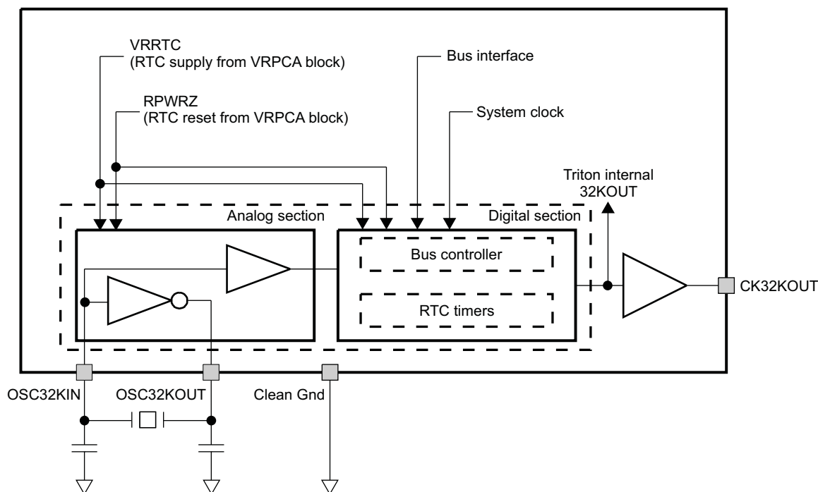
Figure 1-3. RTC
