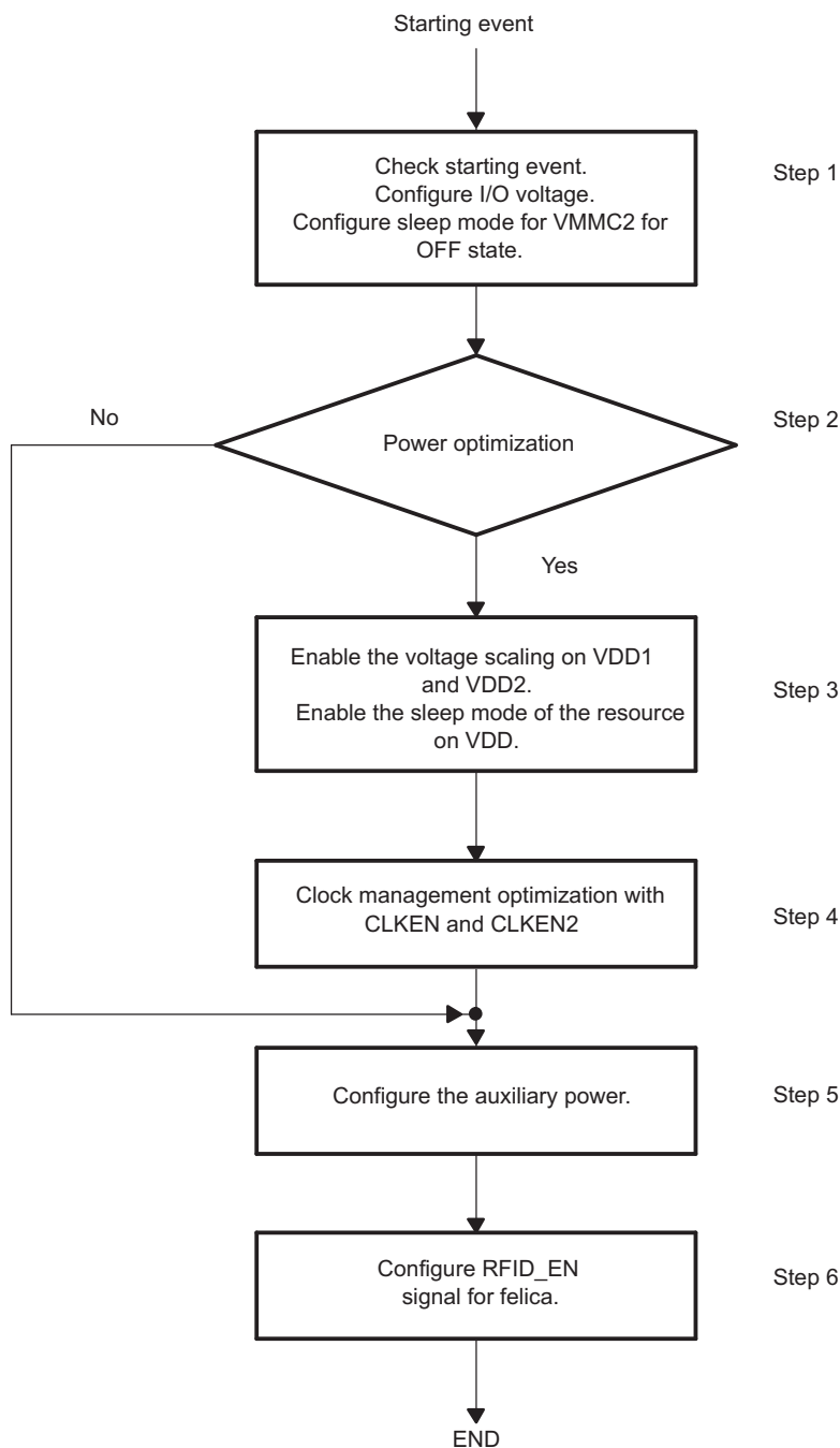
Figure 5-11. Sequencing Flowchart
