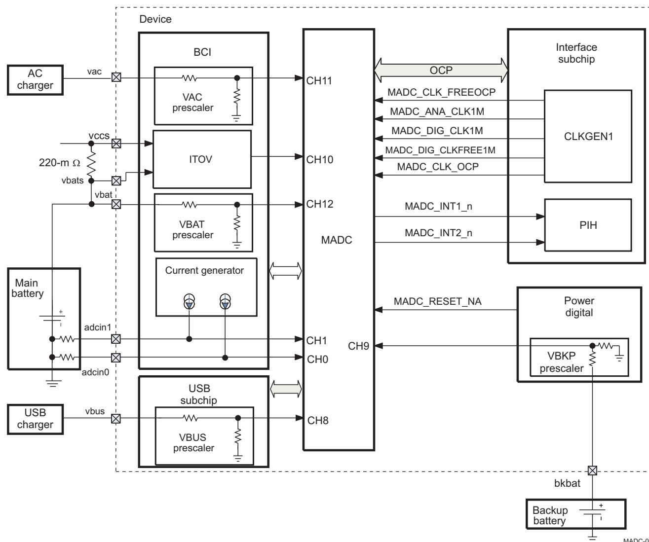
Figure 9-2. MADC Integration in the Device
