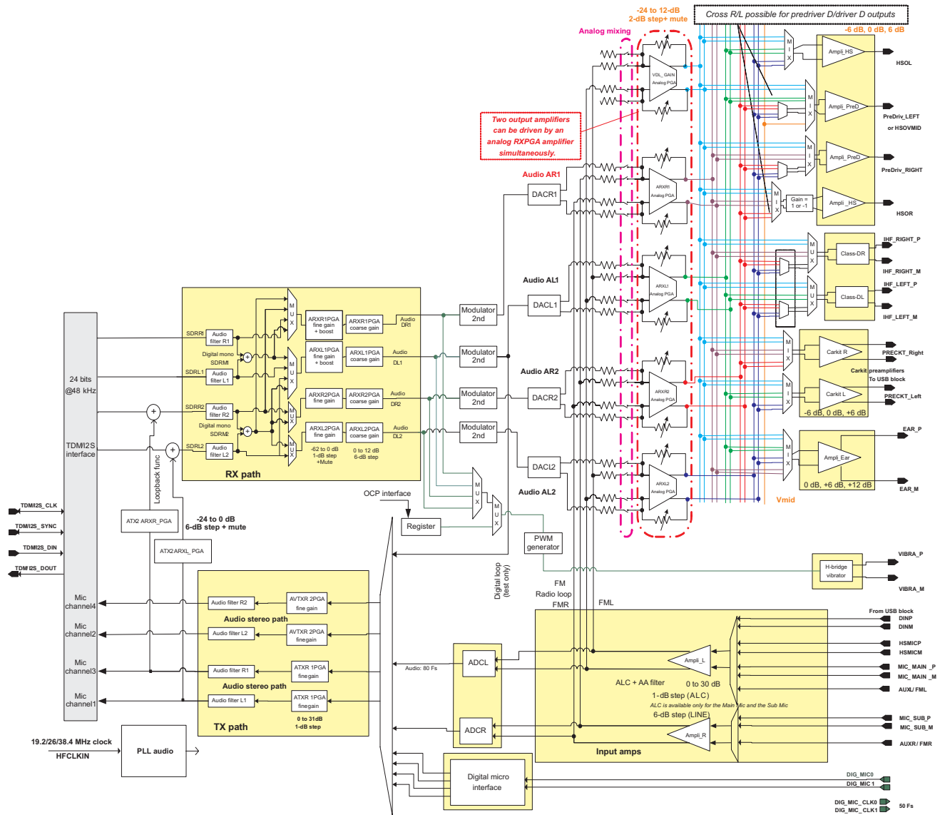
Figure 14-6. Voice/Audio Option 1 (OPT_MODE = 1) Block Diagram
