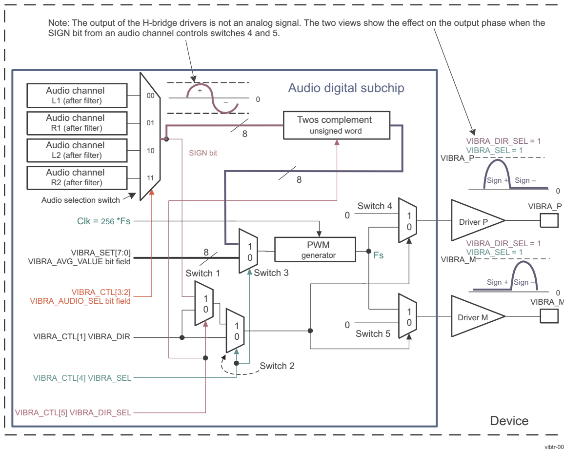
Figure 11-4. Functional Diagram of the Vibrator H-Bridge Driver
