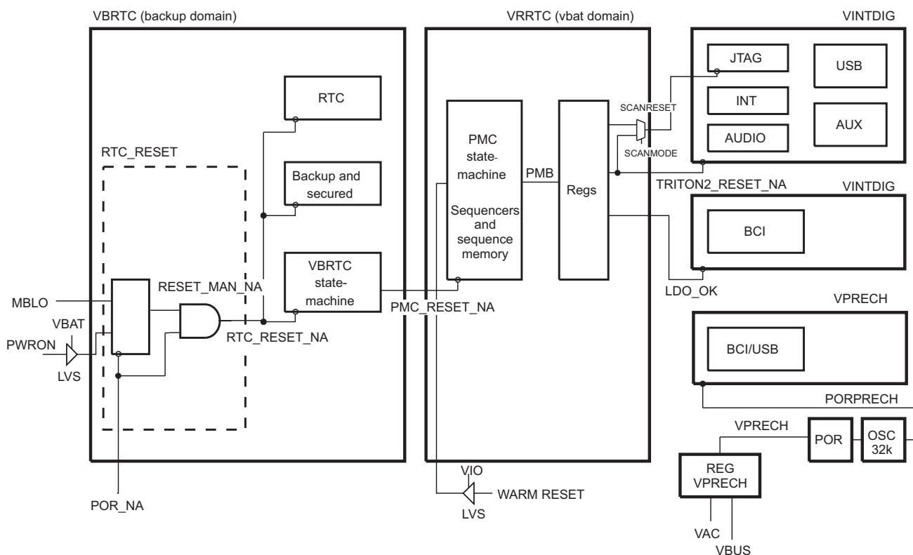
Figure 5-5. Device Reset Tree
