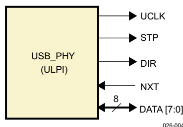
Figure 15-4. ULPI Signals
