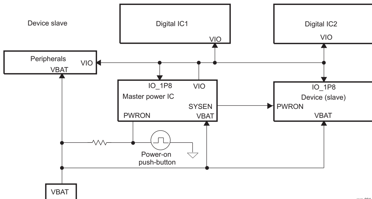
Figure 5-4. Slave Mode Integration
