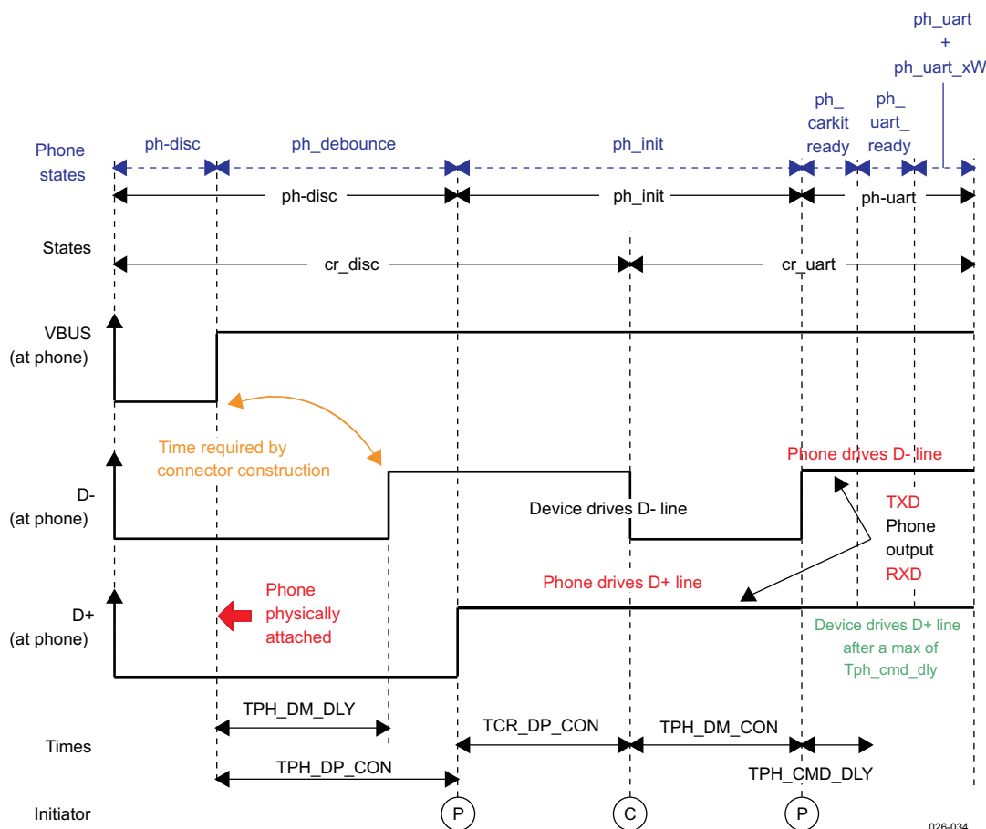
Figure 15-35. CEA Timing Diagram and PSM States Carkit Connection Sequence
