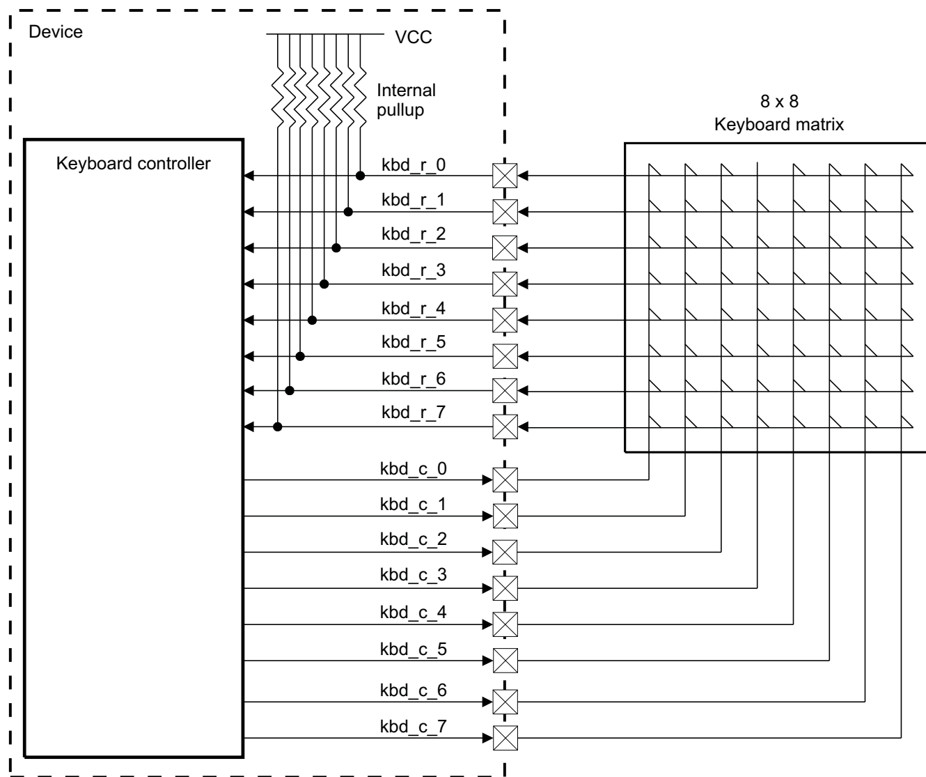
Figure 10-2. Device Keypad Controller Environment
