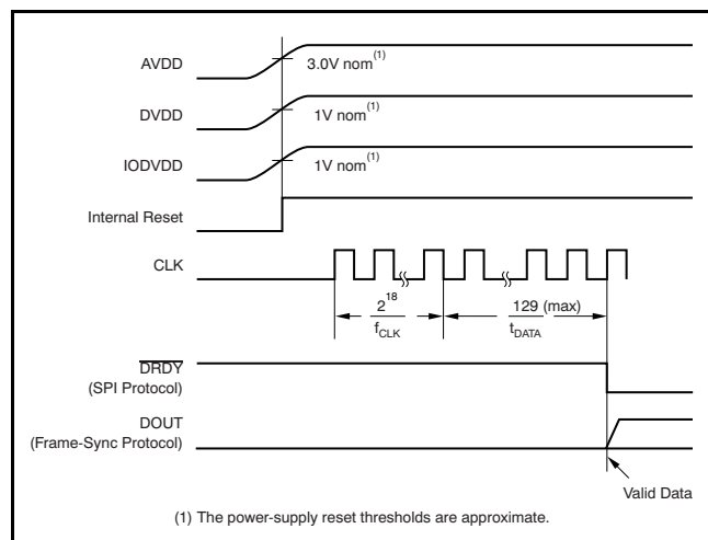
Figure 84. Power-Up Sequence
