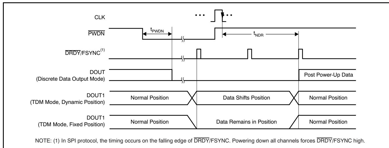
Figure 75. Power-Down Timing
