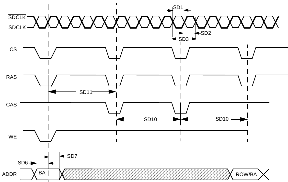
Figure 36. SDRAM Refresh Timing Diagram
