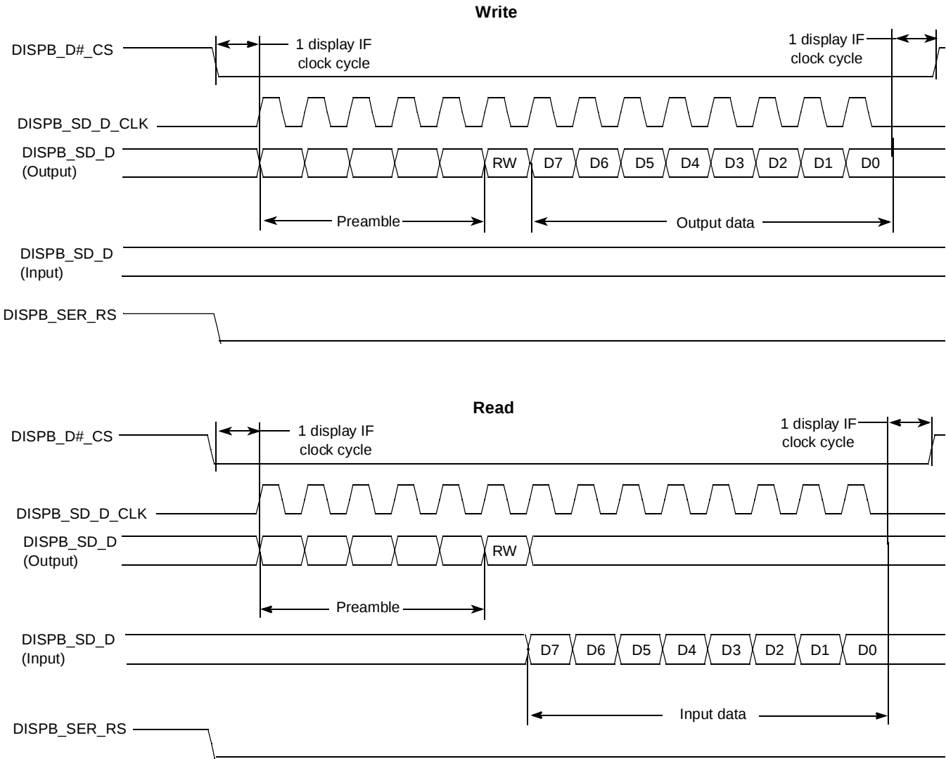
Figure 63. 5-Wire Serial Interface (Type 1) Timing Diagram
