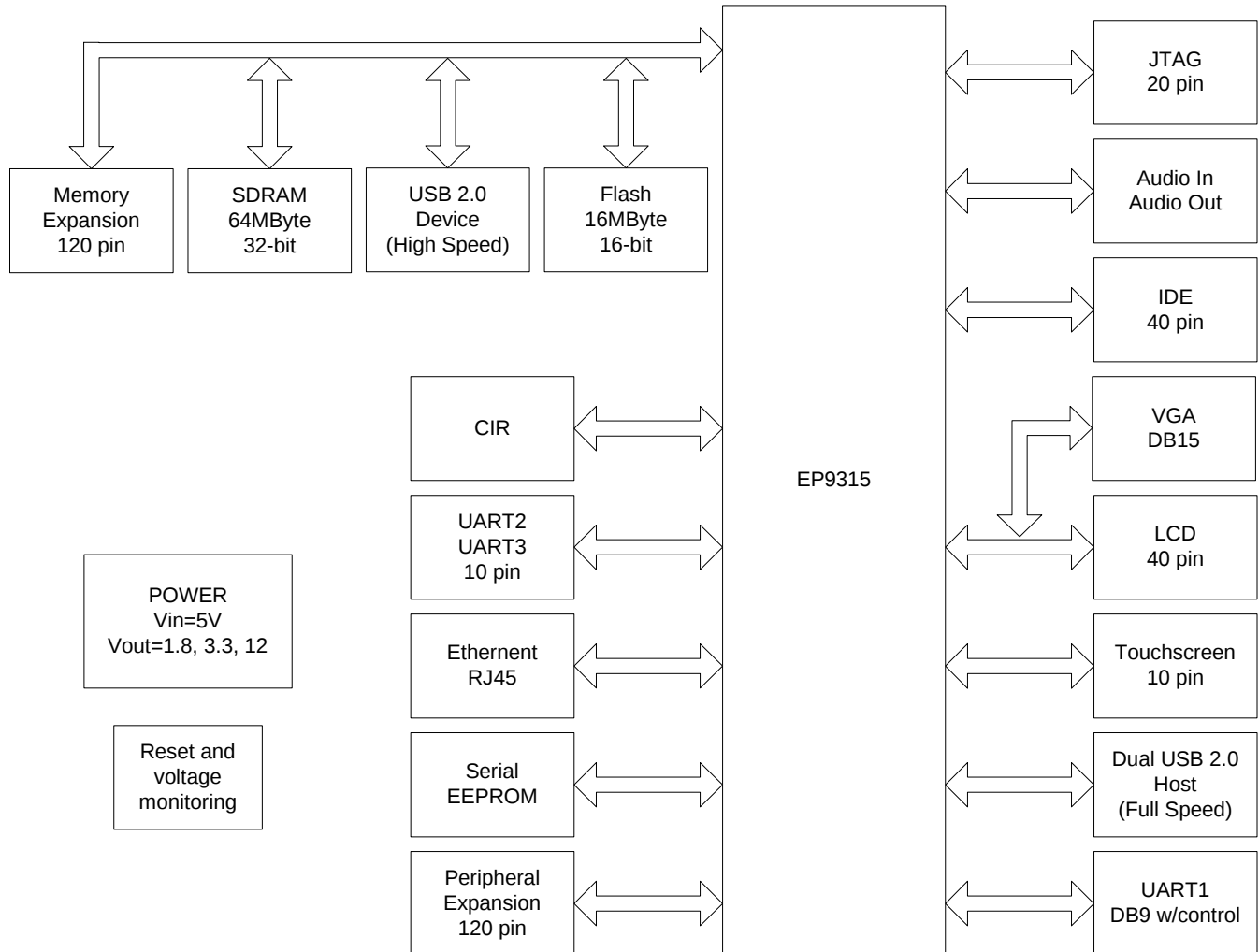
Figure 3. Block Diagram
