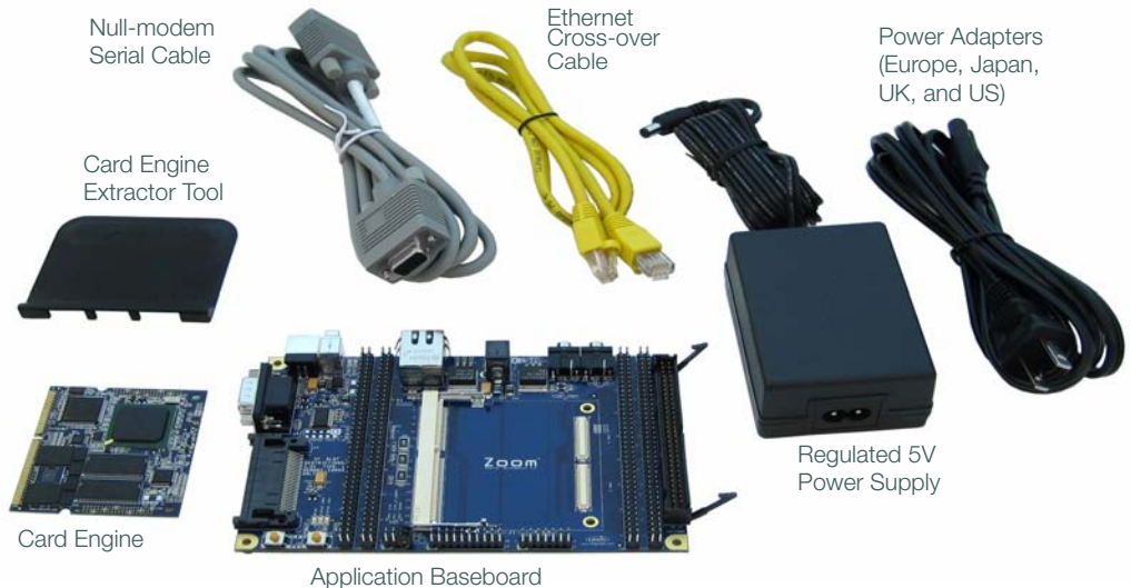
Figure 2.1 – Kit Contents
