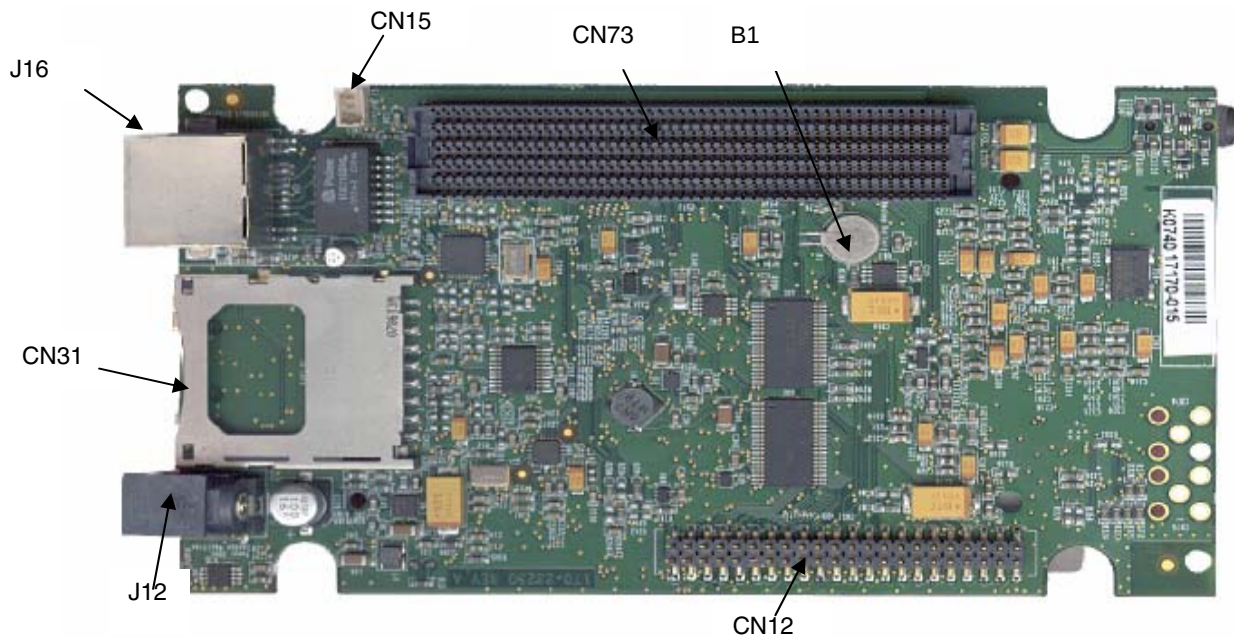
Fig 2-4 Personality Board, Bottom View
