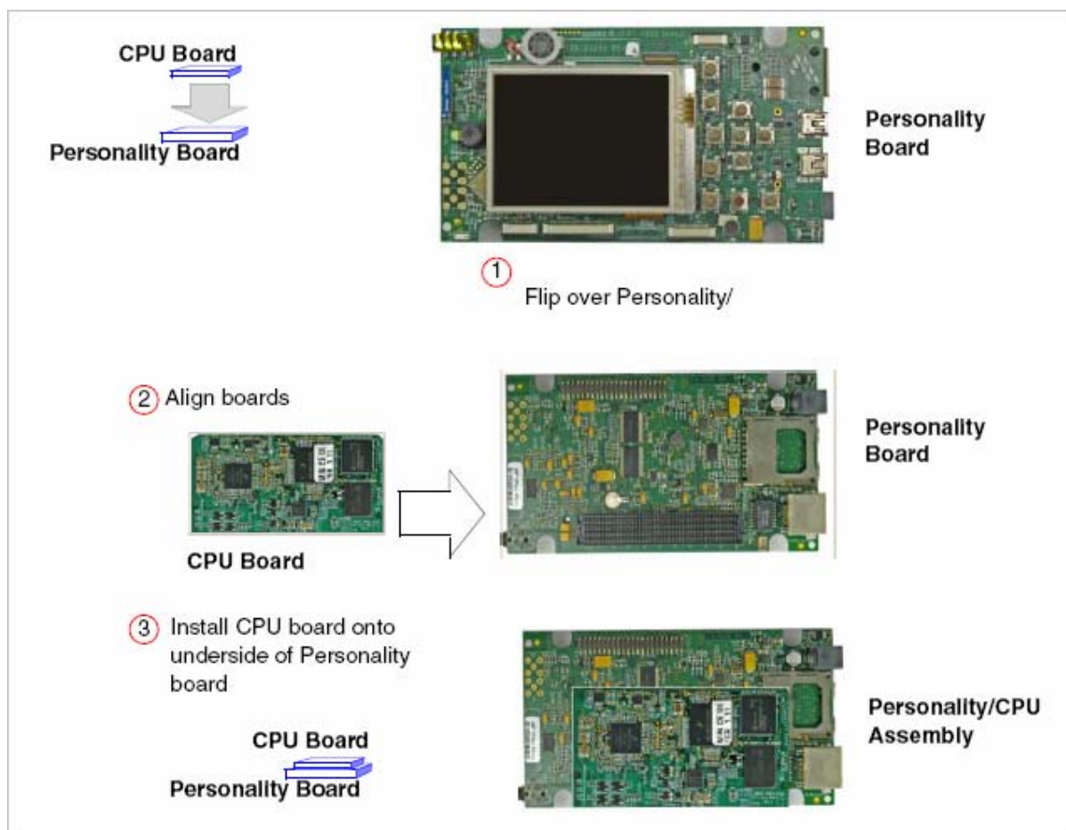
Figure 3-5 Install CPU Board onto Personality Board
