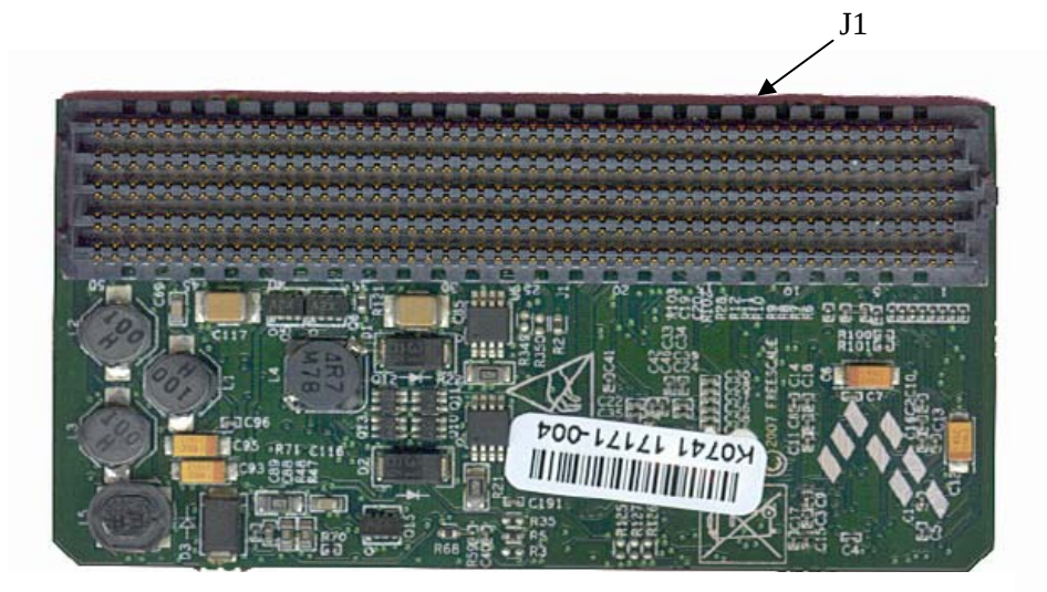
Figure 2-5 CPU Engine Board, Bottom View
