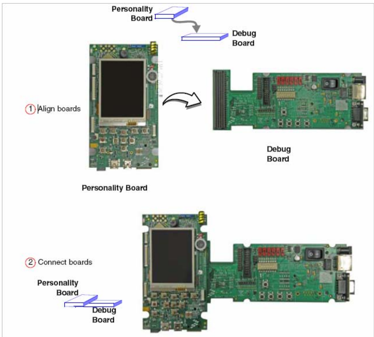
Figure 3-1 Install Personality Board onto Debug Board
