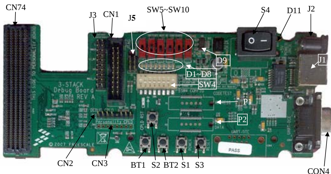
Figure 2-1 Debug Board, Top View
