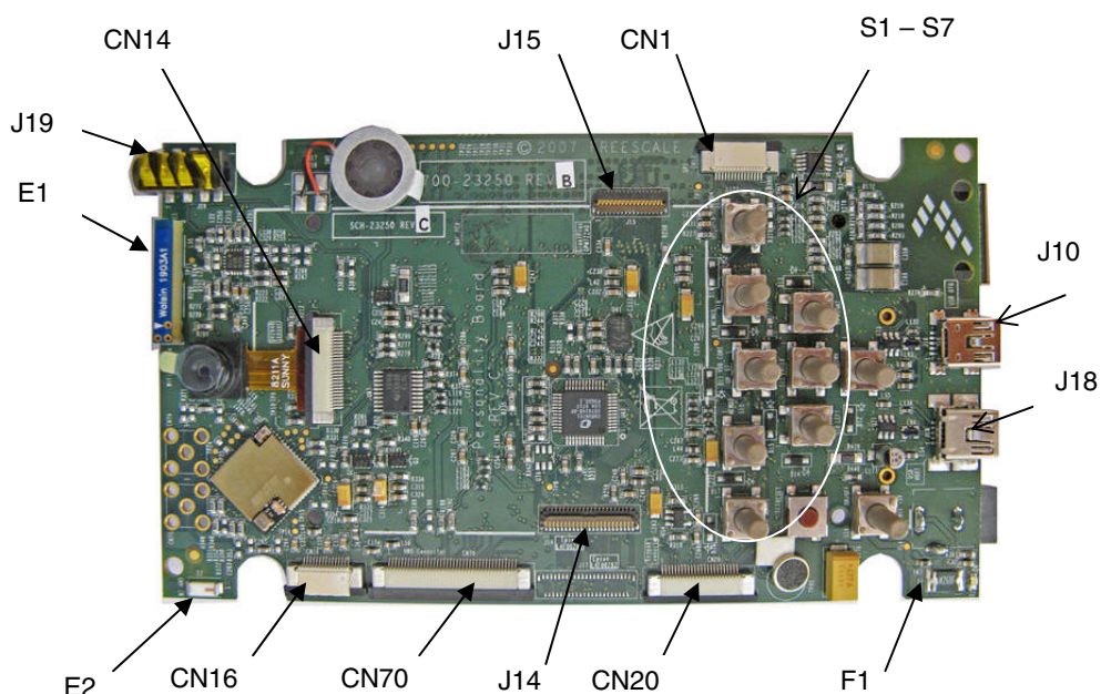
Figure 2-3 Personality Board Connectors, Top View
