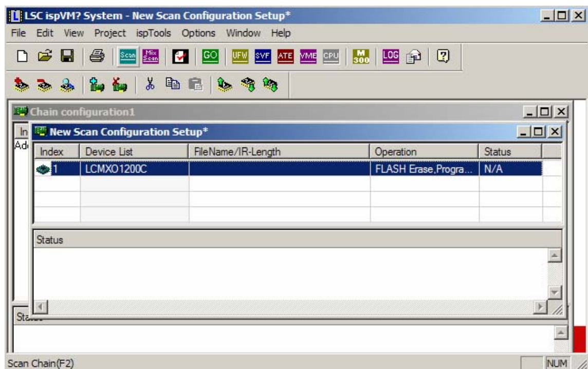
Figure 4-4 Scan CPLD Devices
