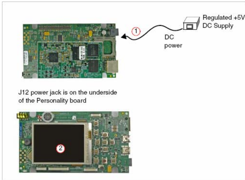
Figure 3-6 Connect Personality Board to Power Supply
