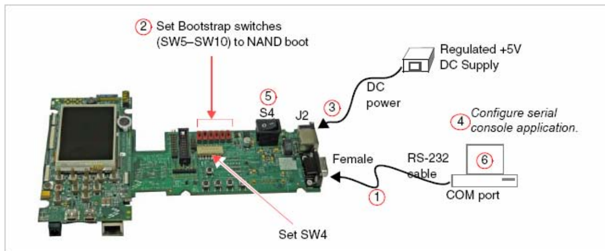
Figure 3-4 Connecting the Platform to Your PC
