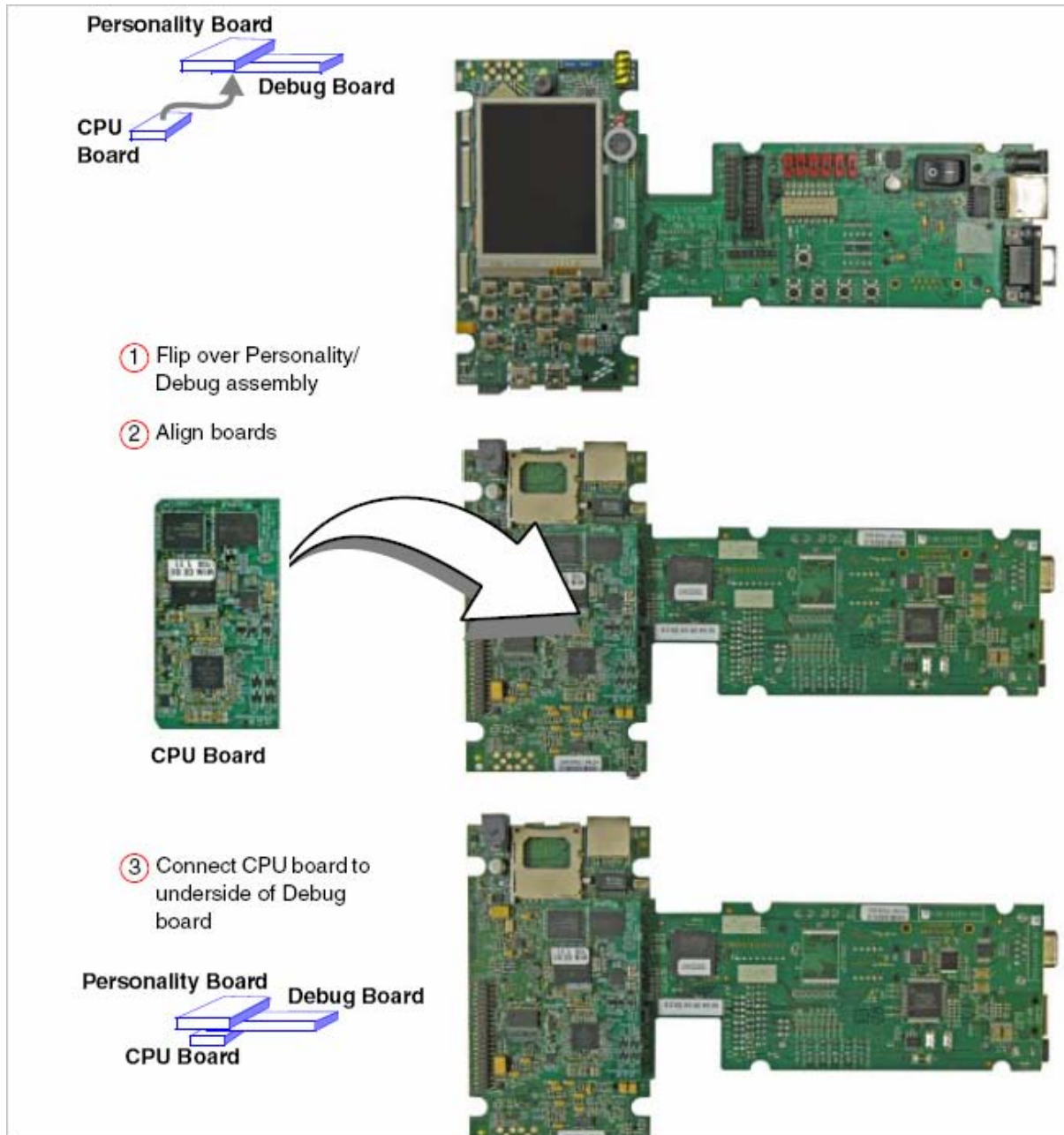
Figure 3-3 Align CPU Board and Debug/Personality Board
