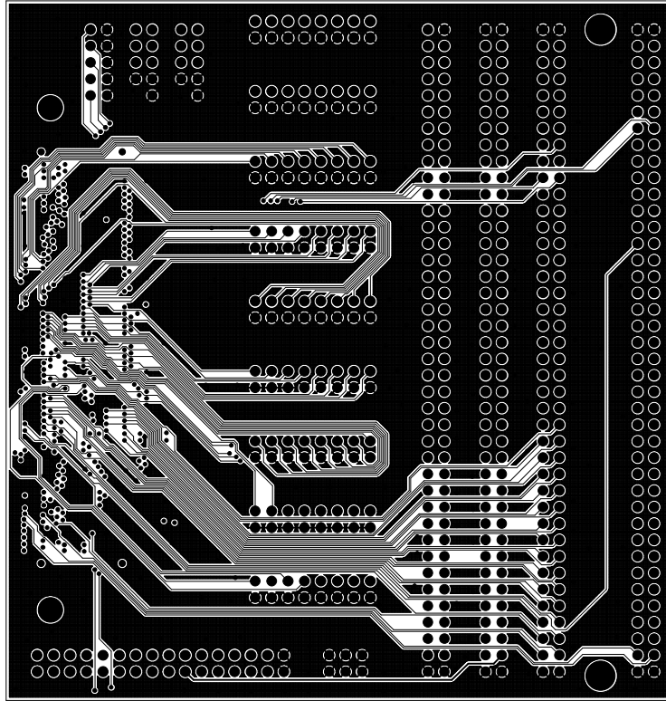
LAYER 2 INNER SIGNAL
