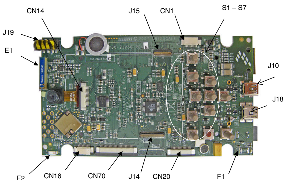
Figure 2-3 Personality Board Connectors, Top View
