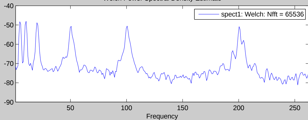
Welch Power Spectral Density Estimate
