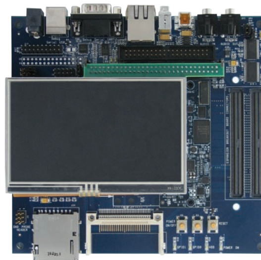
ZOOM OMAP35x DEVELOPMENT KIT WITH OMAP 3 SOM-LV & 4.3" WQVGA LCD INCLUDED
