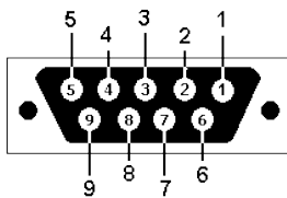
DB-9 Female
