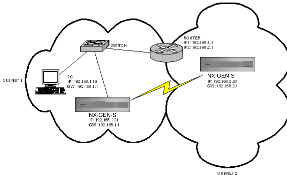
Figure 2-26. NX-GEN-S Units on Different Subnets
