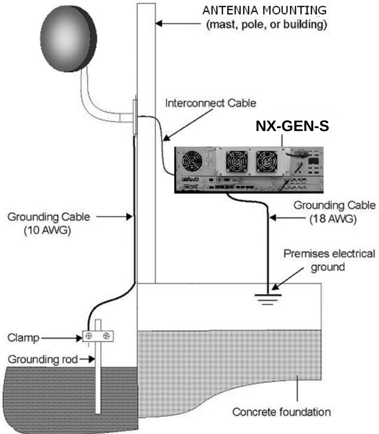
Figure 4-5. Ground Connection
