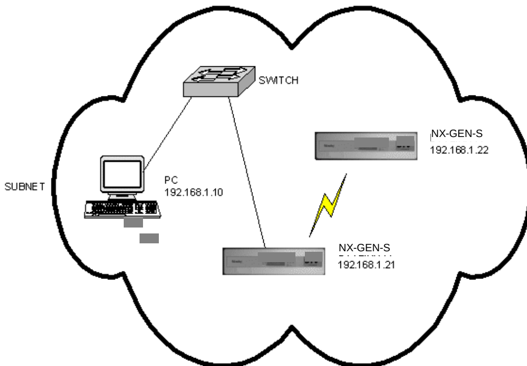
Figure 2-25. PC/NX-GEN-S on Same Subnet
