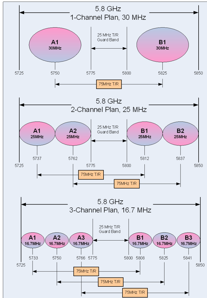
Figure 3-1. 5.8 GHz Channel Plan
