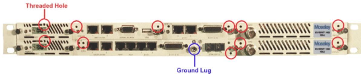
Figure 6-3. Threaded Hole Locations
