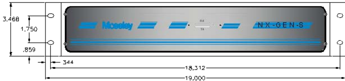
Figure 4-2. NX-GEN-S "ODU" Mounting Dimensions
