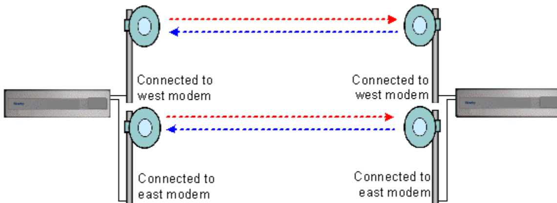
Figure 2-13. 1+1 Diversity Mode Protection
