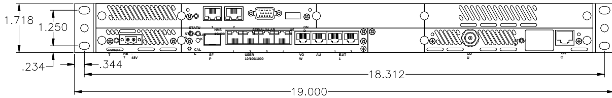
Figure 4-3. NX-GEN-S "SDIDU" Mounting Dimensions
