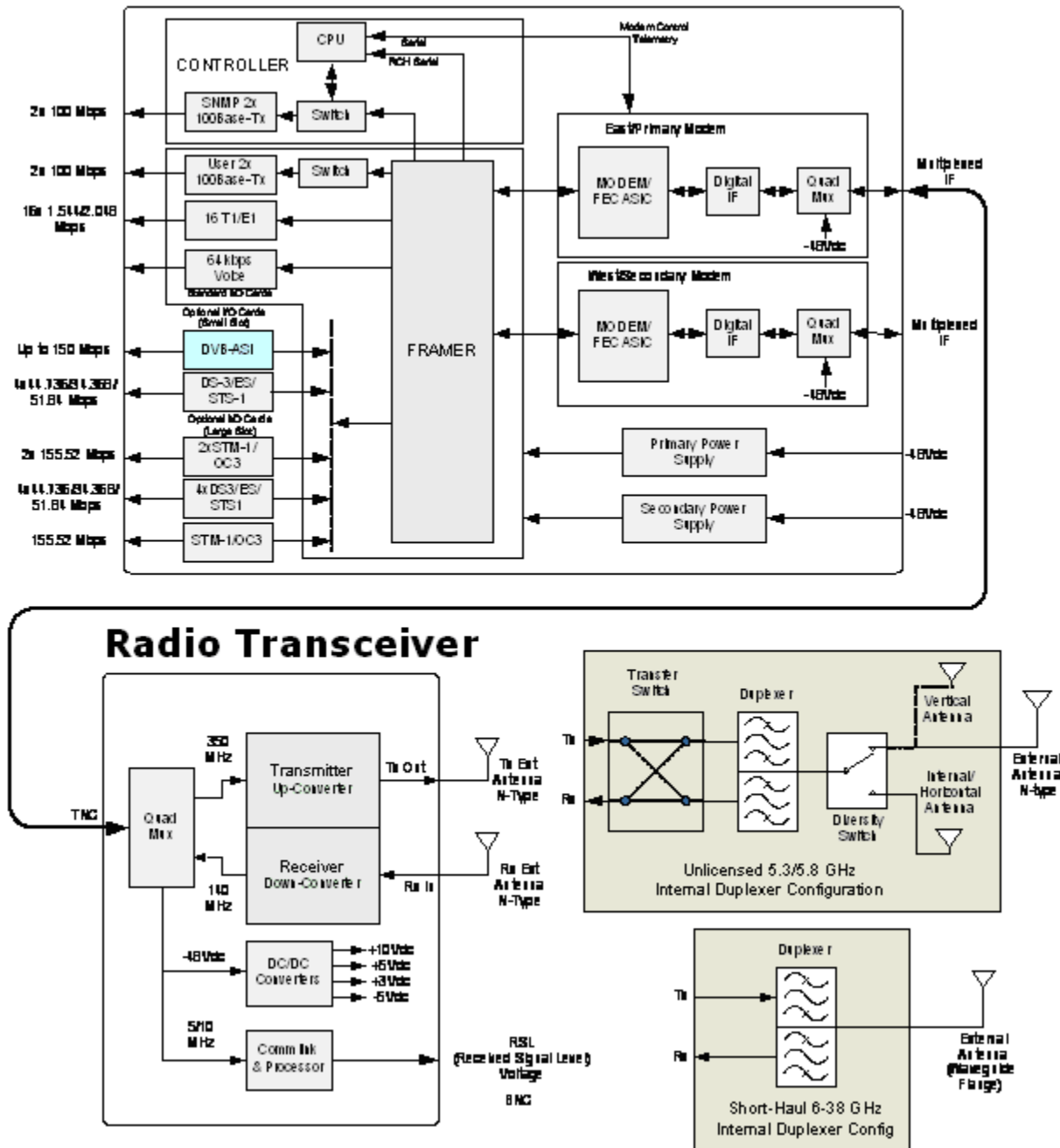
Figure 2-9. NX-GEN-S Block Diagram
