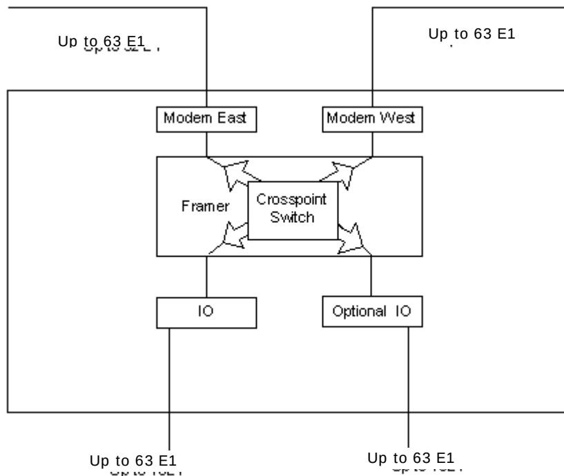
Figure 2-22. Crosspoint Switch
