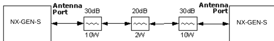
Figure 4-1. Back-to-Back Testing Configuration
