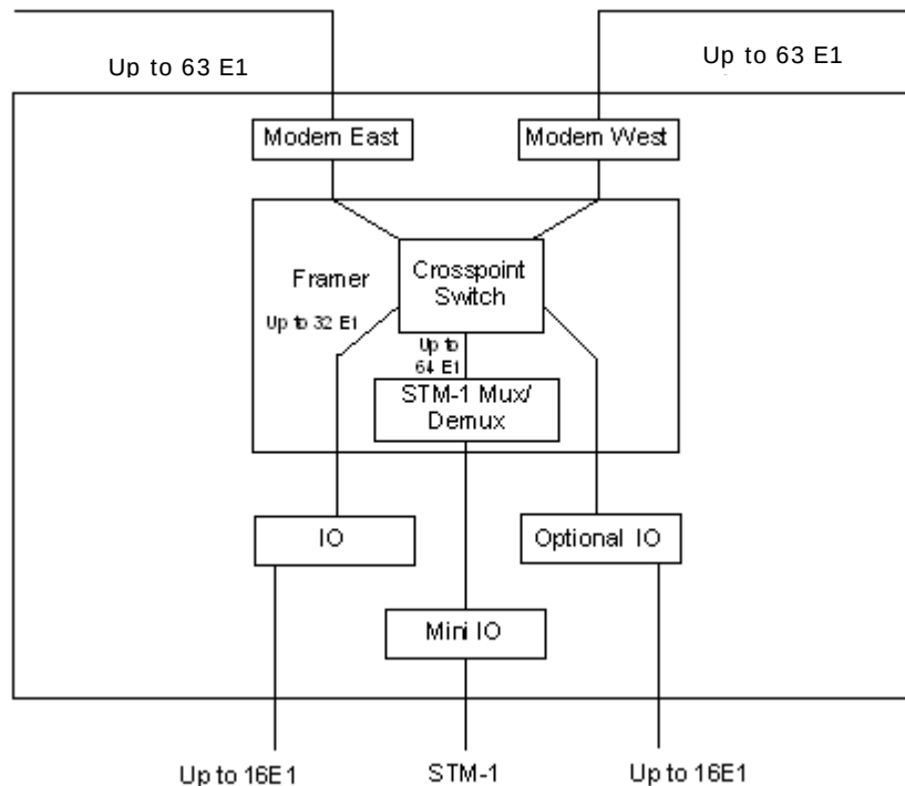
Figure 2-24. STM-1 Mux/Demux
