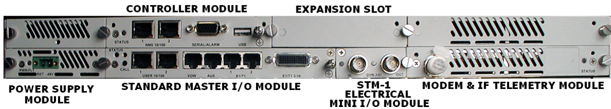
Figure 2-5. NX-GEN-S Modules
