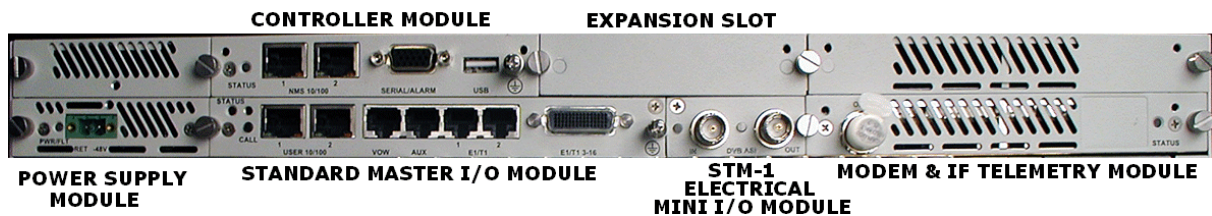
Figure 6-1. NX-GEN-S Modules
