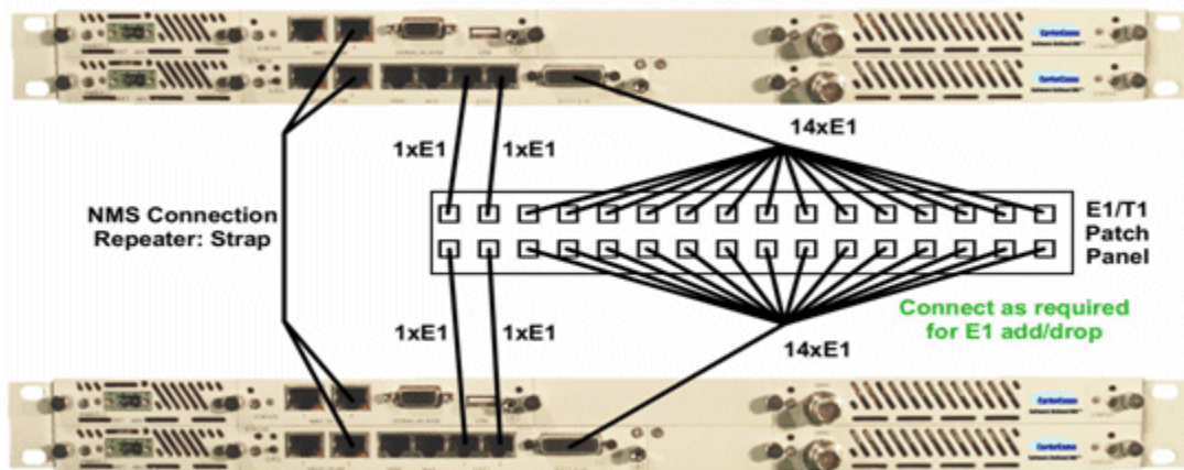
Figure 2-16. Back Panel Connections for E1/T1 Drop/Insert Capability
