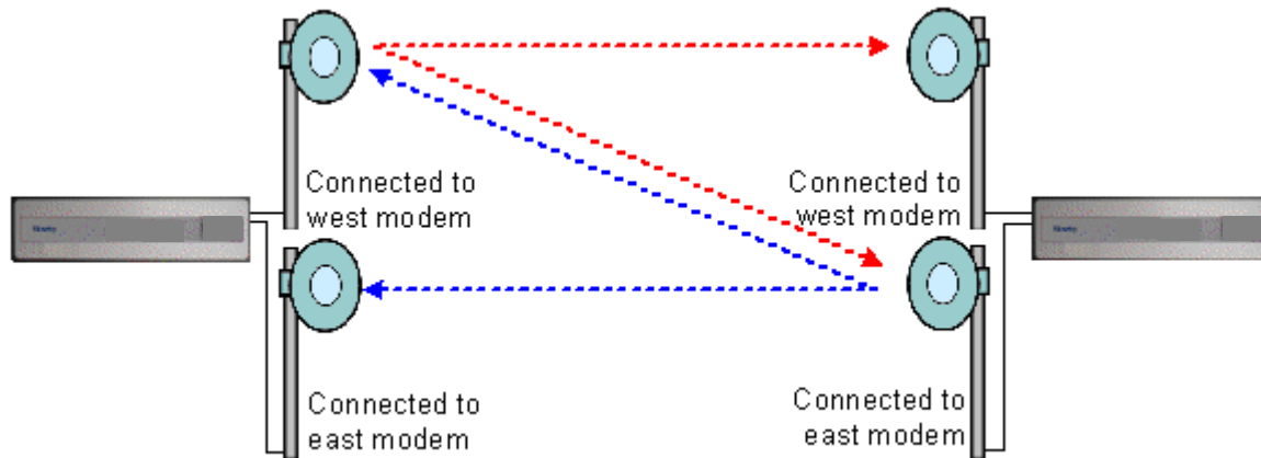
Figure 2-12. 1+1 Non-Diversity Mode Protection
