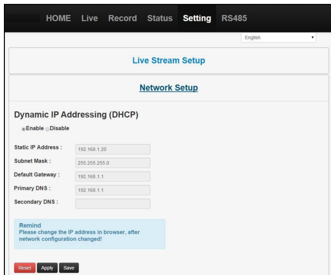
Network Setup
