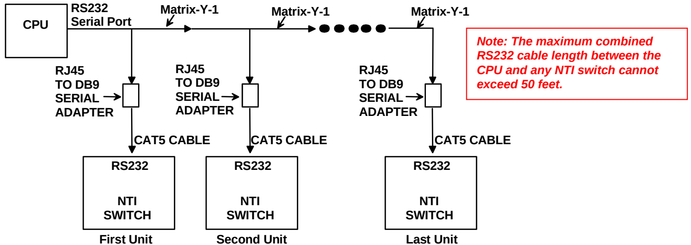
Figure 33- RS232 connection with Matrix-Y-1 cable
