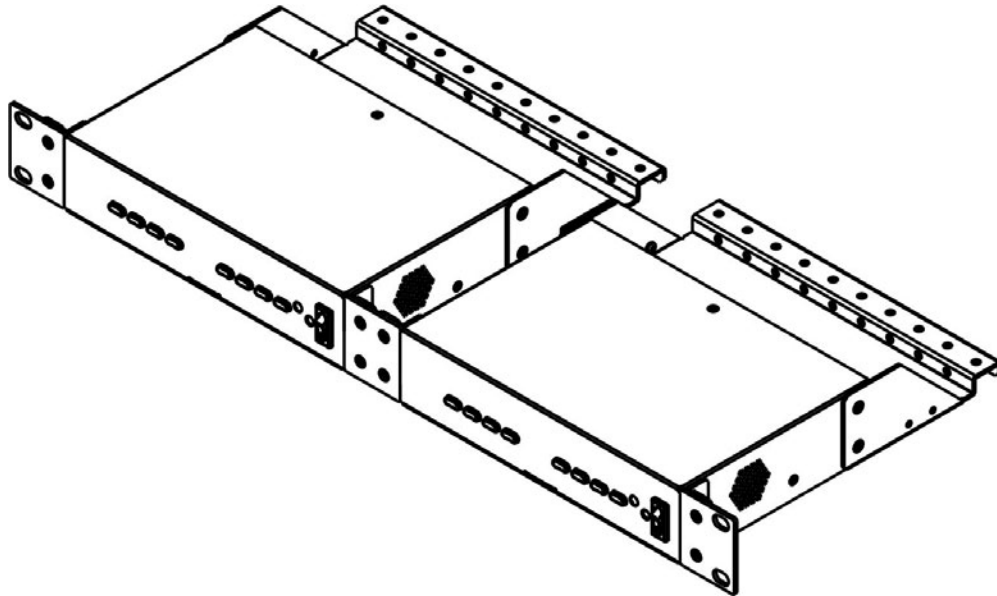
Figure 8- Assembled SPLITMUX-HD-4RT-2R
