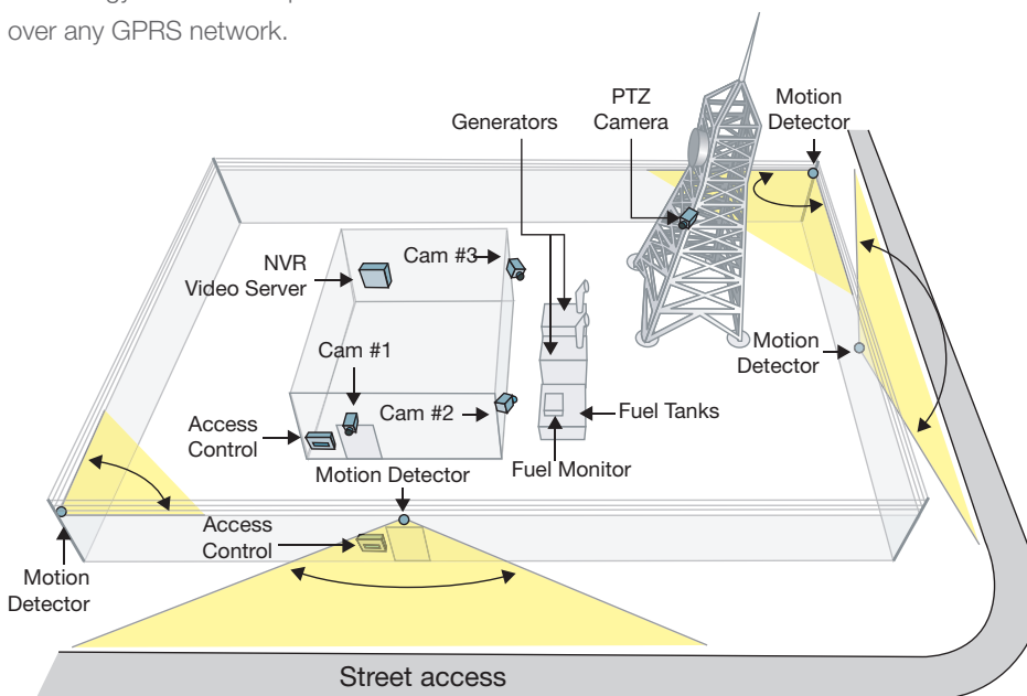
SecureSite integrated into a typical cell site.
