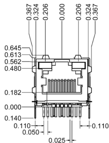
Figure 1 Front View
