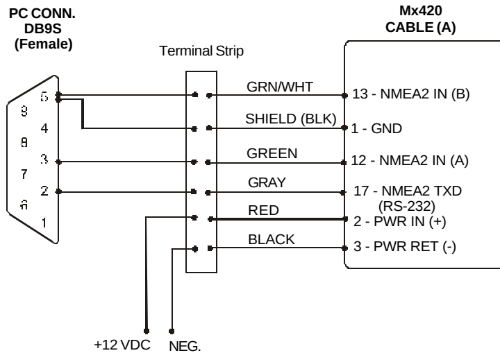
PC Interface Cable Diagram
