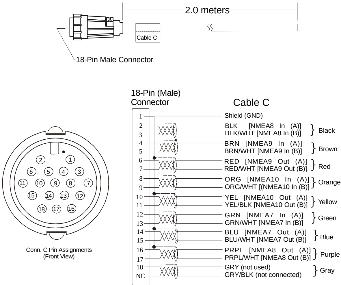
Figure 4.11 Cable (C) Wiring Configuration (Only on MX420/8)
