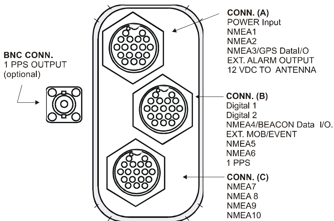
Figure 4.13 MX420/8 Rear Panel Connectors
