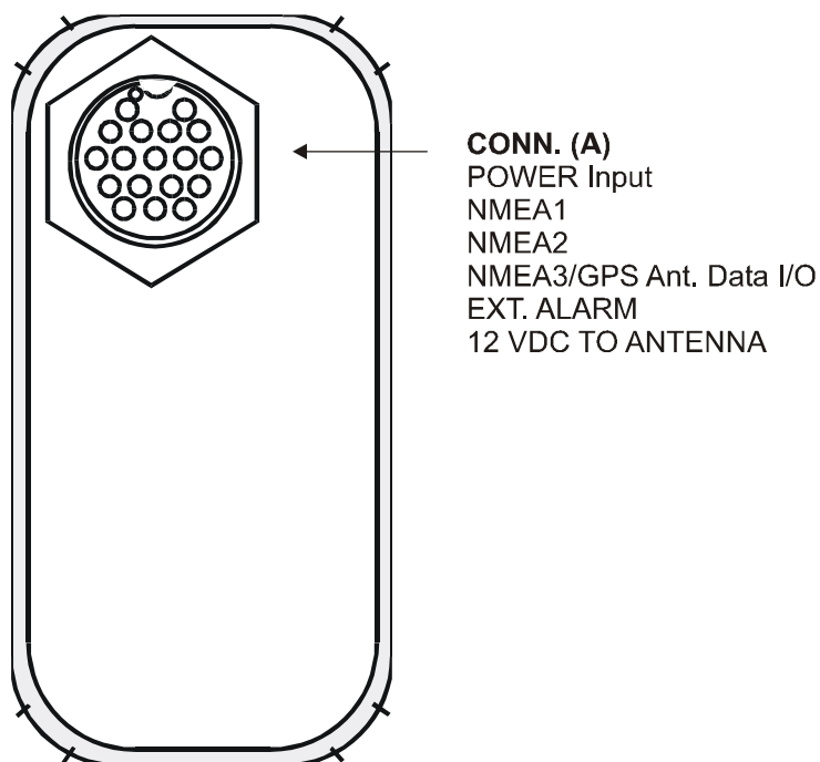
Figure 4.12 MX420/2 Rear Panel Connector
