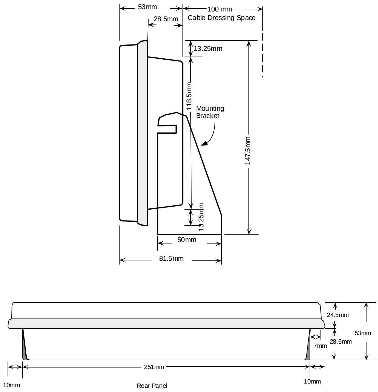
Figure 3.2 MX420 Display Console Dimensions (Top and Side View)
