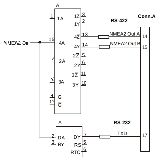
Figure 5.1 Port 2: RS- 422 / RS- 232 Port Schematic
