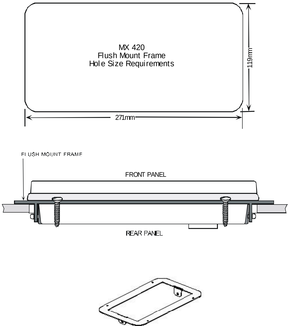
Figure 3.5 Optional Flush Mount Frame Installation
