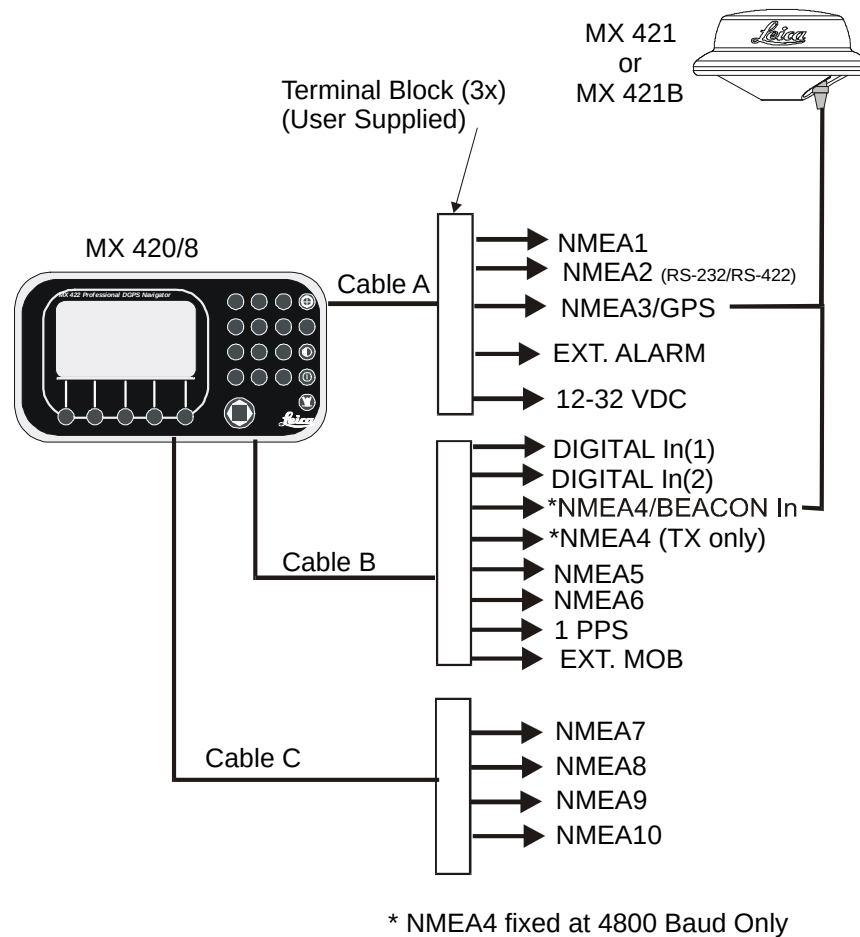
Figure 4.3 MX420/8 System Configuration
