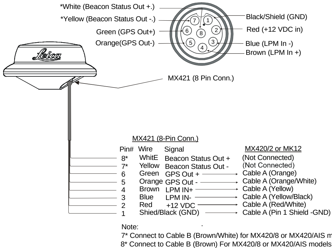
Figure 4.14 MX421(8-Pin) GPS Antenna Wiring Diagram
