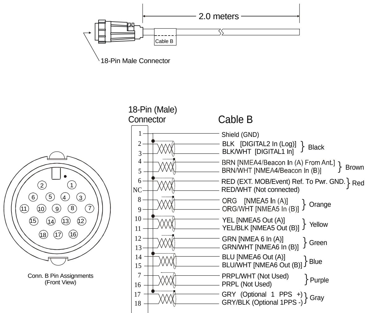
Figure 4.10 Cable (B) Wiring Configuration (Only on MX420/8)
