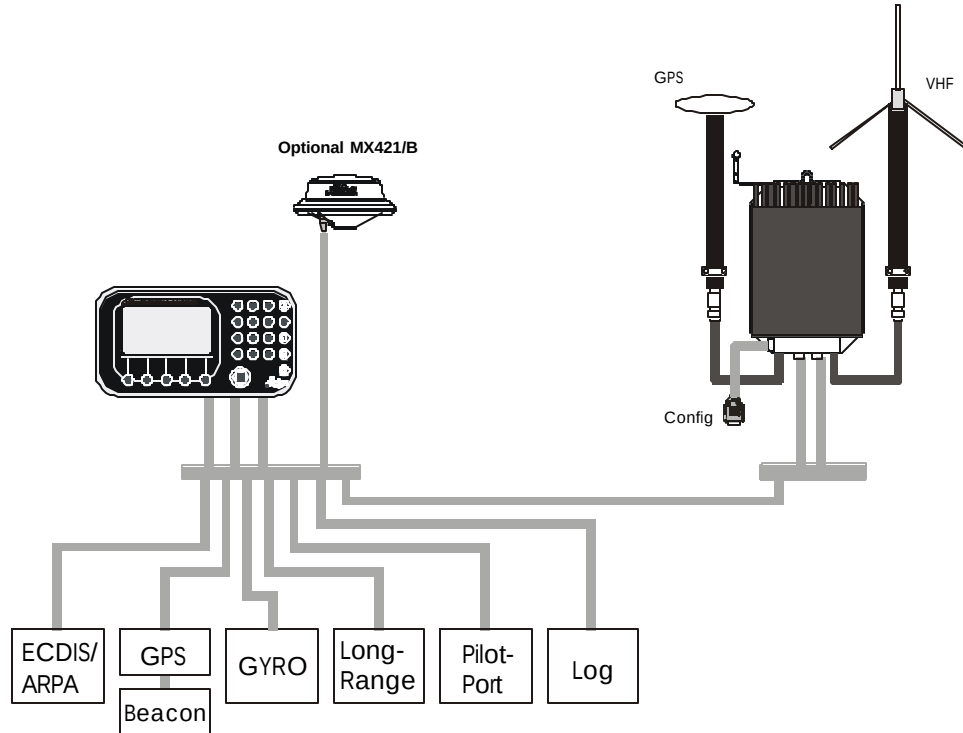
MX420 AIS Basic configuration
