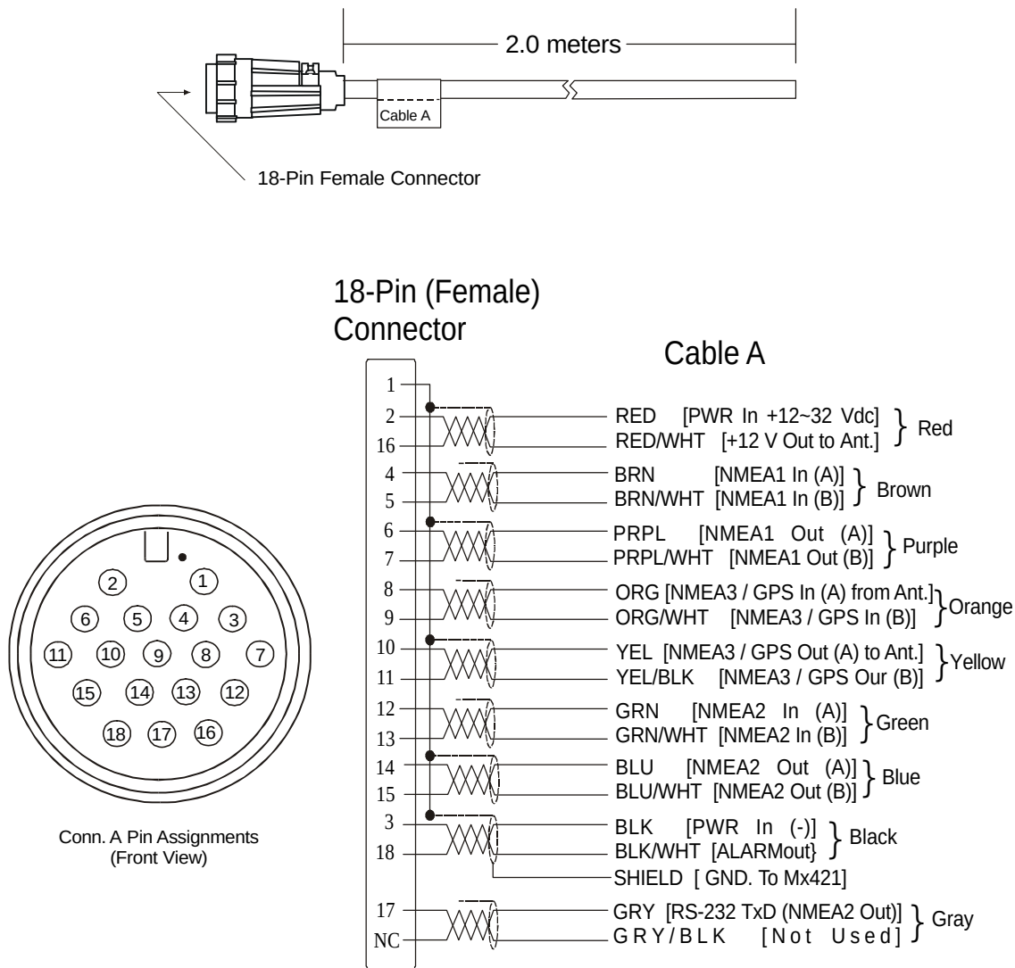
Figure 4.9 Cable (A) Wiring Configuration
