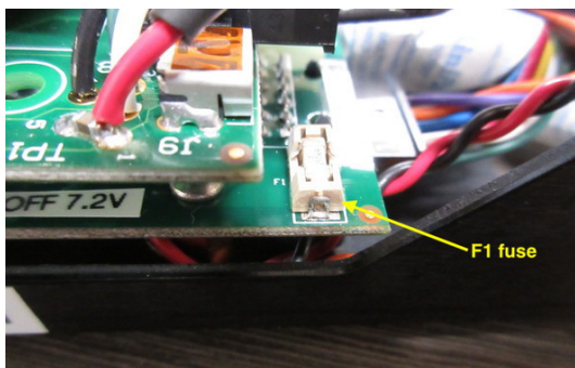
Figure 41: 0.25 A Fuse (for CR123 battery)
