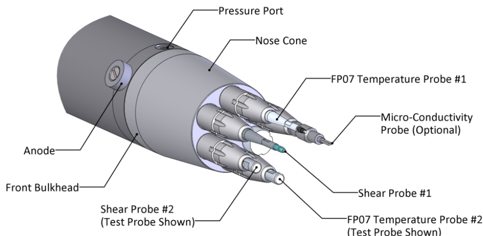
Figure 3: MicroRider-1000 Sensors
