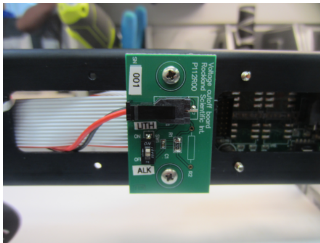
Figure 43: Voltage cutoff board installed in the MicroRider-1000-WireWalker. The switch is set for the Lithium-Ion Battery shutdown voltage of 12.4 V.
