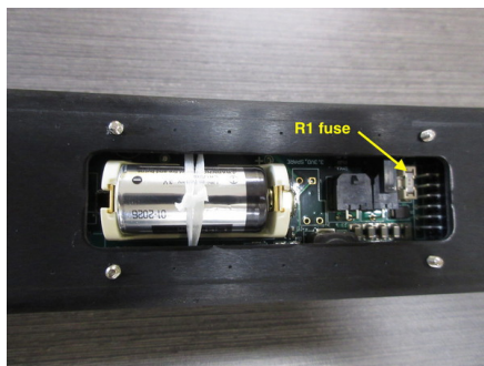
Figure 40: CR123 battery and 1 A fuse (Power Input)
