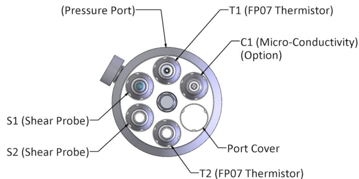
Figure 15: Nose cone sensor layout
