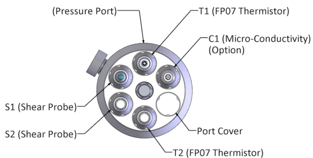
Figure 25: Nose cone sensor layout.
