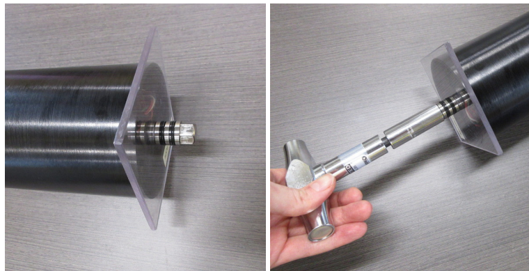
Figure 28: Sliding electronics into the pressure tube using the plastic plate.
