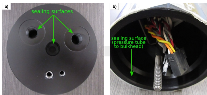
Figure 34: Typical sealing surfaces for a (a) rear bulkhead, and (b) pressure tube. (Note: A MicroCTD bulkhead and tube are pictured.)
