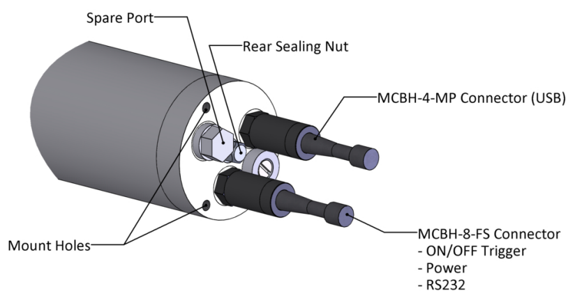
Figure 6: Rear Bulkhead
