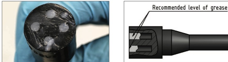
Figure 37: Applying grease to a MCBH connector. (Image source: SubConn and McCartney Underwater Connector Group (2018). Underwater and Harsh Environment Connectors . p. 122. 16 )
