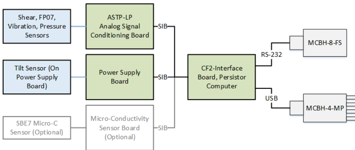
Figure 7: Instrument sensor and electronics system block diagram
