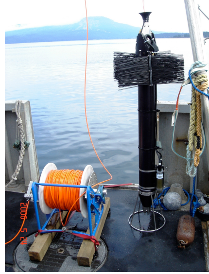
Figure 2: The VMP-500 Profiler and a small hand-winch to manage its electro-mechanical tether.
