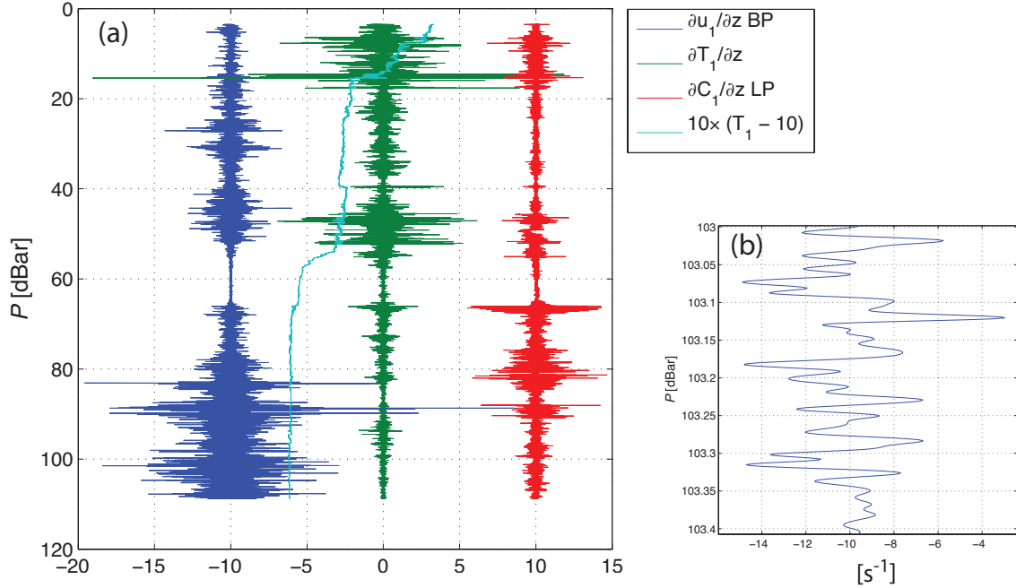
Figure 6: (a) Profiles of shear (blue) and the vertical gradients of temperature (green) and conductivity (red). The data are band-pass filtered between 0.4 and 50 Hz for display purposes only. A scaled version of the temperature profile (cyan) is shown for reference. The shear and the conductivity gradients have been shifted left and right by 10 units for clarity. (b) A 40 cm detail of the shear starting at 103 m depth highlights the centimetre-scale variations resolved by the shear probe.
