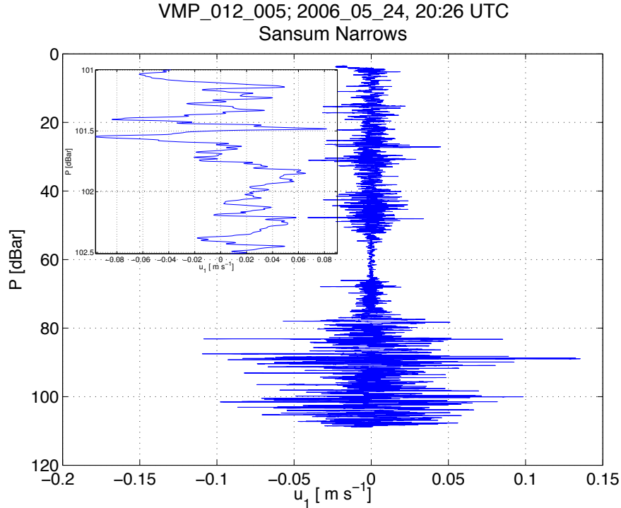
Figure 8: (a) Profiles of turbulent horizontal velocity computed by numerically integrating the vertical shear. (inset) A 1.50 m detail of the velocity starting at 101 m depth highlights the centimetre-scale variations resolved by the shear probe.
