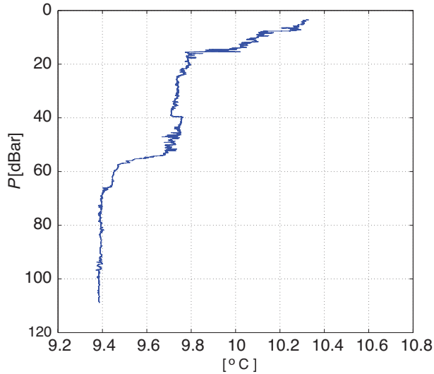
Figure 5: Temperature profile from Sansum Narrows collected with the high-resolution thermistor on the VMP-500.
