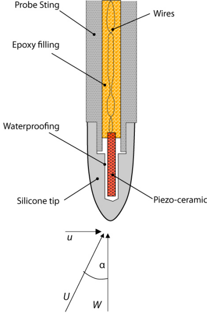
Figure 3: Shear probe schematic. W is the apparent vertical velocity due to profiling, u is the horizontal velocity fluctuation due to turbulence, U is the total velocity, and \alpha is the angle of attack.
