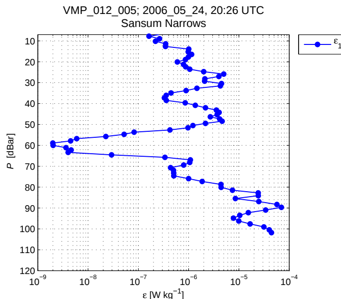
Figure 7: The vertical profile of the rate of dissipation of TKE. The estimates are spaced approximately 1.25 m vertically.
