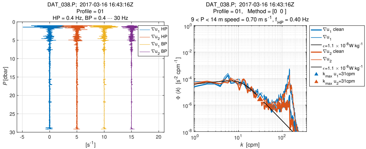
Figure 22: (Left) Data profiles with despiking applied to the same shear signals as in Figure 21. The spike near 10 dbar in Figure 21 has been eliminated. (Right) Shear spectra calculated between 9 and 14 dbar. The spectrum of sh1 is no longer anomalous with respect to the Nasmyth spectrum and the sh2 spectrum.
