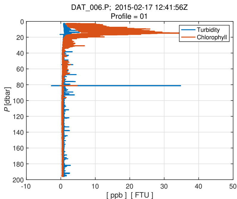
Figure 11: The vertical profile of backscatter in units of FTU (blue line) and chlorophyll in units of ppb (red line) measured with the JAC sensor.
