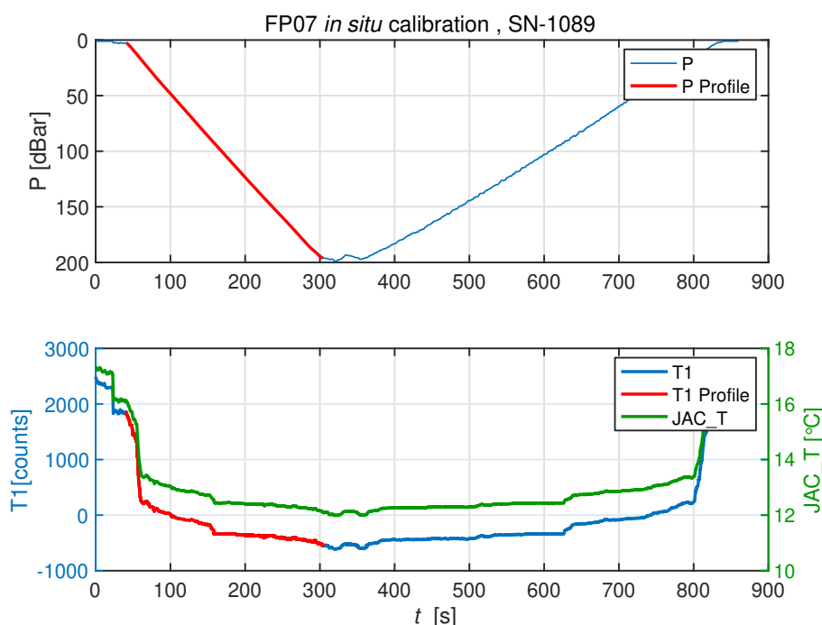
Figure 16: A profile is selected using the parameters described in the input structure cal.info . (Top panel) The pressure signal for the entire datafile is shown in blue and the segment corresponding to the selected profile is shown in red. (Bottom panel) The temperature signal in raw counts for the entire datafile is shown in blue and the segment corresponding to the selected profile is shown in red. The data from the reference thermometer in degrees Celcius is shown in green on the right axis.
