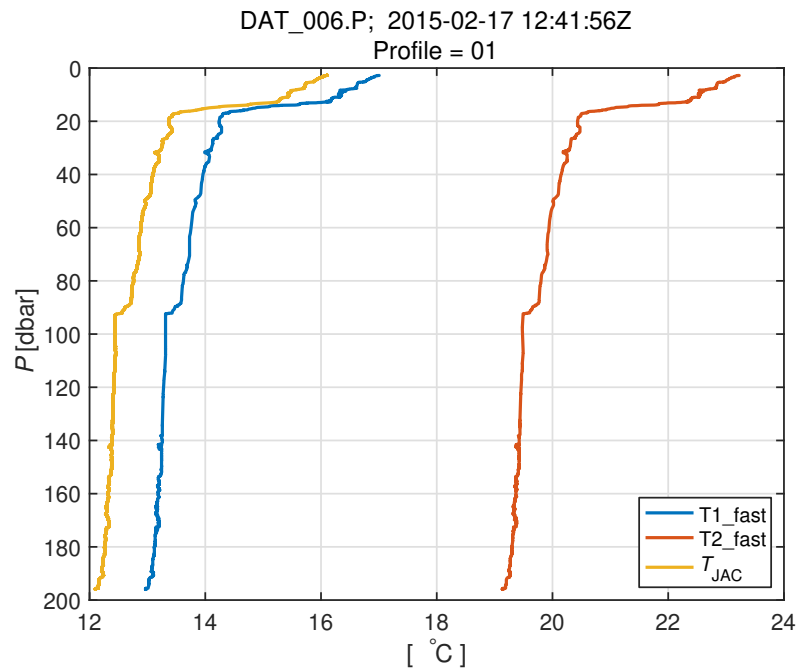
Figure 12: The vertical profiles of temperature from the two thermistors, T_1 (blue) and T_2 (red), and from the stable CT sensor ( T_{JAC} , gold). The thermistors have not been calibrated.
