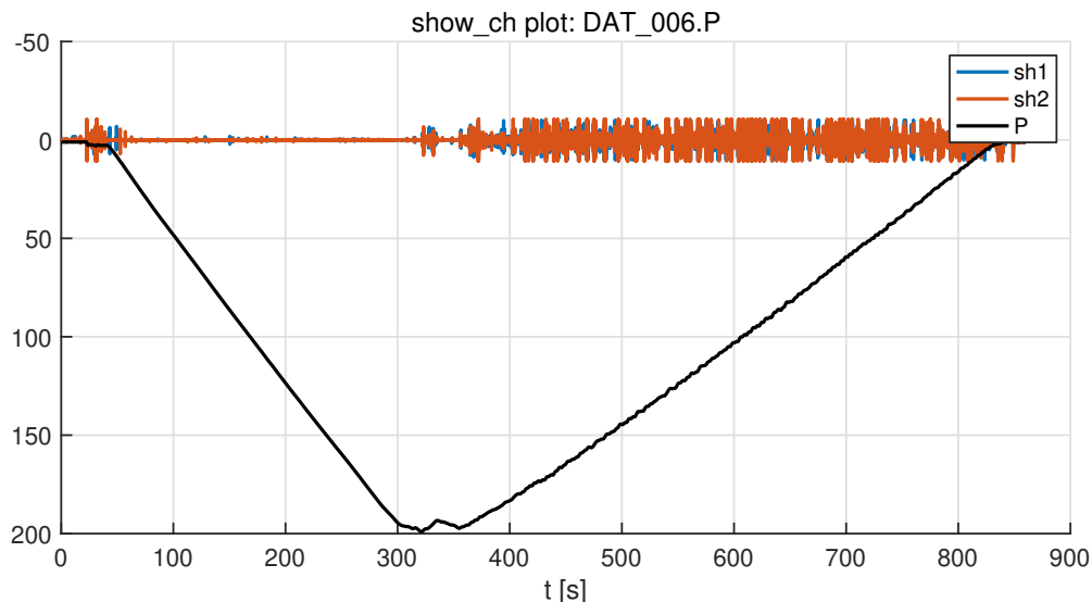
Figure 2: Time series of the pressure and shear signals generated using show_ch . The data are in physical units, i.e. P has units of dbar and sh1 and sh2 have units of s -1 .
