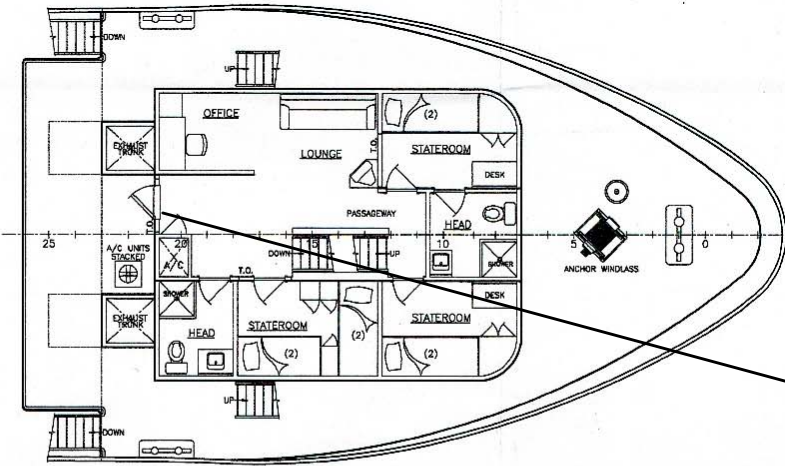
FOC'SLE DECK
