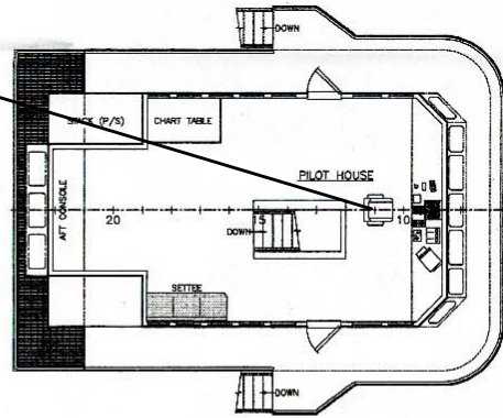
BRIDGE DECK
