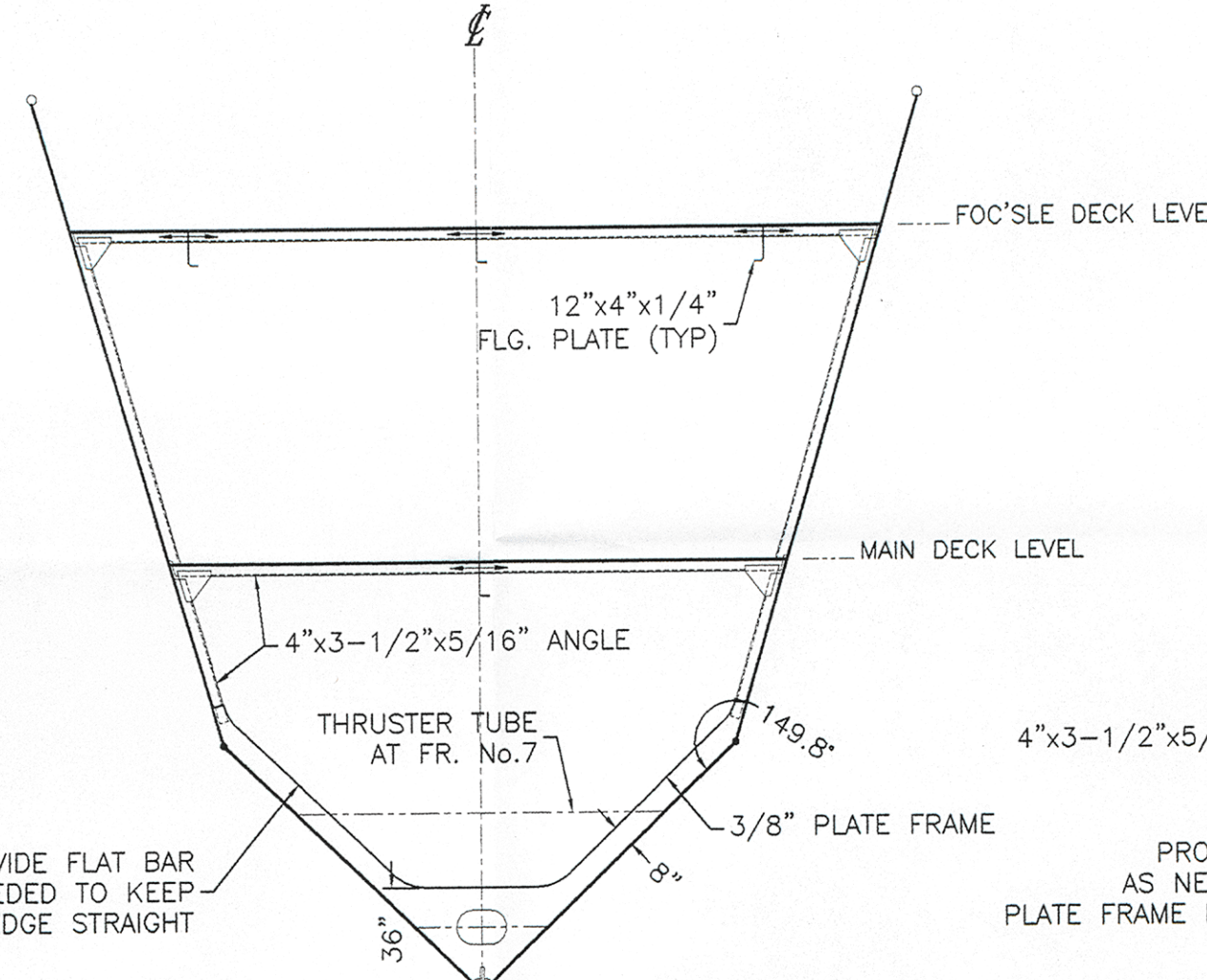
FRAME No.6 LOOKING AFT
