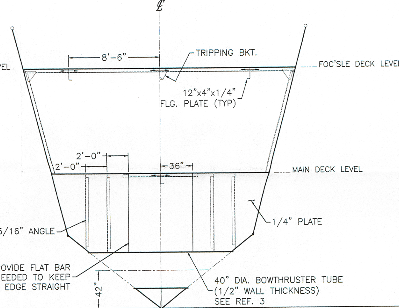
FRAME No.7 LOOKING AFT
