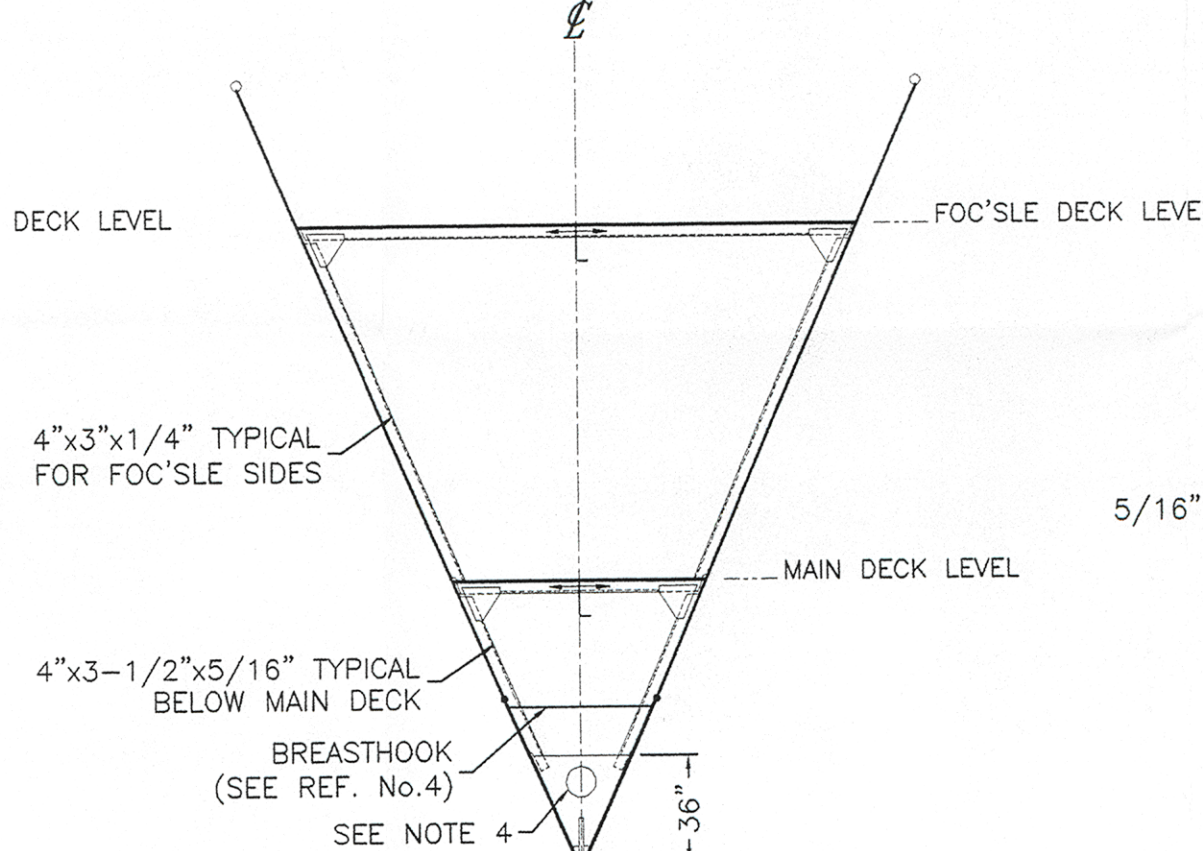
FRAME No.2 LOOKING AFT
