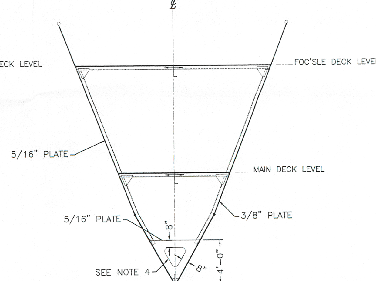
FRAME No.3 LOOKING AFT
