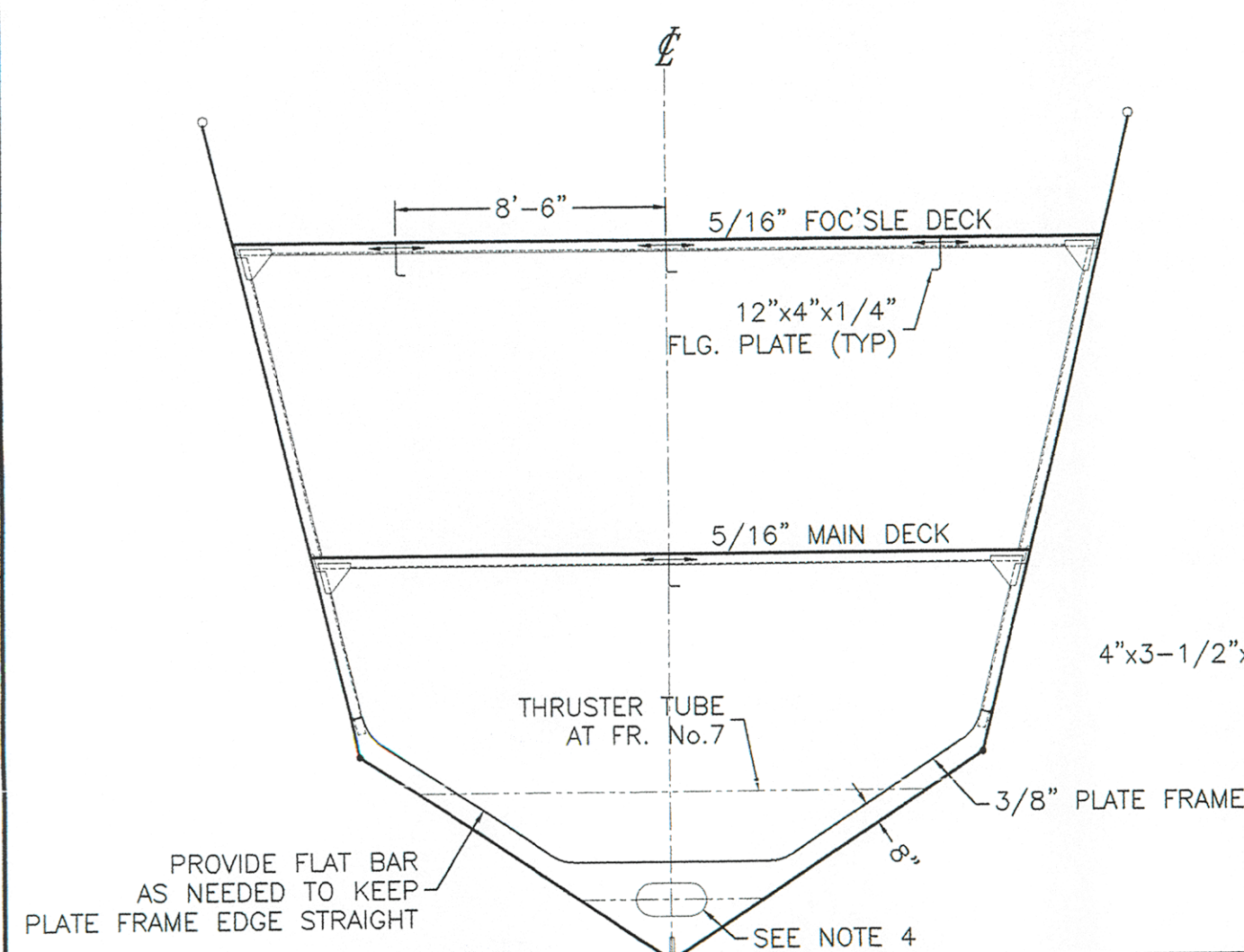
FRAME No.8 LOOKING AFT
