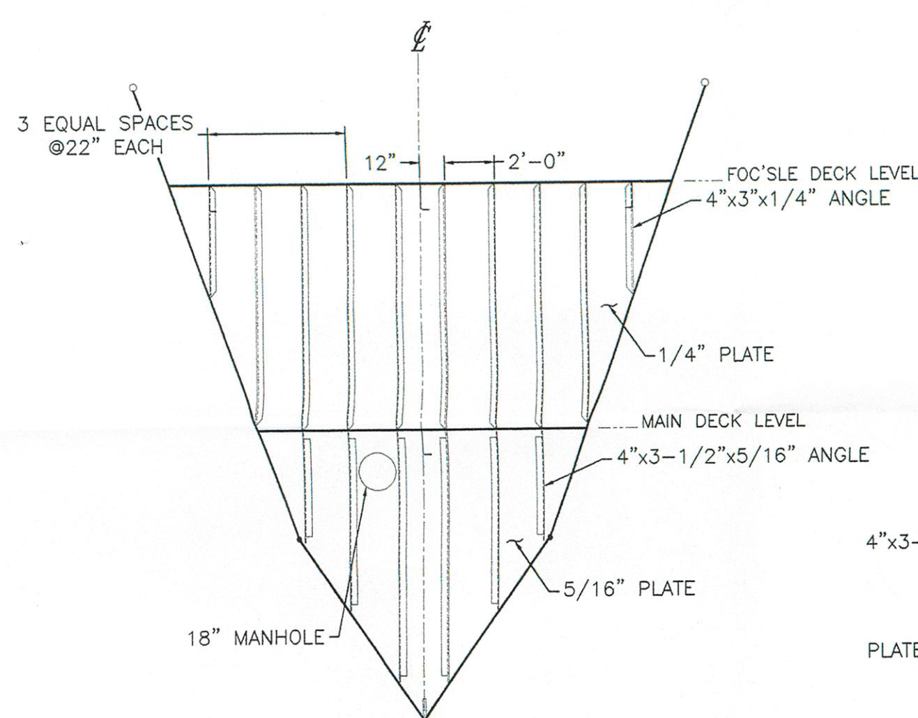
FRAME No.4 LOOKING AFT
