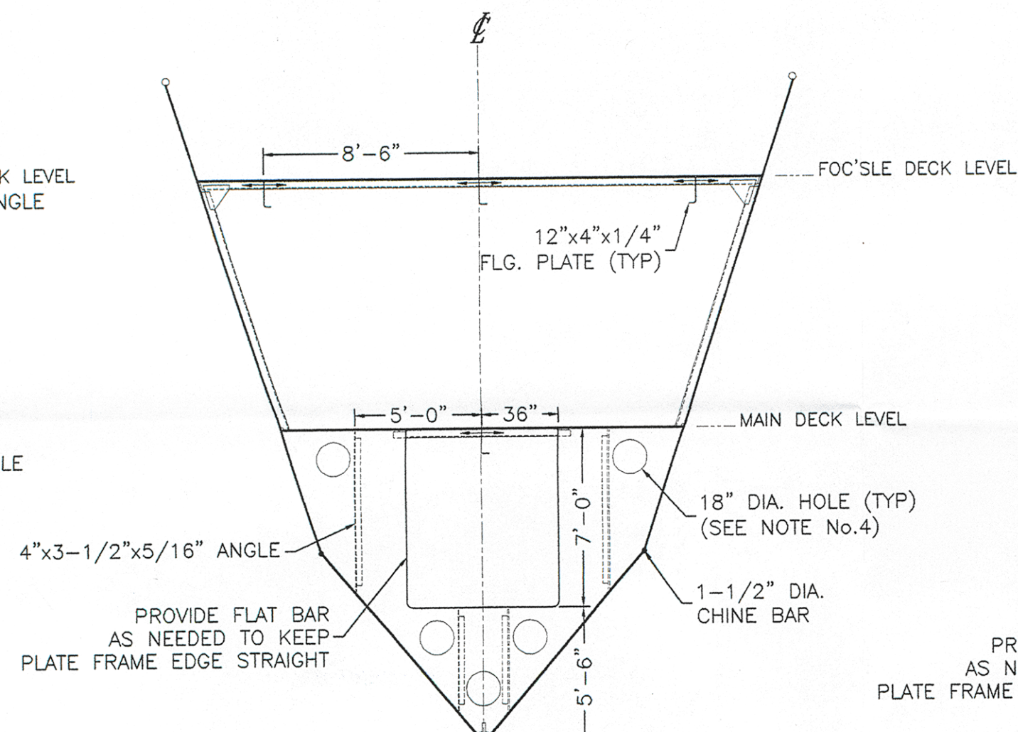
FRAME No.5 LOOKING AFT
