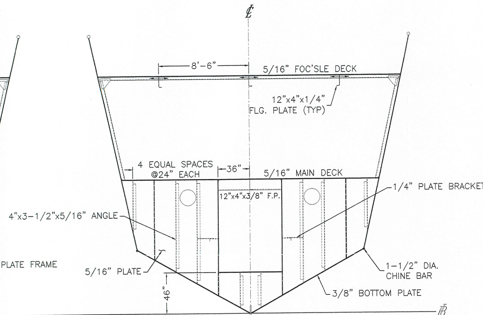
FRAME No.9 LOOKING AFT
