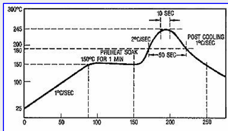
Figure 6. Infra-Red Reflow Soldering Temp/Time Profile
