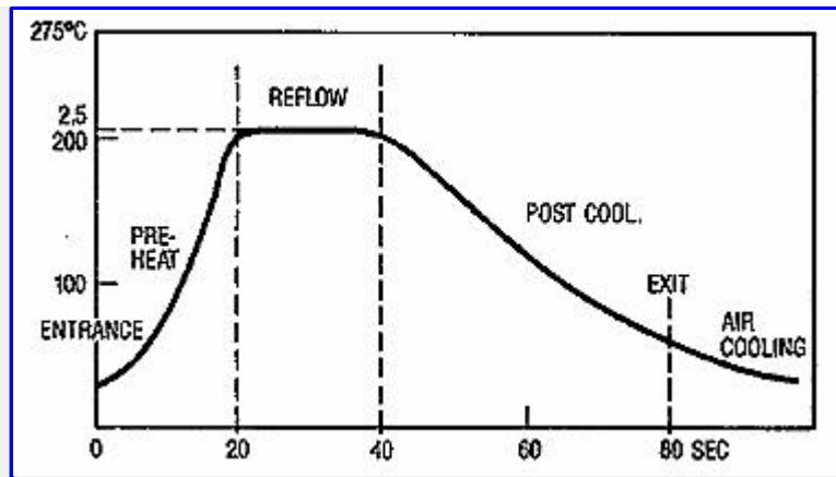
Figure 5. Vapor Phase Soldering Temp/Time Profile
