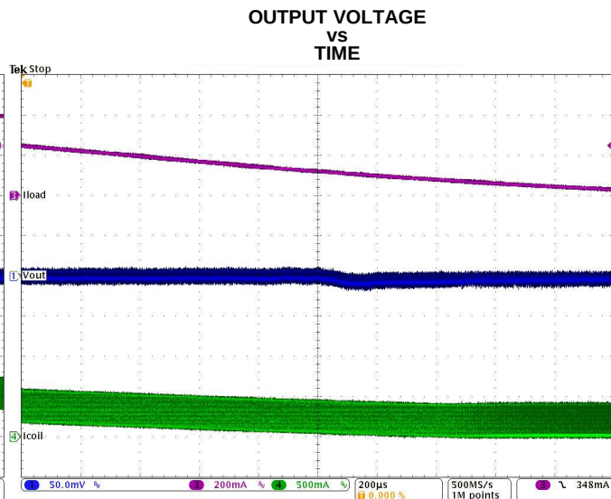
Figure 24. PSM to PWM Mode Transition
