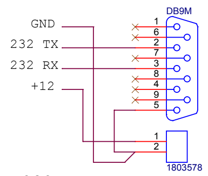
232 CONNECTION DETAIL PORTS 5-10
