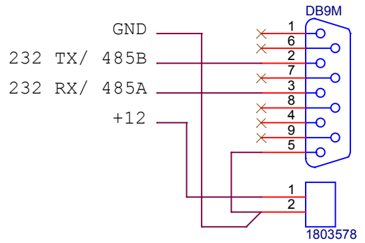
232/485 CONNECTION DETAIL PORTS 1-4
