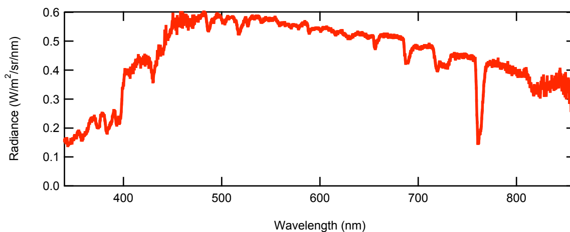
Channel A Example Calibrated Data (Full sun reflected from Spectralon)
