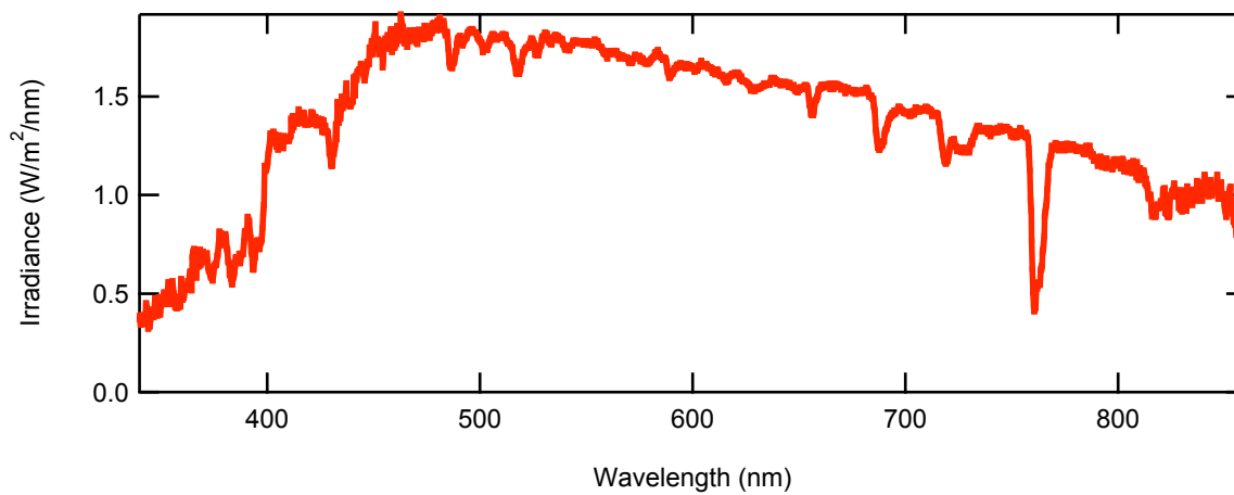
Channel B Example Calibrated Data (Full Sun)
