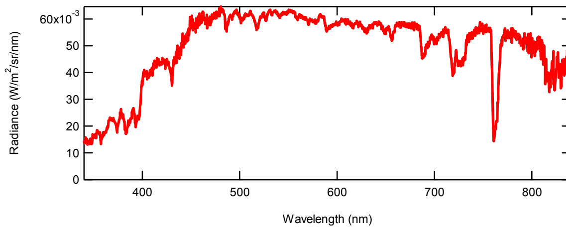
Channel B Example Calibrated Data (Reflection from Spectralon, hazy sky)
