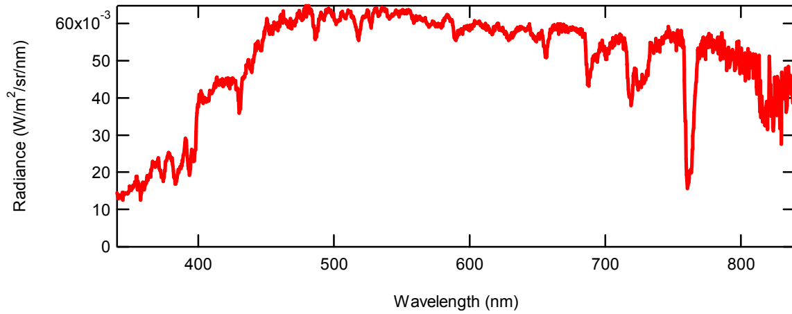
Channel C Example Calibrated Data (Reflection from spectralon, hazy sky)
