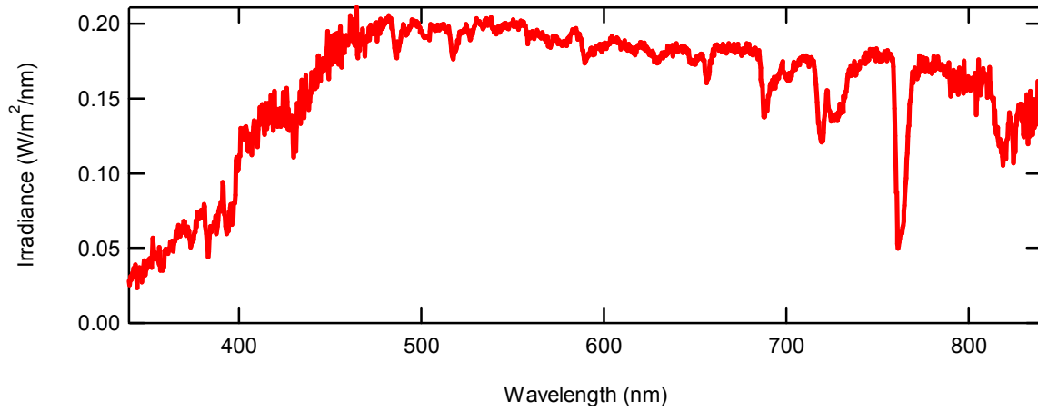
Channel A Example Calibrated Data (Direct sunlight, hazy sky)
