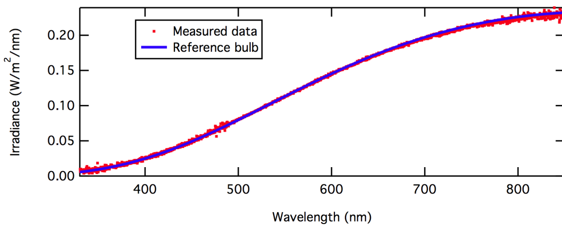
Channel C Example Calibrated Data (Direct Sunlight)
