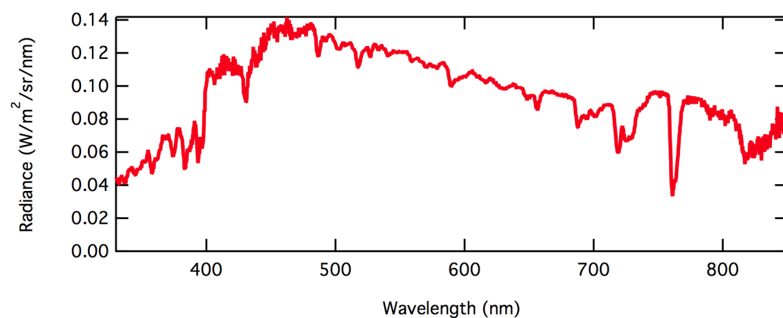
Channel A Example Calibrated Data (Sunlight reflected from clay soil)
