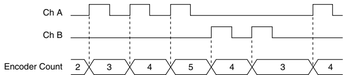
Figure 18. Two-Pulse Encoder
