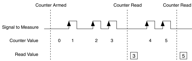
Figure 3. Edge Counting
