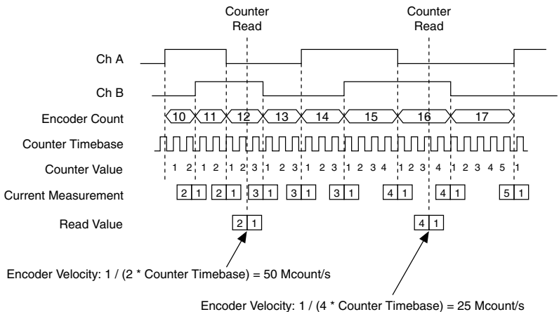
Figure 21. Quadrature Encoder Velocity Measurement
