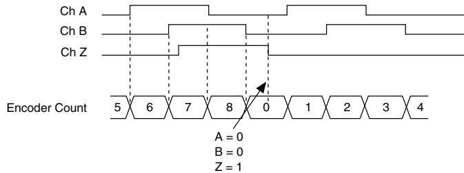
Figure 17. Channel Z Reload
