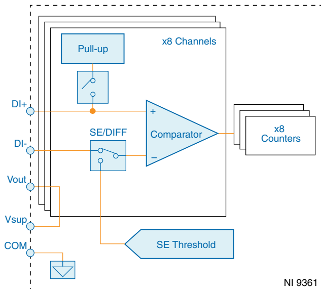
Figure 1. NI 9361 Input Circuitry
