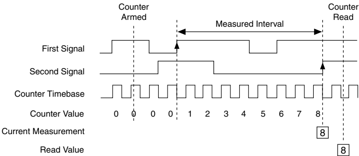
Figure 13. Two-Edge Separation
