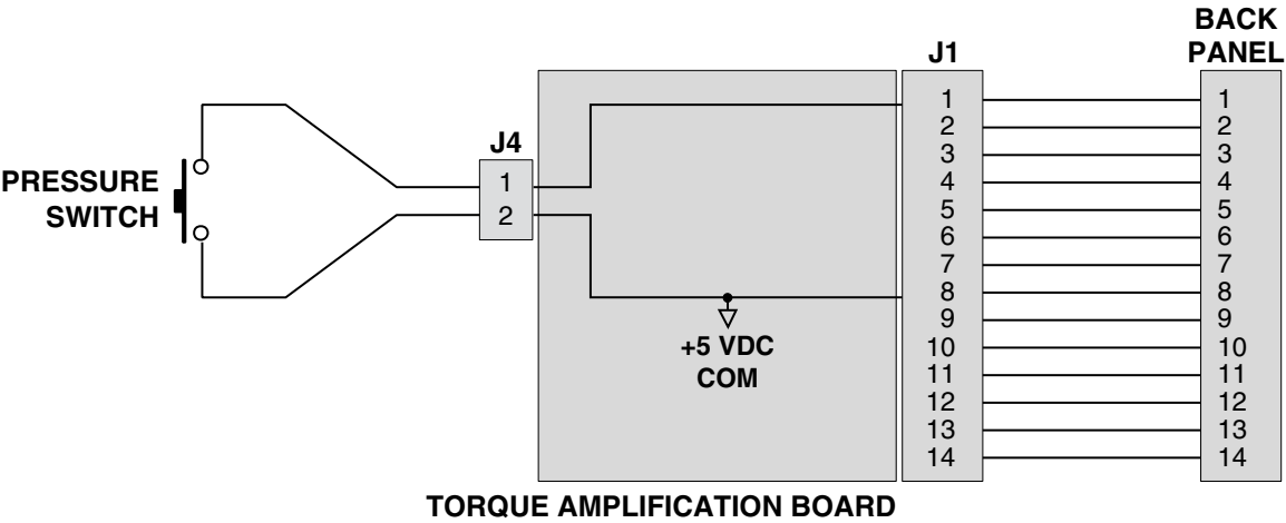
Figure 3–9 Air Flow Sensor Schematic
