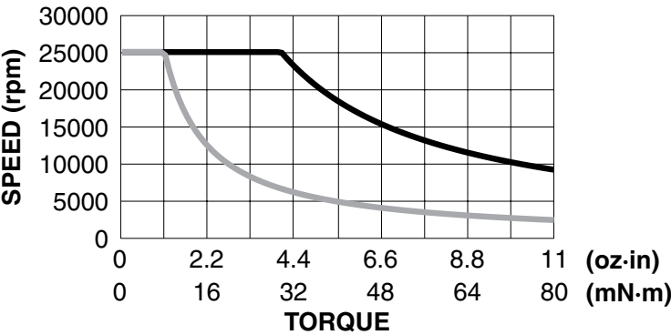
Figure 4-3 HD 100 Power Absorption Curve
