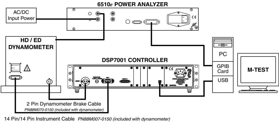
Figure 3–8 Dynamometer with 6510e Power Analyzer, DSP7001 Controller and M-TEST Software
