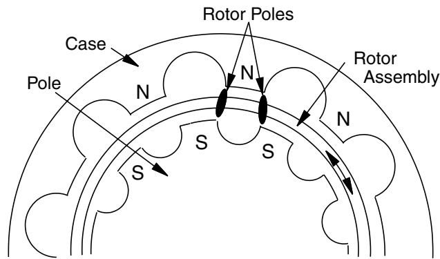
Figure 4-23 Hysteresis Brake Cross-Section
