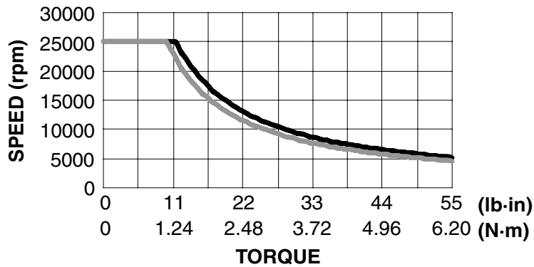
Figure 4-12 HD 715 Power Absorption Curve
