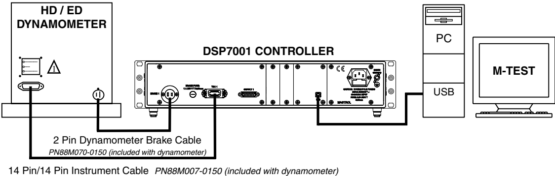
Figure 3–7 Dynamometer with DSP7001 Controller and M-TEST Software
