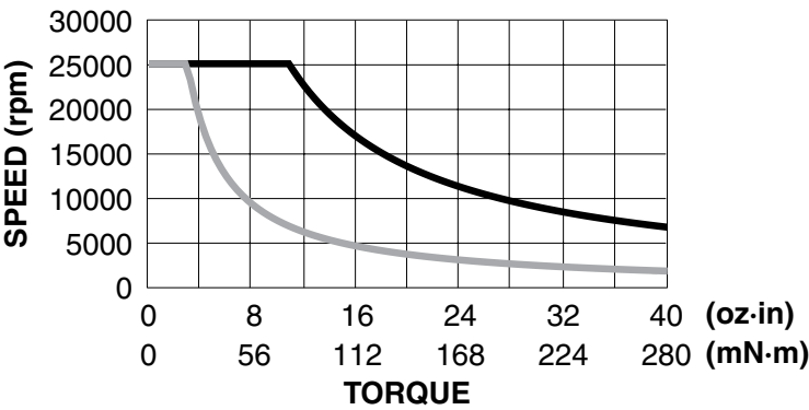
Figure 4-4 HD 400 Power Absorption Curve
