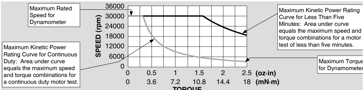
Figure 4-1 Power Absorption Curve Parameters
