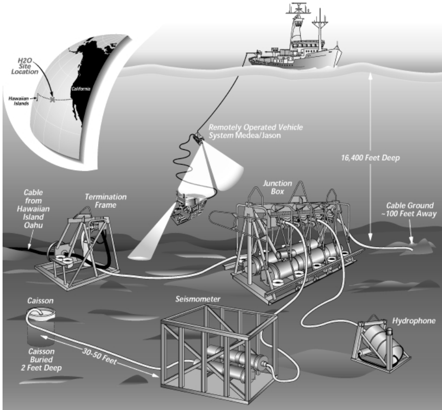
FIGURE 3-3 The H2O, the first deep-sea cabled research observatory, was established in 1998 using the retired Hawaii-2 coaxial telecommunications cable. A seafloor junction box in 5,000 m of water provides power and data communication for up to six instruments including a broad-band seismometer. More than 35,000 km of electro-optical telecommunications cable will be retired in place by industry within the next few years, providing a potentially significant resource for ocean observatory science. Figure courtesy of Jayne Doucette, ©Woods Hole Oceanographic Institution.
