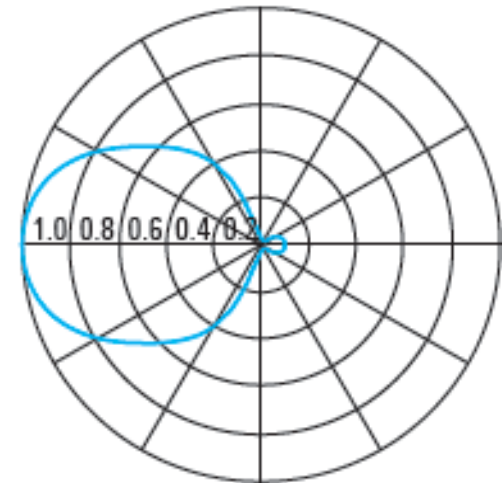
Typical gain pattern of a handheld DF antenna – note the directivity
