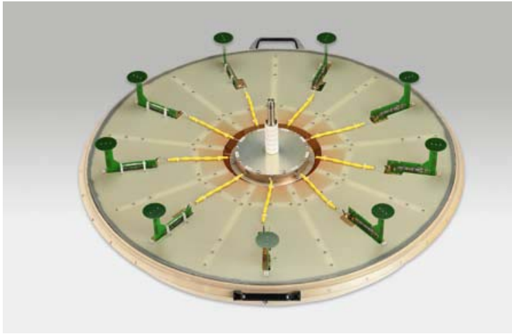
Inside the radome of a 9-element correlative interferometer antenna
