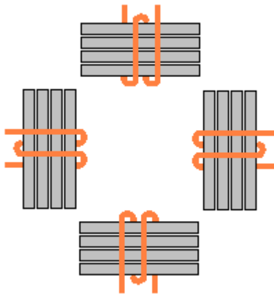
Crossed ferrite loops
