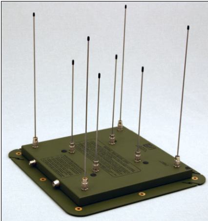
Figure 7 - DMA-1315B1 80-520 MHz Mobile Adcock DF Antenna
