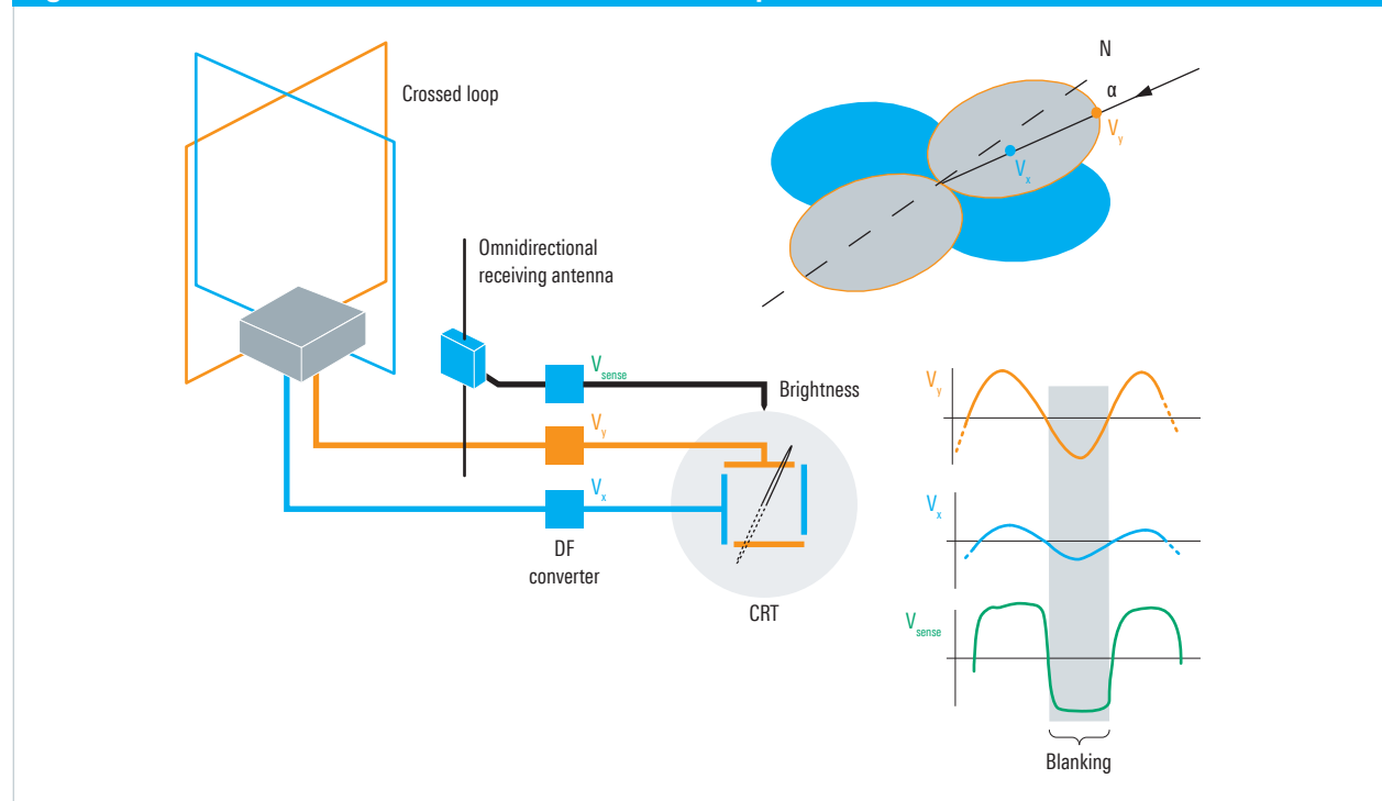
Fig. 8: Watson-Watt direction finder with crossed-loop antenna
