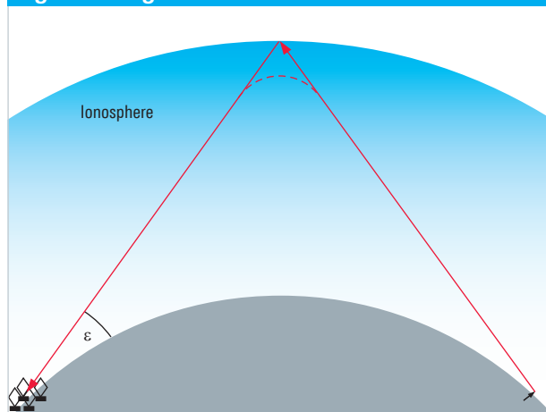
Fig. 34: Single station location
