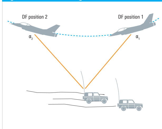
Fig. 33: Position finding
