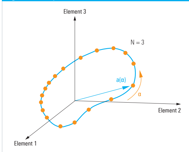
Array manifold characterizing an antenna array.
