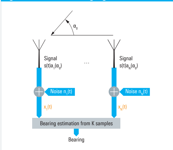
Fig. 36: Model describing signal and noise
