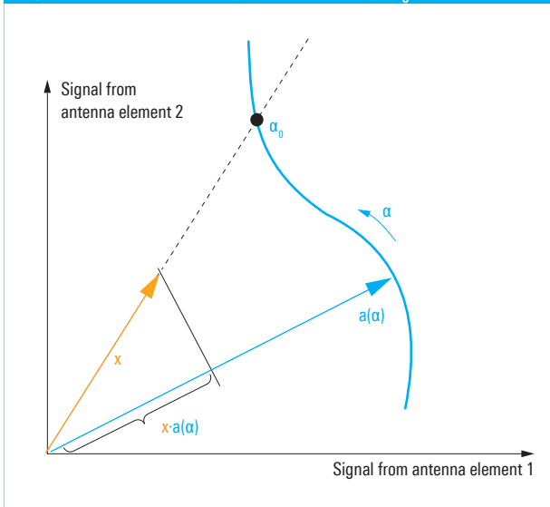
Fig. 22: Determining the bearing \alpha_0
