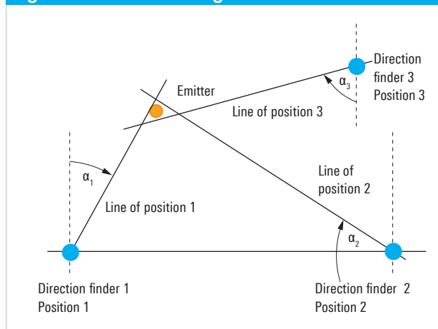
Fig. 32: Position finding
