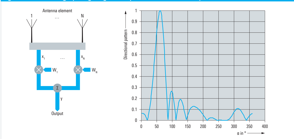
Fig. 23: Beamforming by weighting the outputs of an antenna array
