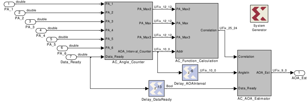
Figure 3.10 Block Diagram of the Amplitude Comparison Implementation
