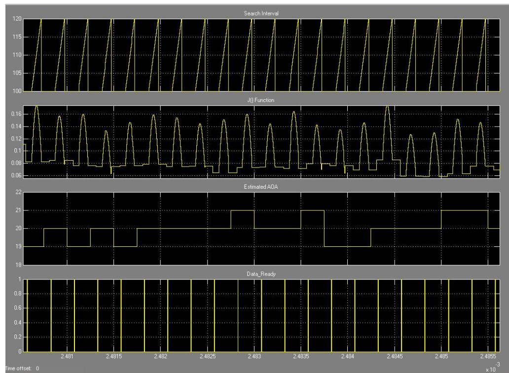
Figure 3.44 Screen Shot from System Generator (Implementation of Phase Comparison Algorithm)
