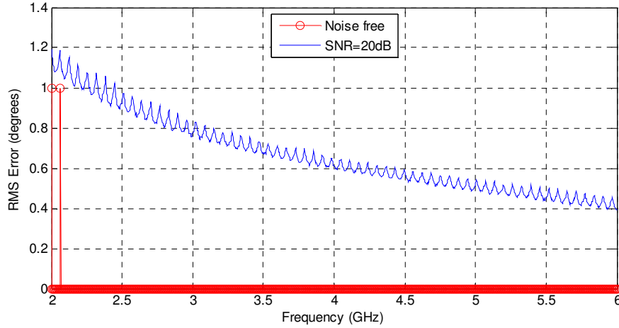
Figure 3.36 The RMS Error vs. Frequency when f_{\text{resolution}}=64 MHz (AOA=30 degrees)
