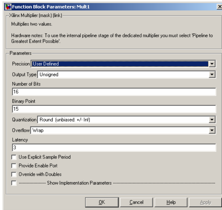
Figure C.1 Function Block Parameters of a Xilinx Multiplier Block
