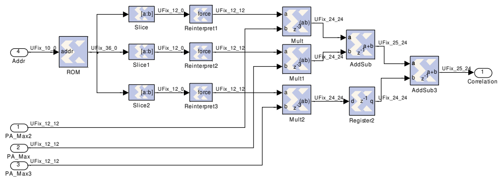
Figure 3.16 Logic Diagram of the AC_Correlation_Computation Block
