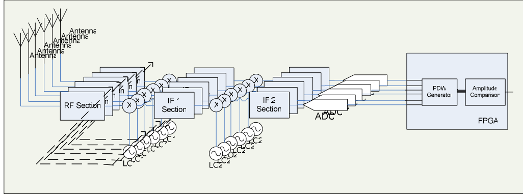
Figure 3.1 Block Diagram of the Amplitude Comparison DF System
