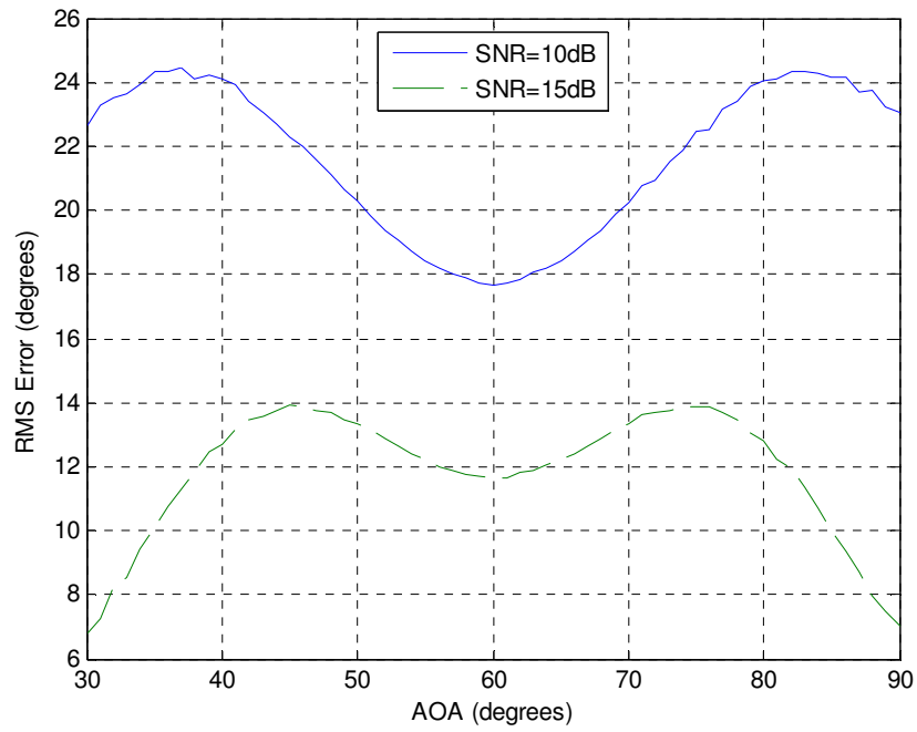
Figure 3.6 RMS Error vs. AOA (SNR is equal to 10dB and 15dB)
