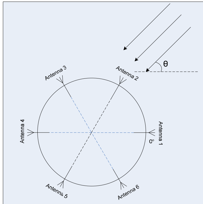
Figure 2.1 Circular Array Geometry ( N=6 )
