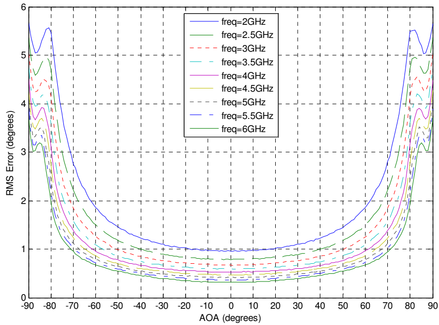
Figure 3.32 RMS Error vs. AOA when Frequency is varied from 2 GHz to 6 GHz in steps of 500MHz at SNR = 20dB.
