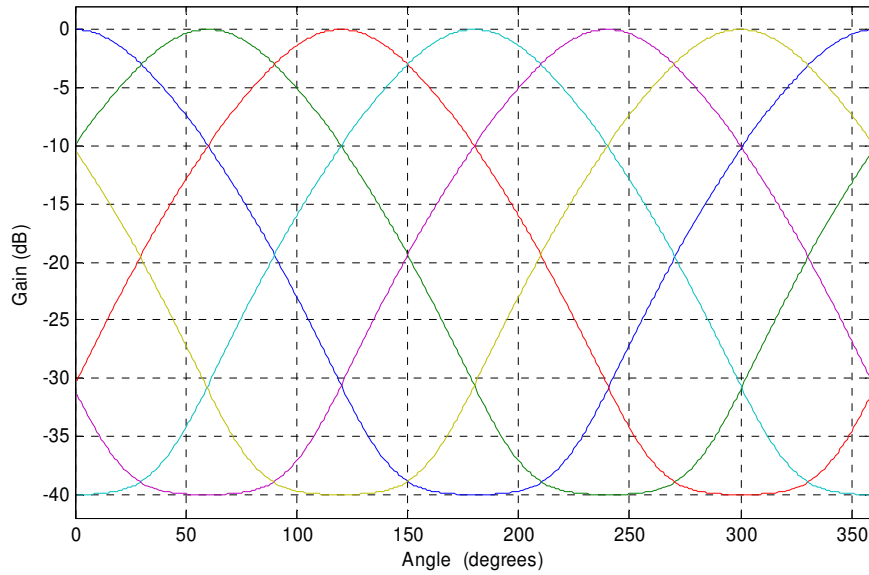
Figure 3.2 Amplitude Comparison Antenna Gain vs. Angle
