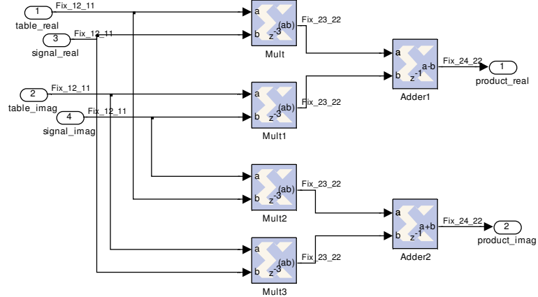
Figure 3.42 Logic Diagram of Complex_Multiplier_2 Block
