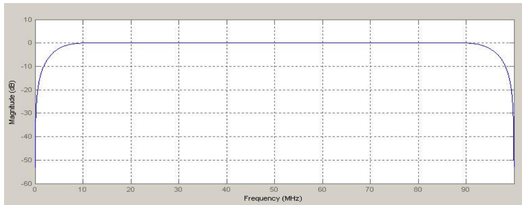
Figure 3.52 Magnitude Response of FIR Filter (Hilbert Transformation)
