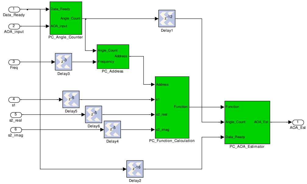
Figure 3.55 Block Diagram of the Phase Comparison Implementation
