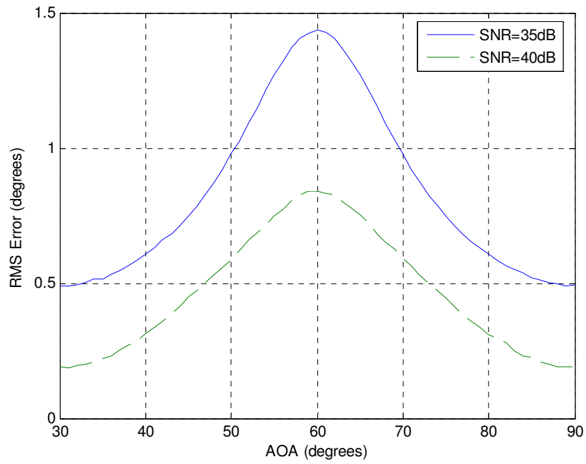
Figure 3.5 RMS Error vs. AOA (SNR is equal to 35dB and 40dB)
