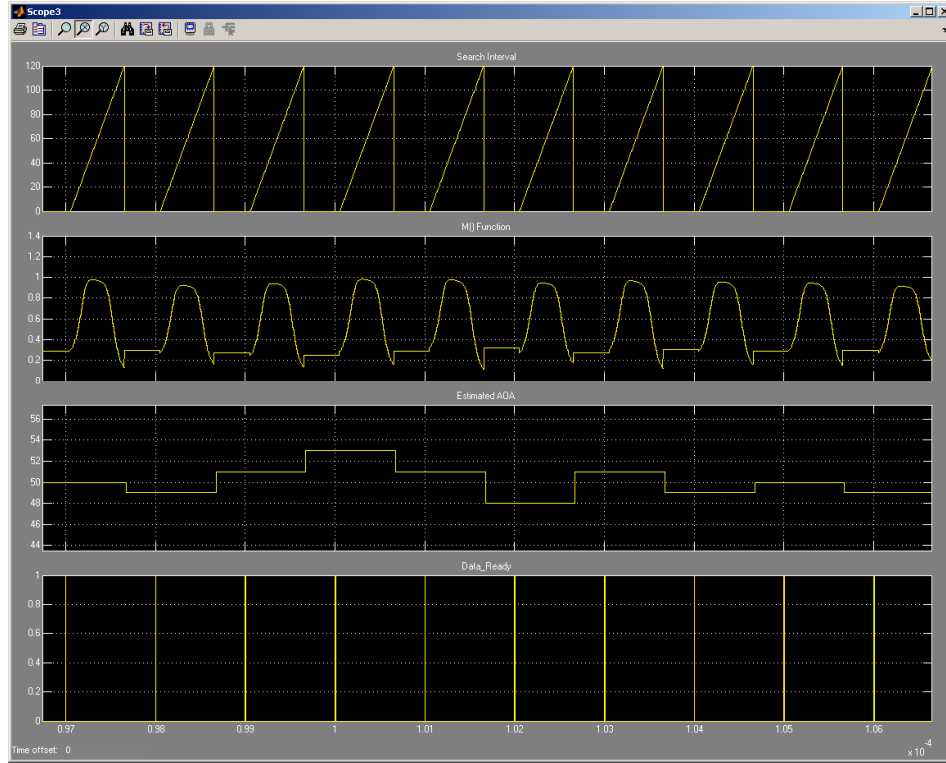
Figure 3.18 Screen Shot from System Generator (Implementation of Amplitude Comparison)
