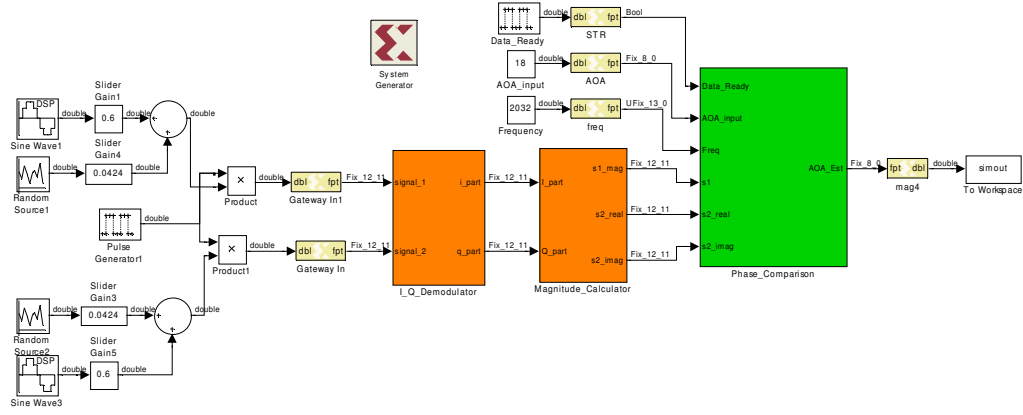
Figure 3.49 Block Diagram of Phase Comparison Implementation
