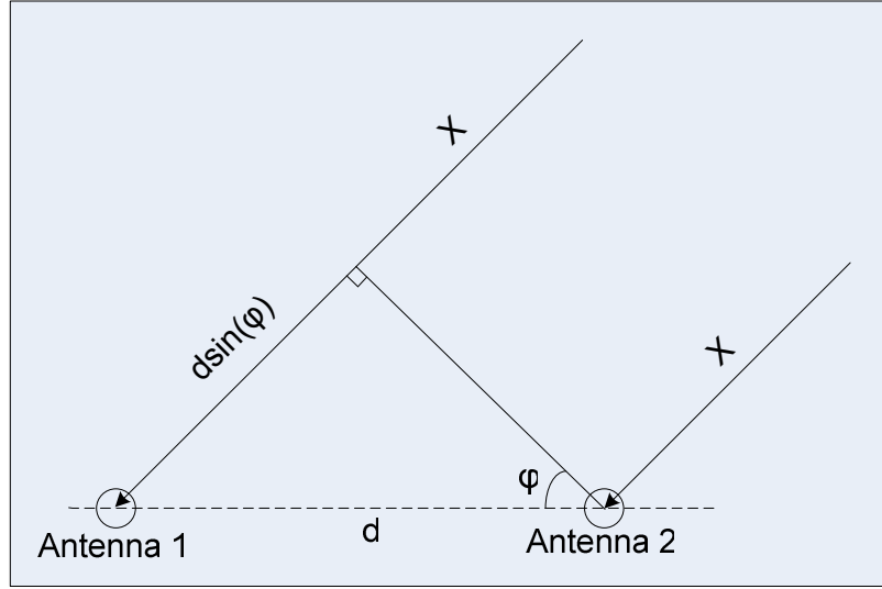
Figure 3.22 Single Baseline Interferometer
