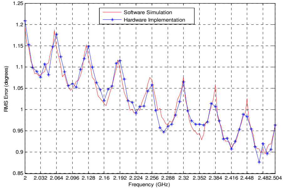
Figure 3.48 RMS Error of Hardware Implementation due to Frequency Quantization
