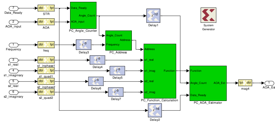
Figure 3.37 Block Diagram of Phase Comparison Implementation
