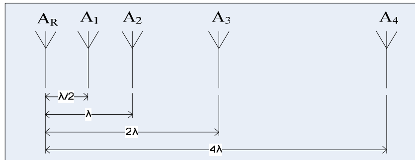
Figure 1.1 Harmonic Binary Related Interferometer
