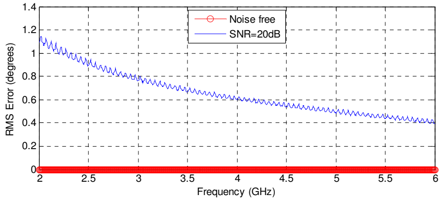
Figure 3.35 The RMS Error vs. Frequency when f_{\text{resolution}} = 50 MHz (AOA=30 degrees)
