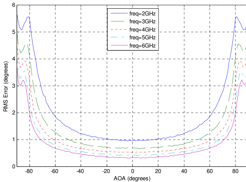
Figure 3.45 Phase Comparison Hardware Implementation RMS Error vs. AOA (SNR=20dB)
