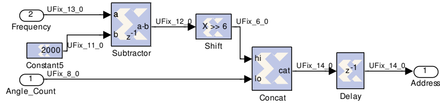
Figure 3.39 Logic Diagram of the PC_Address_Decoder Block
