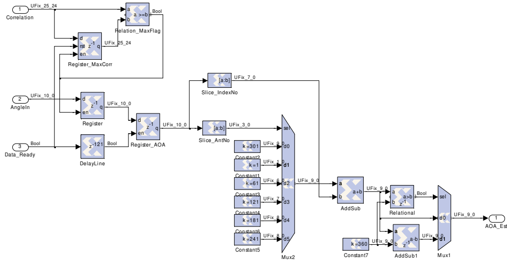
Figure 3.17 Logic Diagram of AC_AOA_Estimator Block
