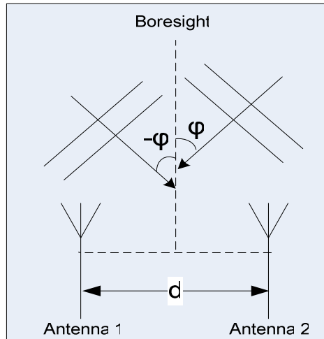
Figure 3.23 Phase Comparison Antenna Layout
