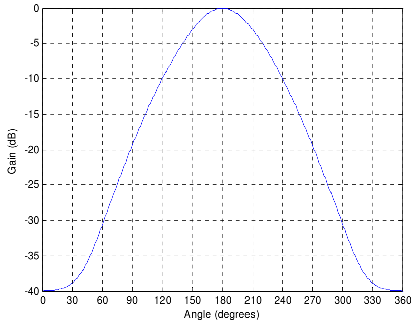
Figure A.1 Generated Antenna Pattern for Amplitude Comparison
