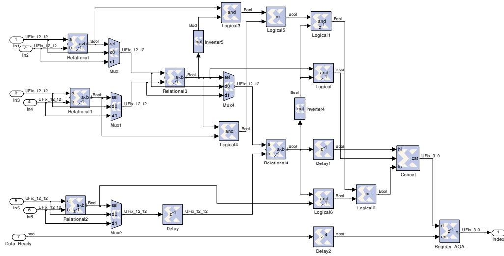
Figure 3.12 Logic Diagram of AC_Max_Amplitude_Finder Block
