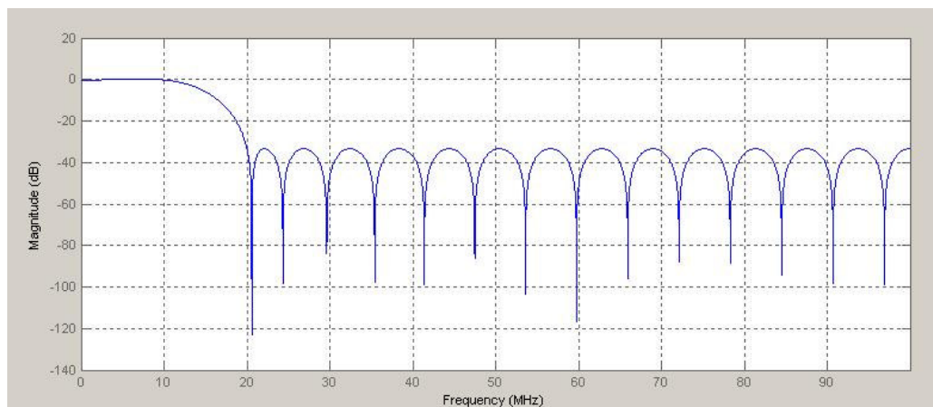
Figure 3.53 Magnitude Response of FIR LPF
