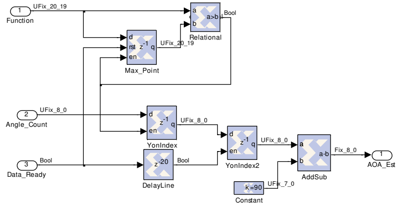
Figure 3.43 Logic Diagram of the PC_AOA_Estimator Block
