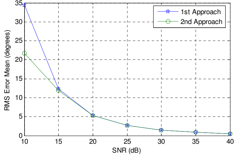
Figure 3.9 Mean of RMS Error vs. SNR
