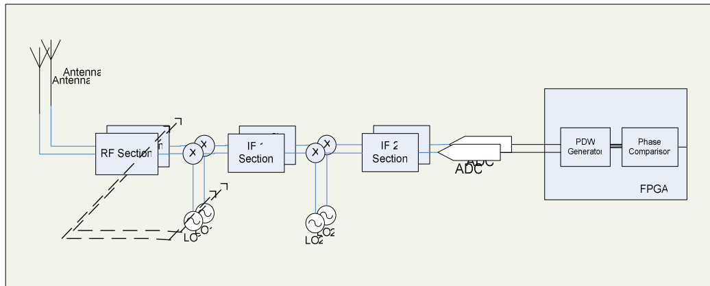
Figure 3.21 Block diagram of the Phase Comparison DF system
