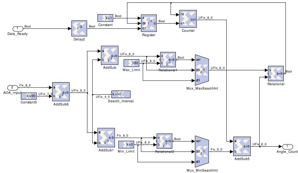
Figure 3.38 Logic Diagram of the PC_Angle_Counter Block
