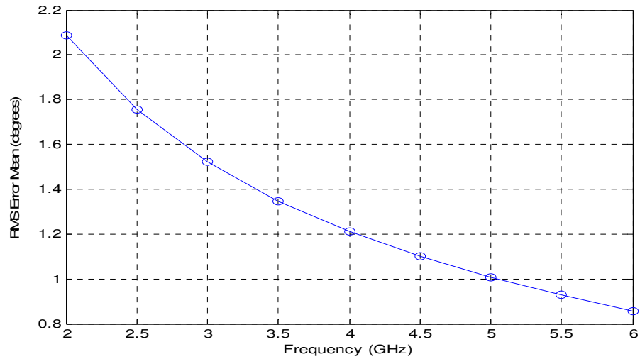
Figure 3.33 Mean of the RMS Error vs. Frequency at SNR=20dB.
