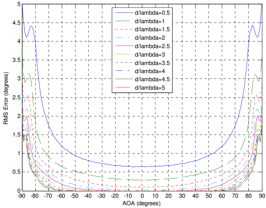
Figure 3.30 Phase Comparison RMS Error vs. AOA at d/\lambda value from 1 to 5 in steps of 0.5 (SNR = 30 dB)
