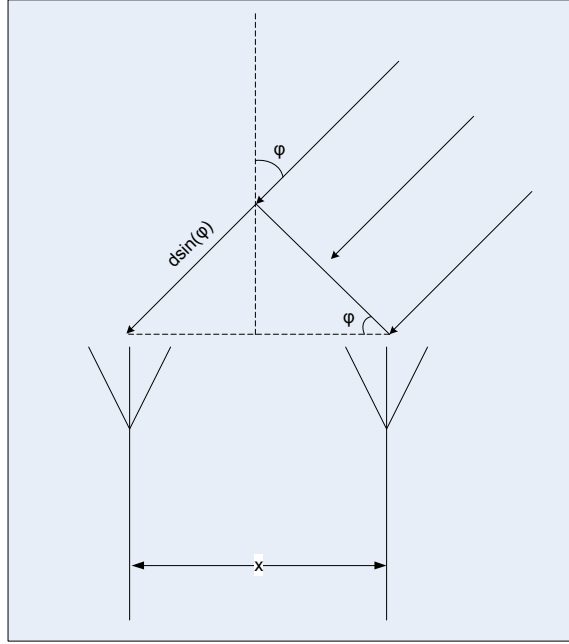
Figure 2.2 Phase Array Geometry
