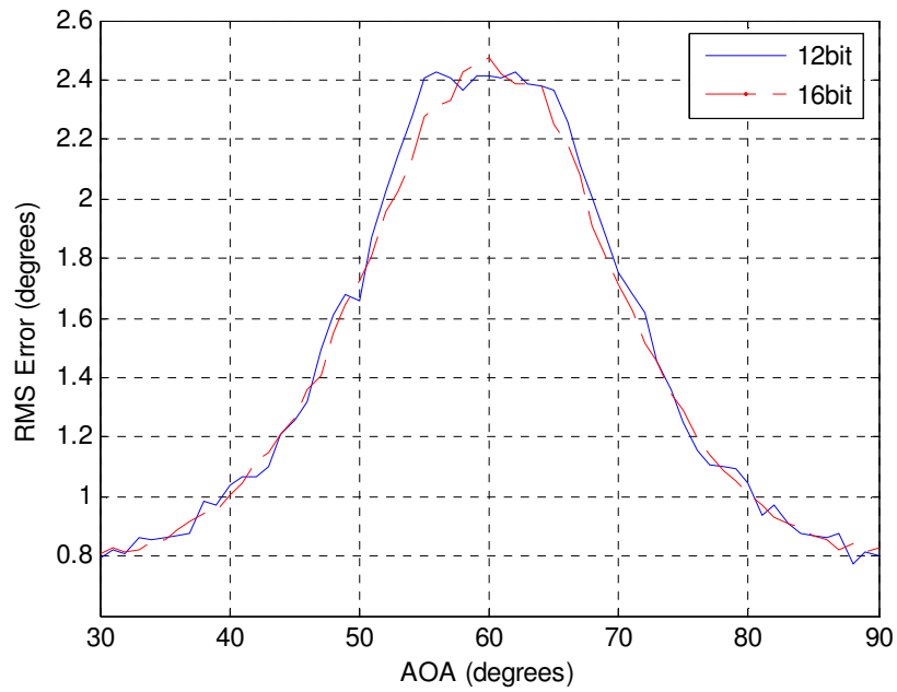
Figure 3.20 RMS Error vs AOA of Amplitude Comparison Hardware Implementation at 30dB SNR
