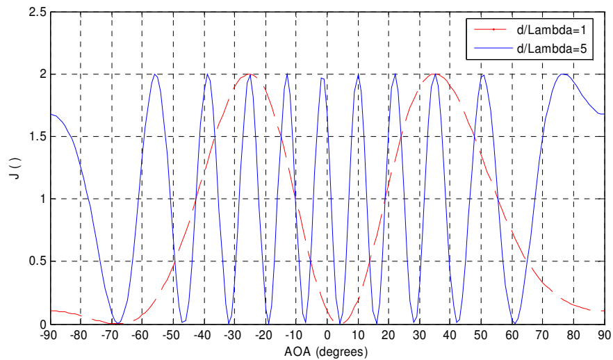
Figure 3.26 Typical Plot of J(\phi) vs. AOA for d/\lambda=1 and d/\lambda=5 (AOA=35)
