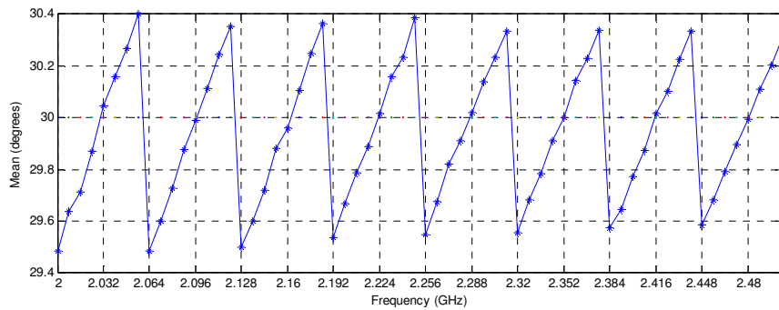
Figure 3.47 Mean of the Estimated AOA vs. Frequency
