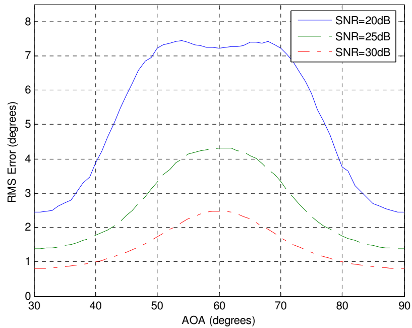
Figure 3.7 RMS Error vs. AOA (SNR is equal to 20dB, 25dB and 30dB )
