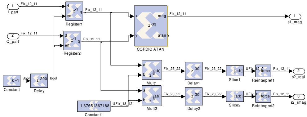
Figure 3.54 Logic Diagram of Magnitude_Calculator Block
