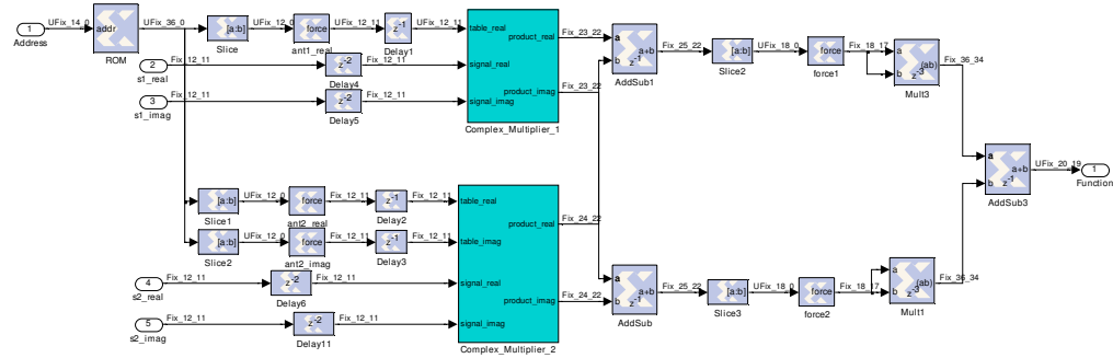
Figure 3.40 Logic Diagram of PC_Function Calculation Block
