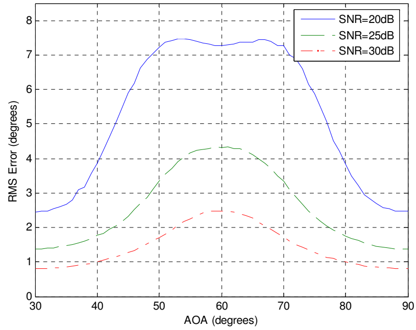
Figure 3.4 RMS Error vs. AOA (SNR is equal to 20dB, 25dB and 30dB)
