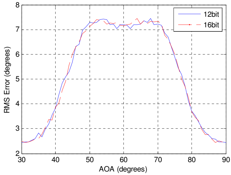
Figure 3.19 RMS Error vs AOA of Amplitude Comparison Hardware Implementation at 20dB SNR
