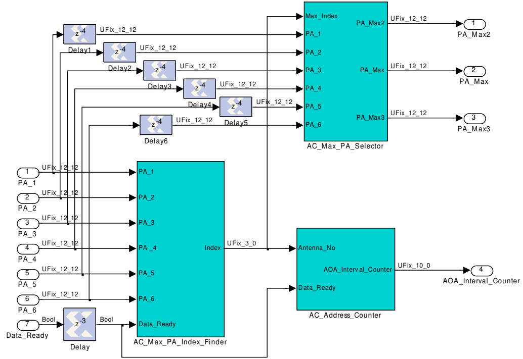
Figure 3.11 Logic Diagram of AC_Angle_Counter Block
