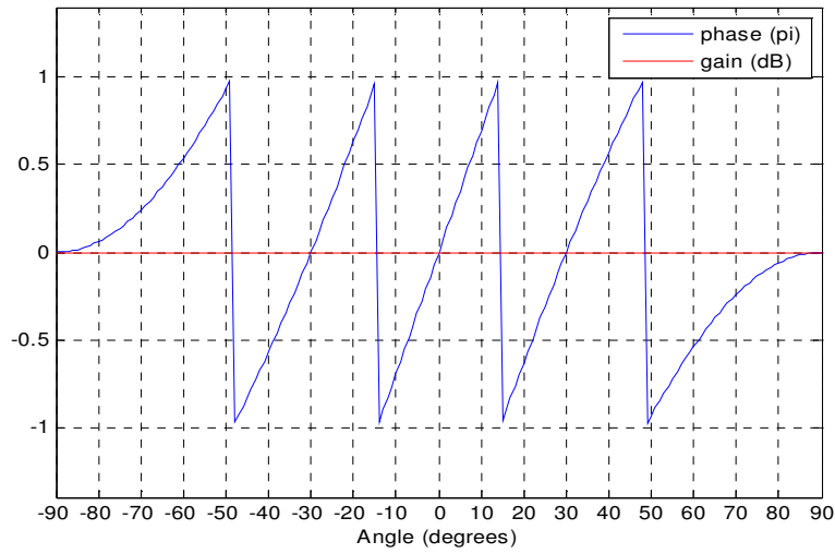
Figure 3.25 Phase Comparison Antenna Gain and Phase Pattern for d/\lambda=2
