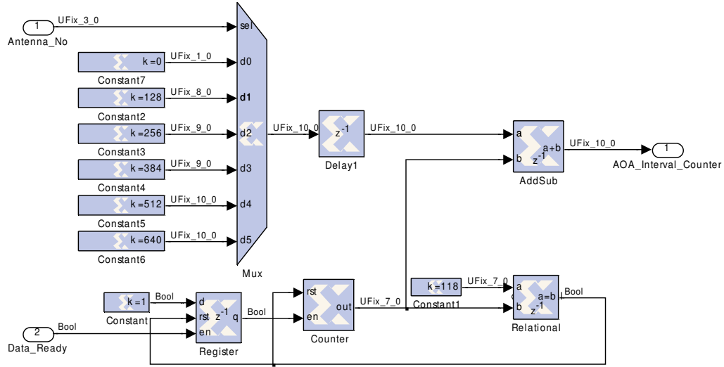
Figure 3.14 Logic Diagram of AC_Address_Counter Block
