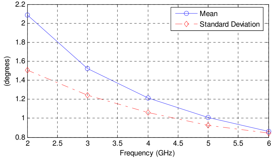
Figure 3.46 Mean and The Standard Deviation of RMS Error
