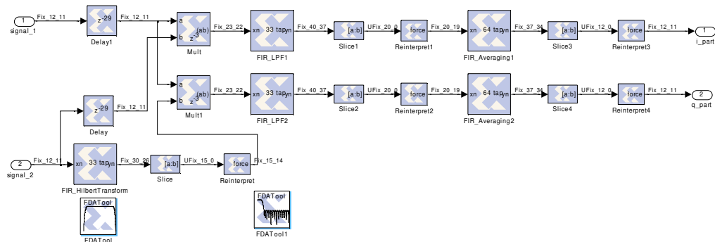
Figure 3.51 Logic Diagram of I and Q Demodulator Block
