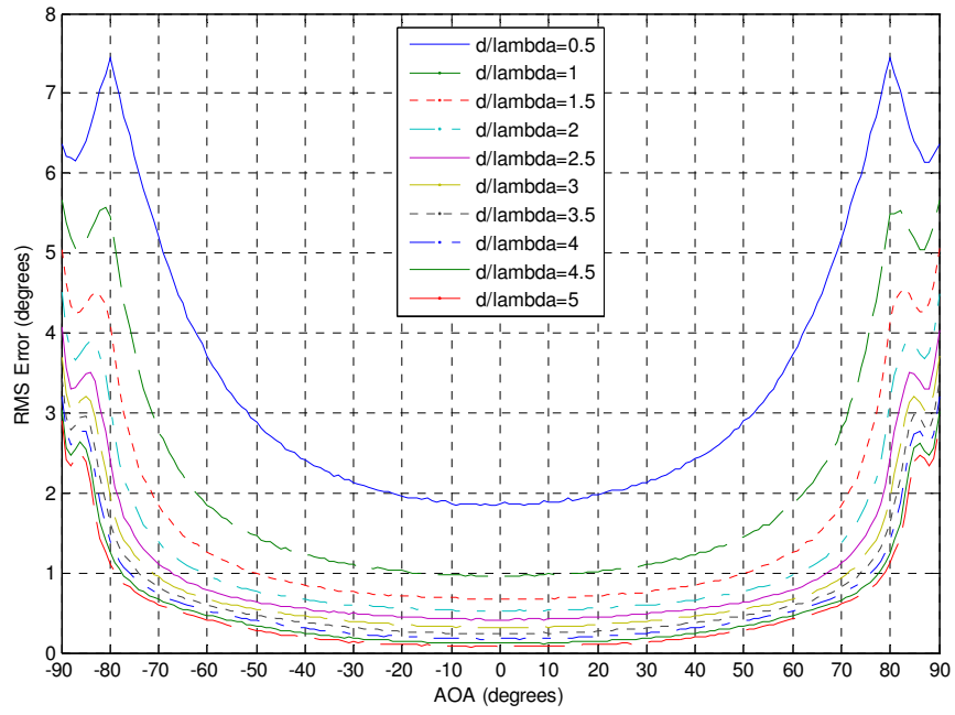
Figure 3.29 Phase Comparison RMS Error vs. AOA at d/\lambda value from 1 to 5 in steps of 0.5 (SNR = 20 dB)
