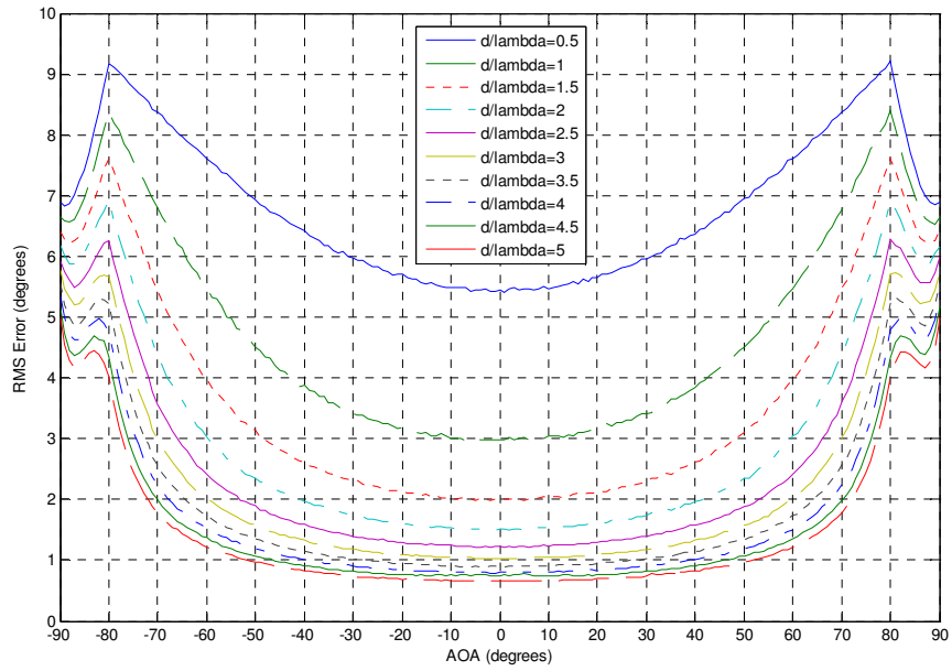
Figure 3.28 Phase Comparison RMS Error vs. AOA at d/\lambda value from 1 to 5 in steps of 0.5 (SNR = 10 dB)
