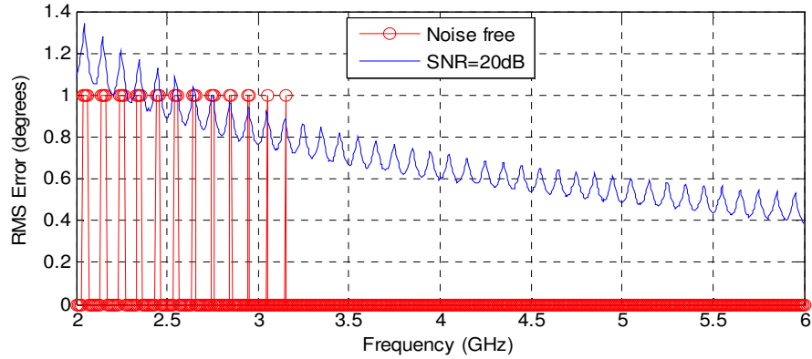
Figure 3.34 The RMS Error vs. Frequency when f_{\text{resolution}} = 100 MHz (AOA=30 degrees)
