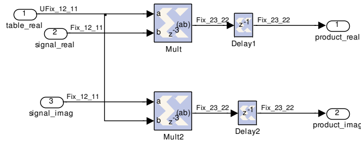
Figure 3.41 Logic Diagram of Complex_Multiplier_1 Block
