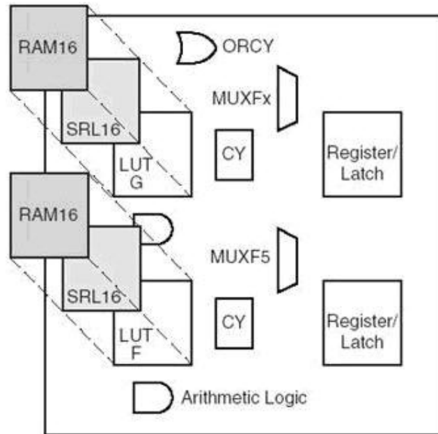
Figure B.1 Virtex Family FPGA Logic Slice
