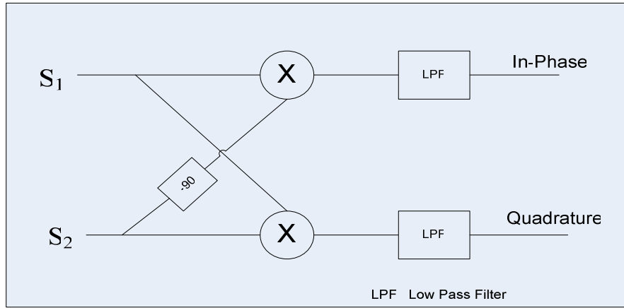
Figure 3.50 I and Q Demodulation
