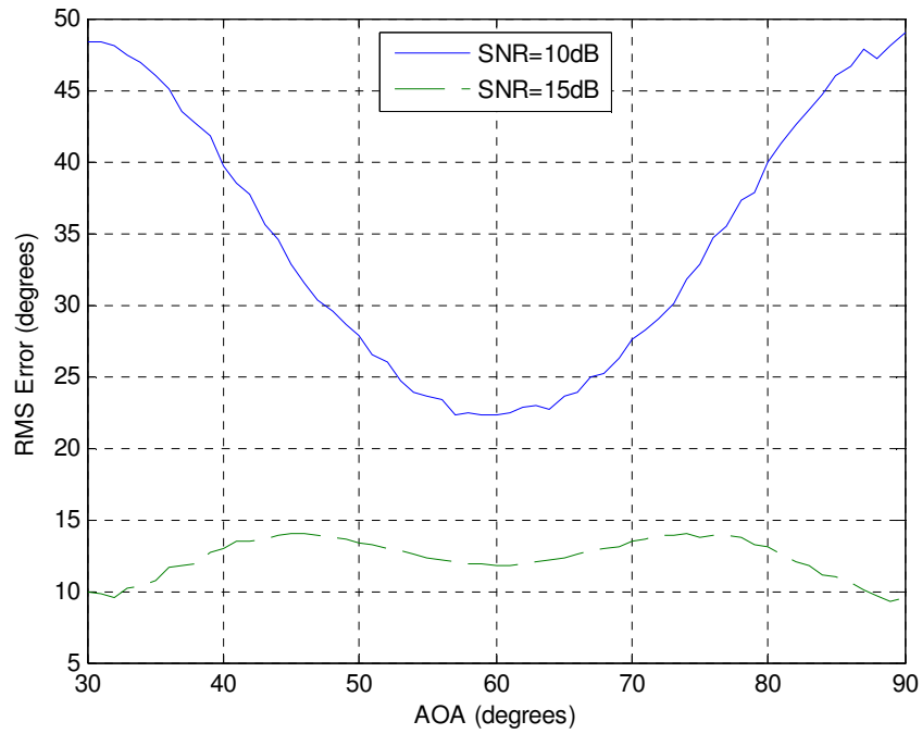
Figure 3.3 RMS Error vs. AOA (SNR is equal to 10dB and 15dB)
