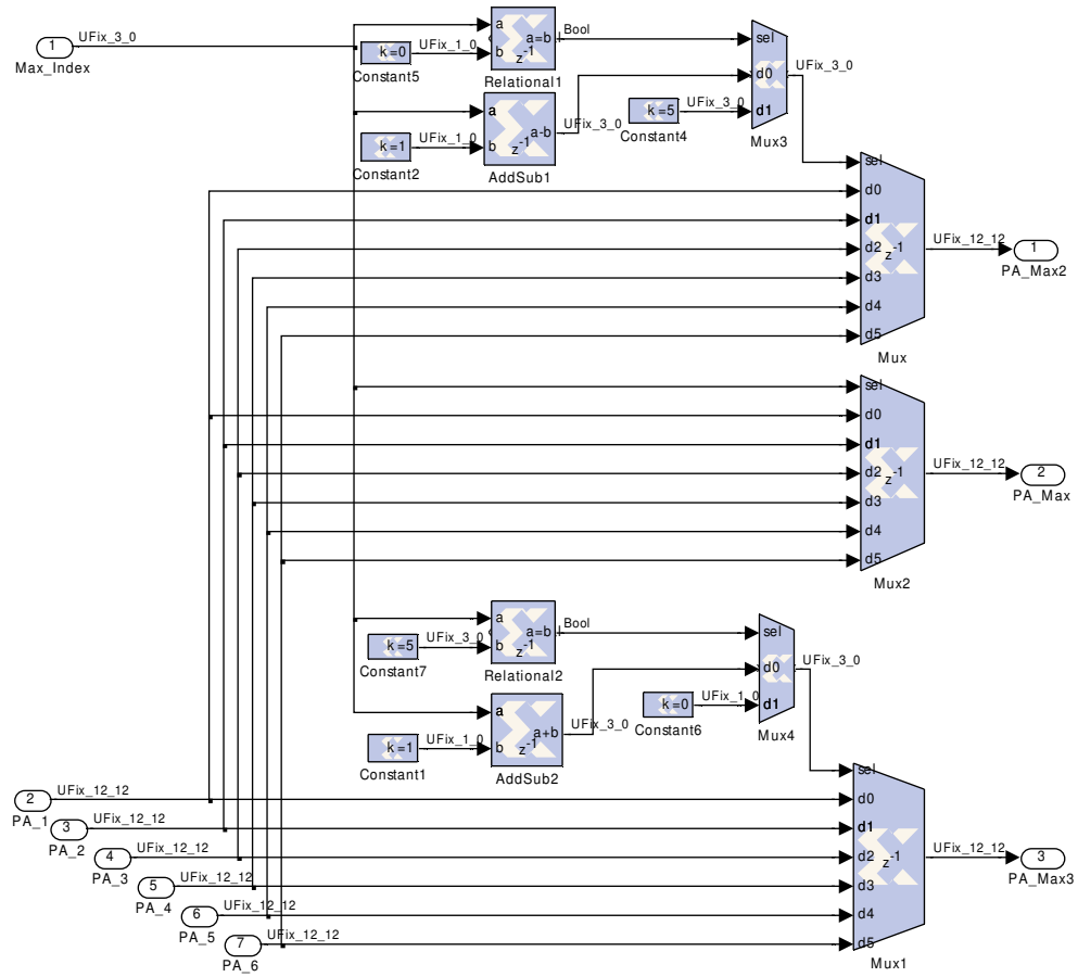
Figure 3.13 Logic Diagram of AC_Max_PA_Selector Block
