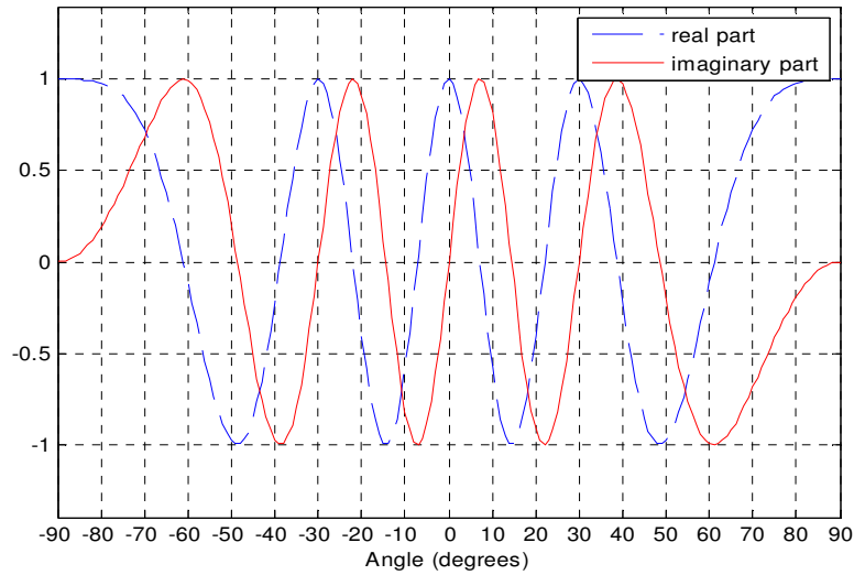
Figure 3.24 Real and Imaginary parts of Phase Comparison for d/\lambda=2
