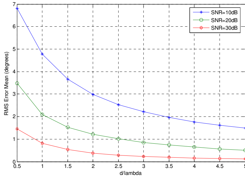
Figure 3.31 Mean of RMS Error vs. d/\lambda Values for SNR=10dB, 20dB and 30dB
