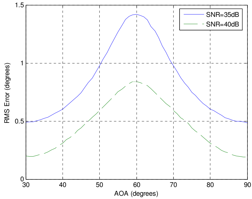
Figure 3.8 RMS Error vs. AOA (SNR is equal to 35 dB and 40dB)
