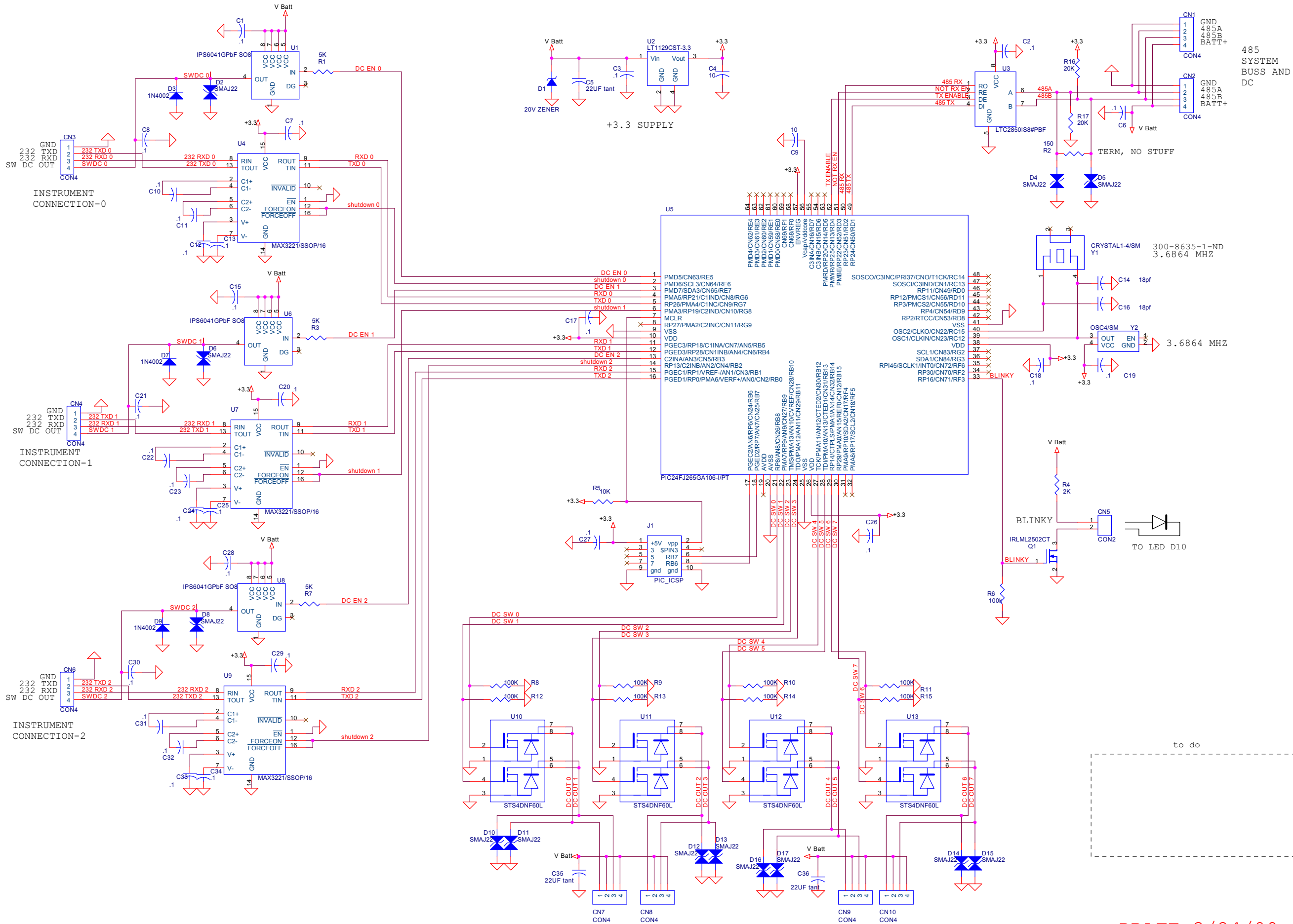
DC OUTPUTS FOR STIRRING, SAMPLING AND INJECTORS
