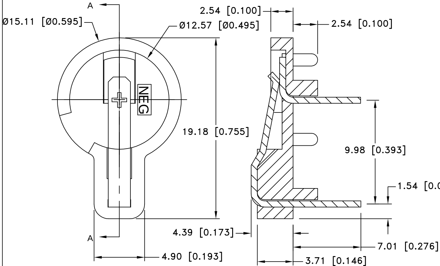
PCB LAYOUT
