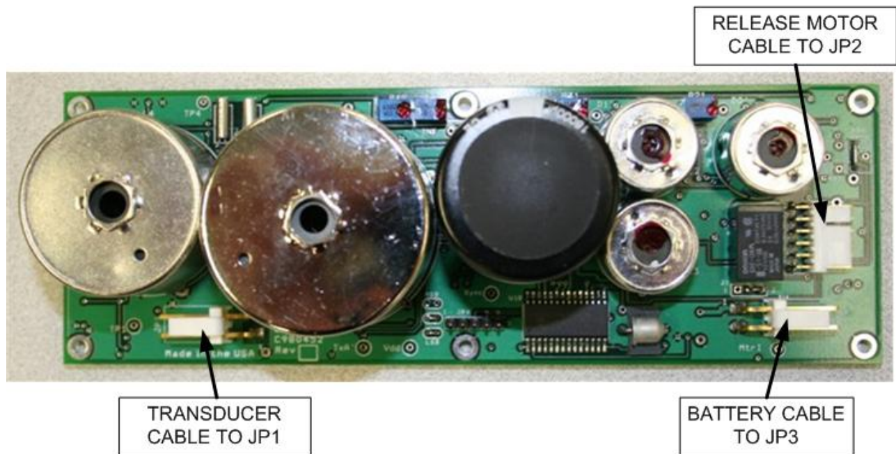
Figure 4 - PCB CONNECTORS
