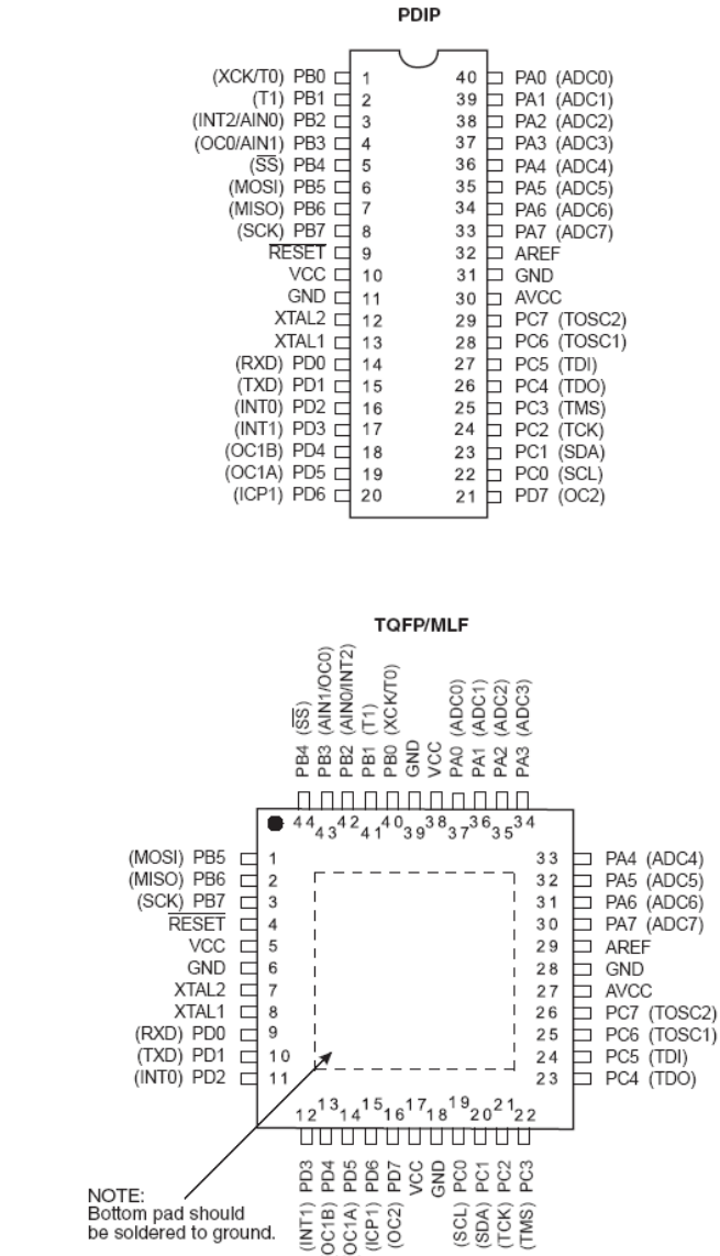
Figure 1. Pinout ATmega16
