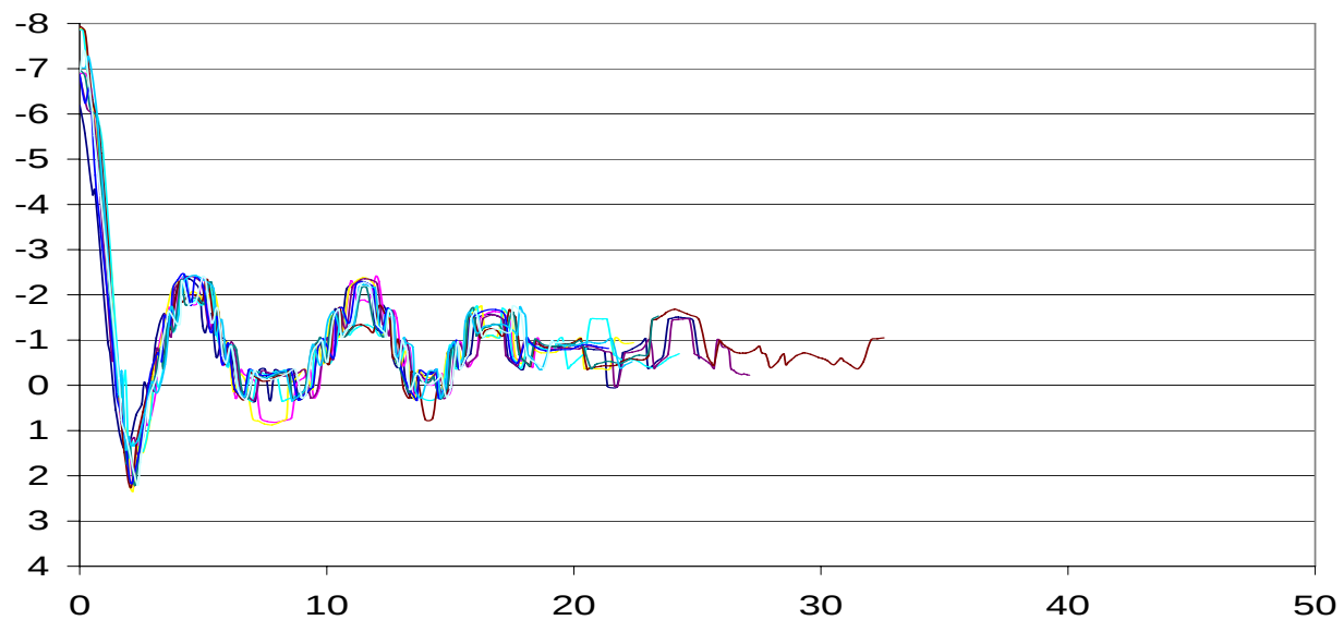
Bow Displacement Response with 16" Freeboard
