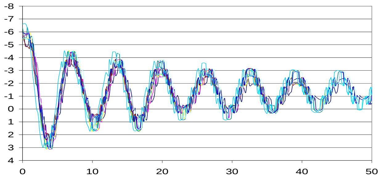
Bow Displacement Response with 8" Freeboard
