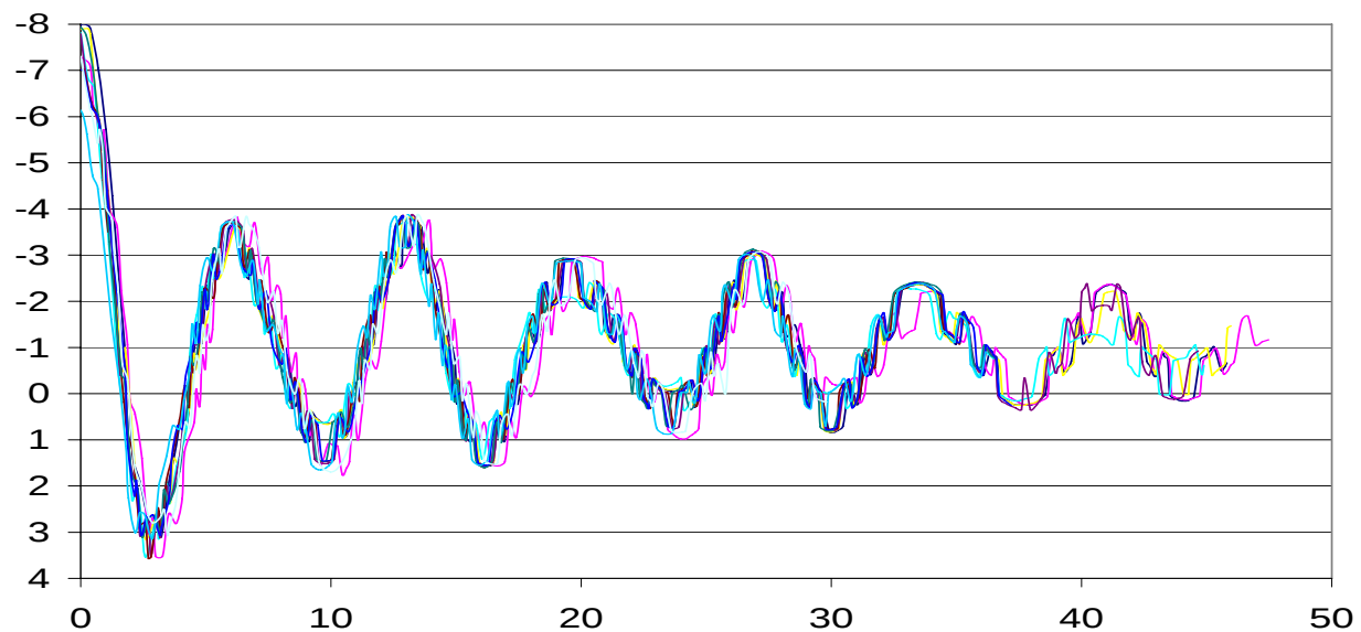
Bow Displacement Response with 12" Freeboard
