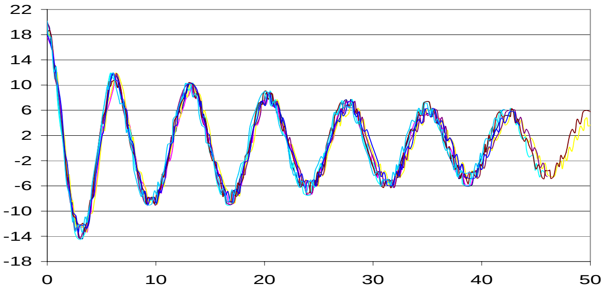
Side Displacement Response with 12" Freeboard
