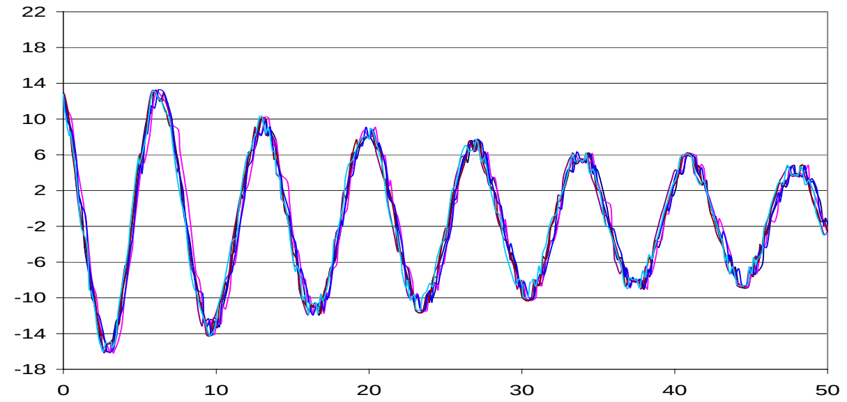
Side Displacement Response with 8" Freeboard
