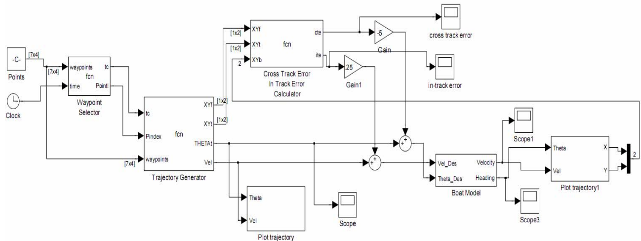
Figure 3.13 – Trajectory Controller Simu-link model. Using the system dynamics of the boat, a model in simu-link was able to be developed in order to test functionality of trajectory control. In the actual system, the boat model would be replaced with communications to the physical boat.
