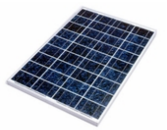
Figure 7.3-Solar Panel. The Kyocera KC85TS solar electric panel produces 87 peak watts and covers an area of .7 meters.[8]
