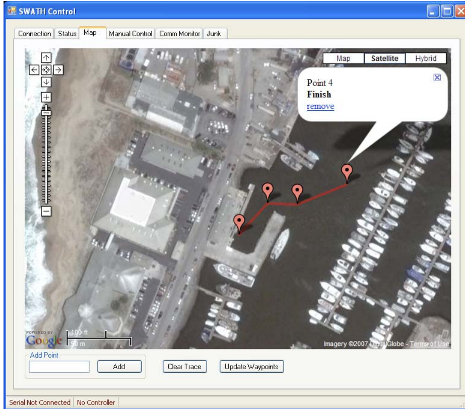
Figure 7.2- Google Maps Interface. Using C# hooks into JavaScript, Google Maps was able to be utilized for real time monitoring and way-point routing for the autonomous SWATH boat. The red icon represents the current position of the boat, and light red teardrops are way-points. The way-points can be nicknamed, drag-and-dropped, and rearranged in real time.
