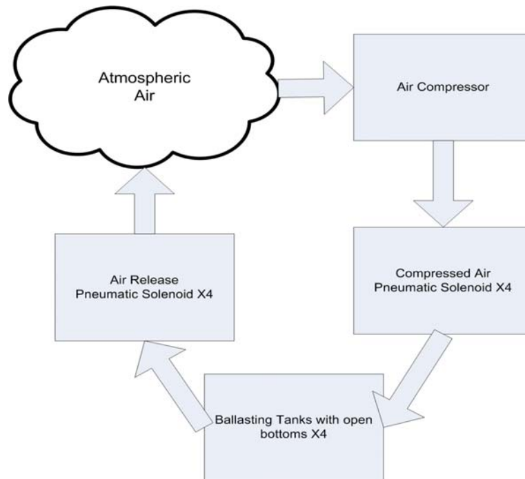
Figure 3.10 – Ballast System Diagram. The ballast system works by filling the ballast tanks with compressed air to displace water and increase lift, or releasing air to add water and decrease lift.
