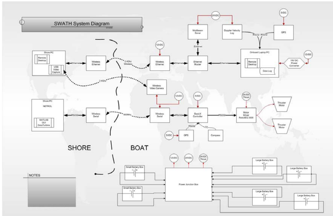
Figure 2.1 – SWATH System Level Diagram. This diagram shows the various subsystems on the boat, including the scientific, navigation and control, and power subsystems. Also shown are their power and communication paths.
