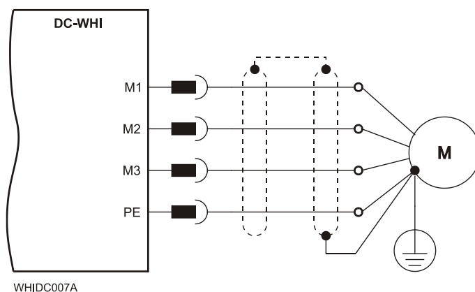
Figure 4: AC Motor Power Connection Diagram
