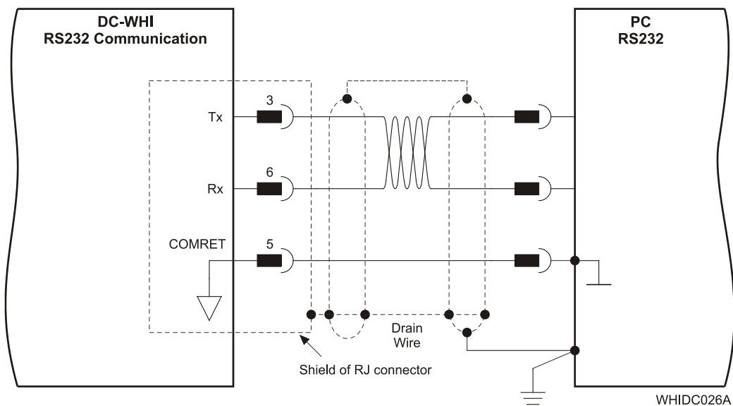
Figure 24: RS-232 Connection Diagram
