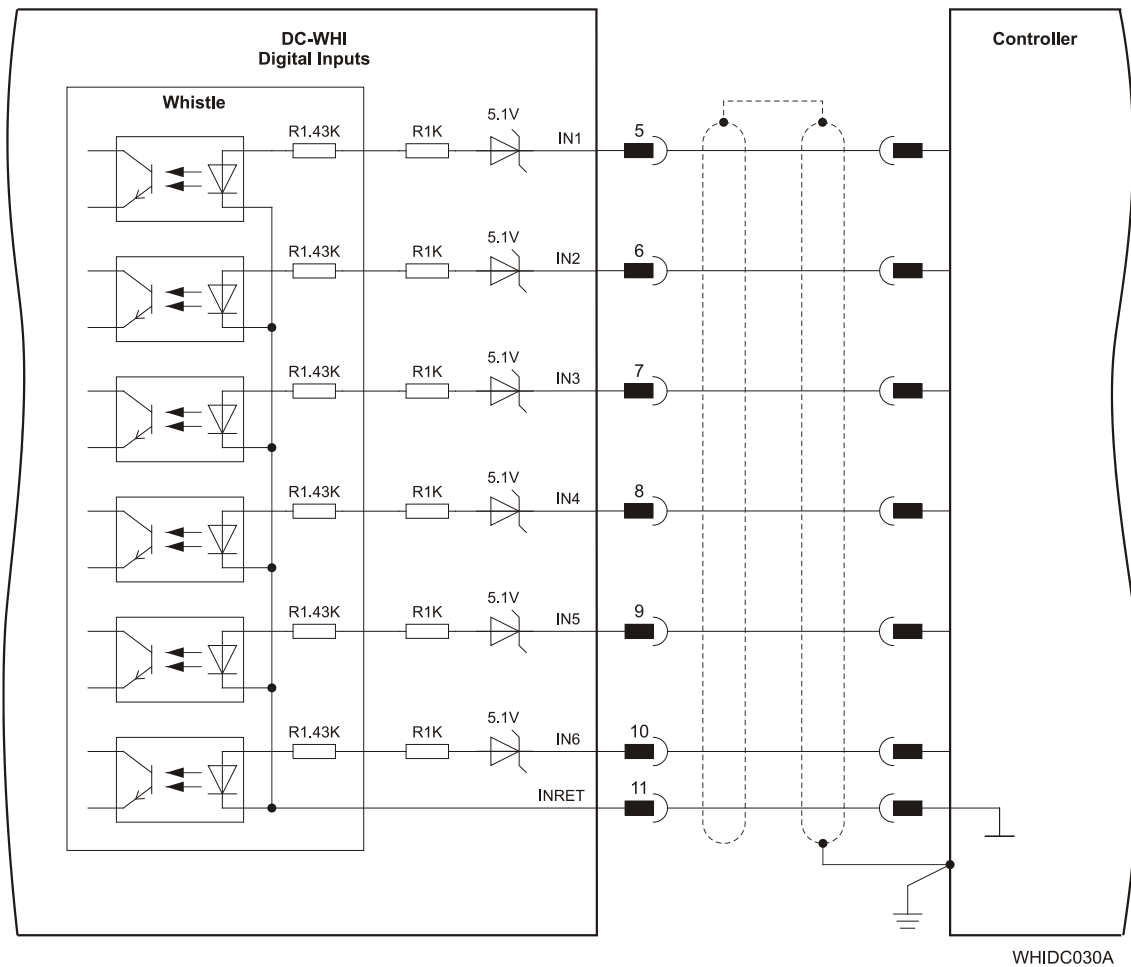
Figure 21: Digital Input Connection Diagram
