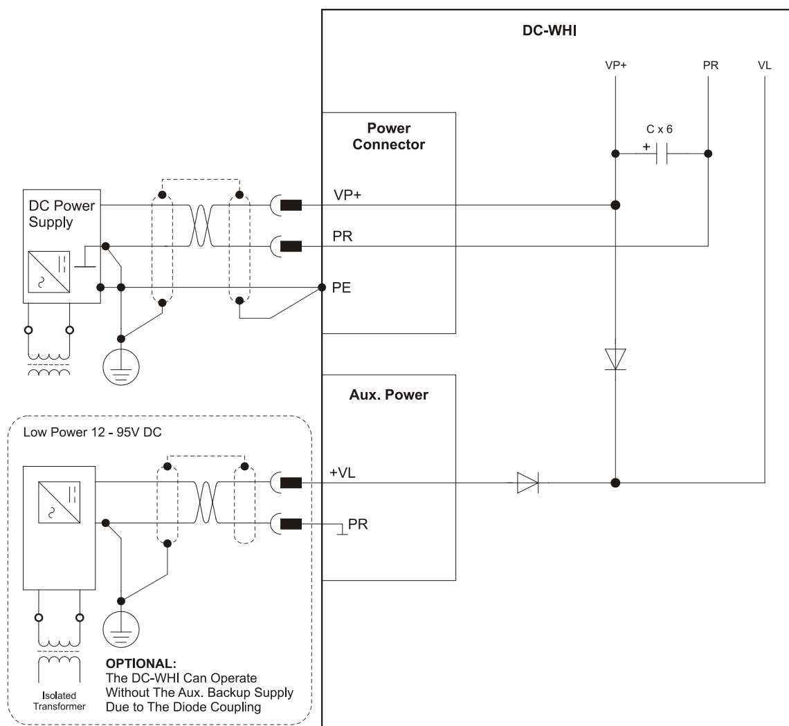
Figure 7: Shared Supply Connection Diagram
