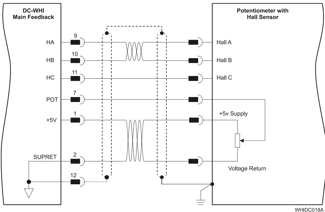
Figure 15: Main Feedback – Potentiometer Feedback with Digital Hall Sensor - Connection Diagram for Brushless Motors
