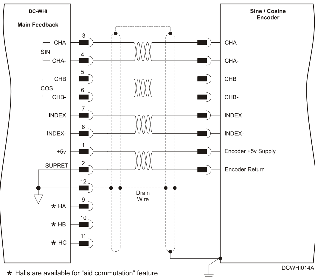
Figure 11: Main Feedback – Interpolated Analog (Sine/Cosine) Encoder Connection Diagram
