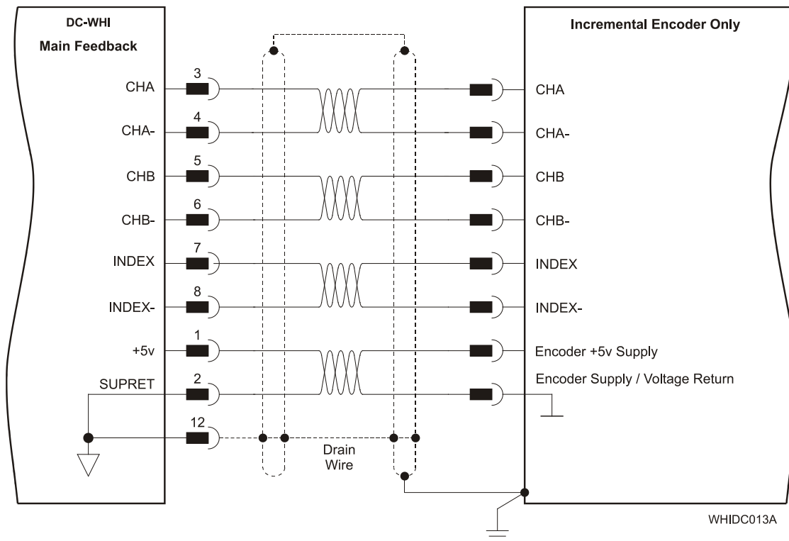
Figure 10: Main Feedback- Incremental Encoder Only Connection Diagram
