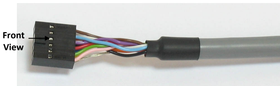
Figure 31: Single-Sided Main Feedback Cable (Part No. CBL-HDRFB-001)
