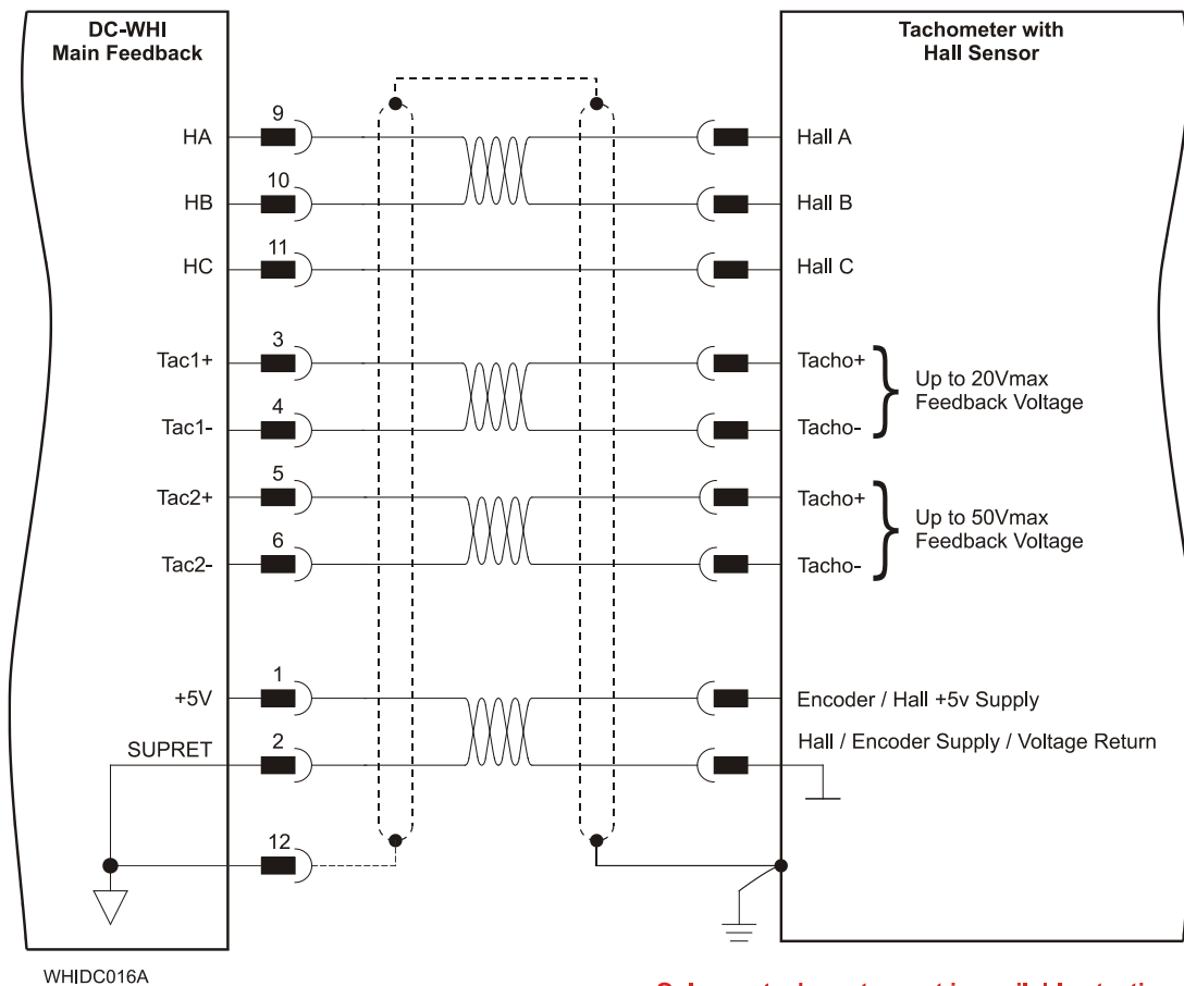
Figure 13: Main Feedback – Tachometer Feedback with Digital Hall Sensor - Connection Diagram for Brushless Motors
