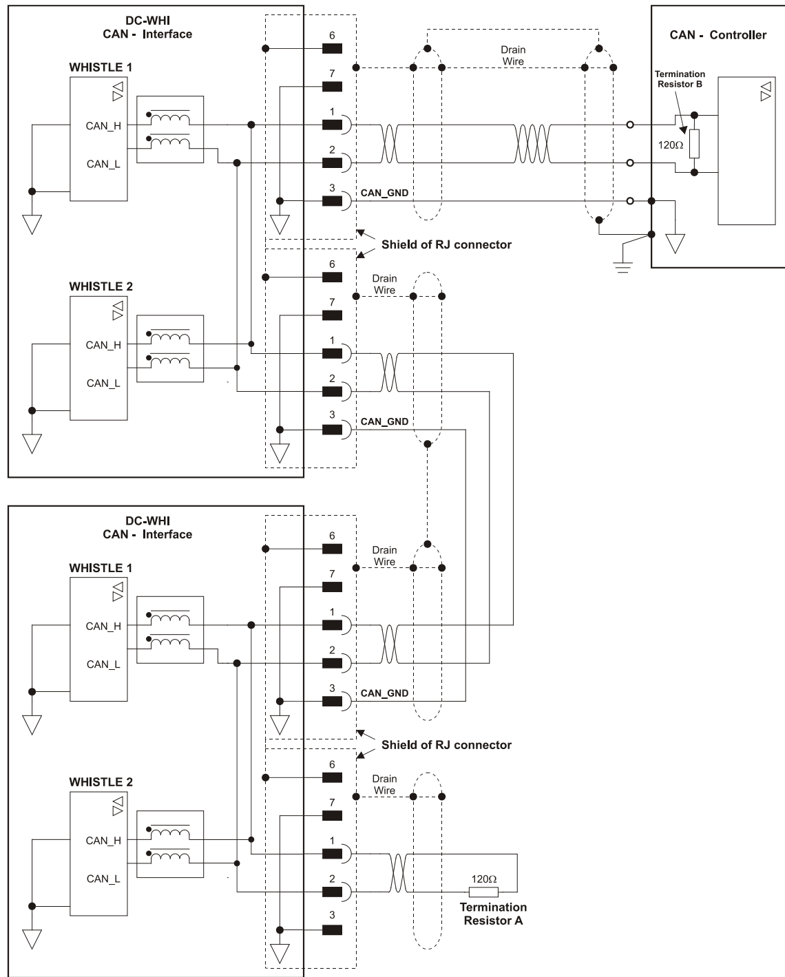
Figure 25: CAN Network Connection Diagram
