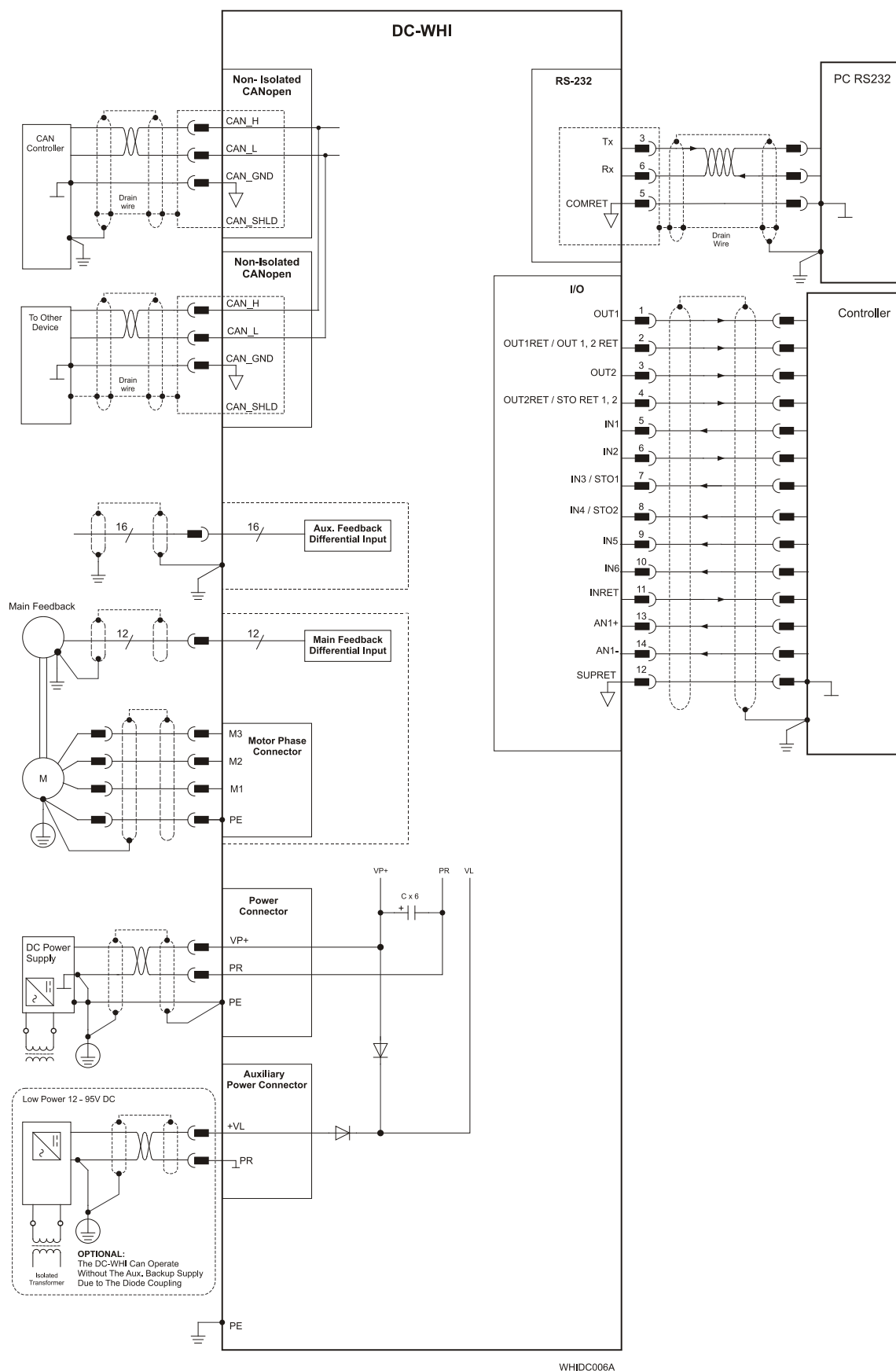
Figure 3: DC Whistle Connection Diagram
