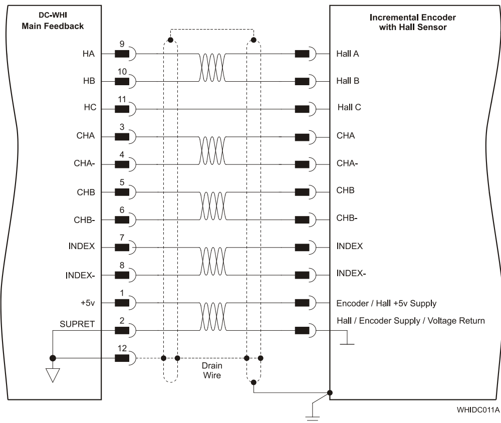
Figure 9: Main Feedback- Incremental Encoder with Digital Halls Sensors Connection Diagram
