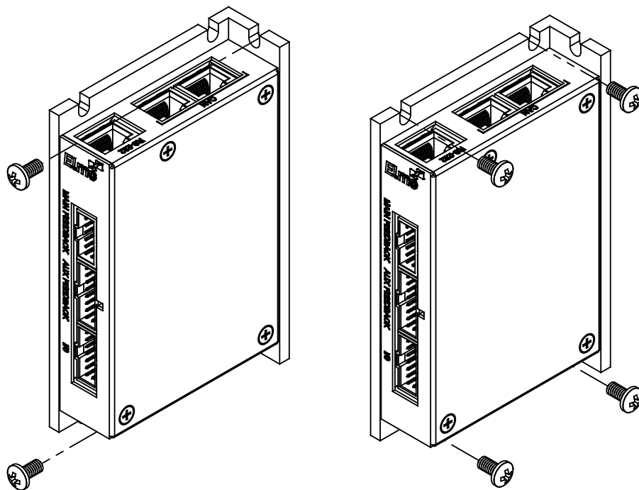
Figure 2: Mounting the DC Whistle
