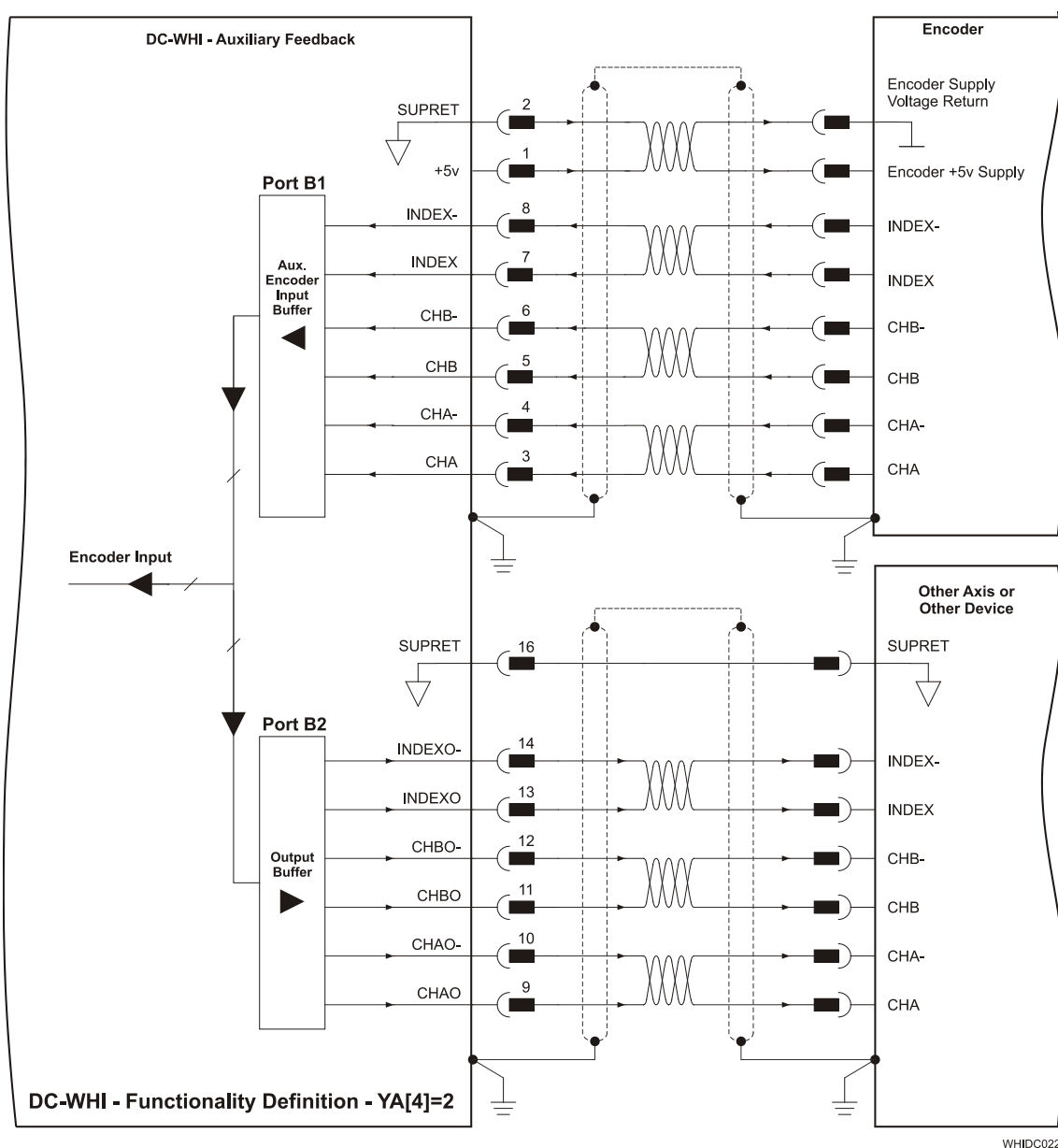
Figure 19: Differential Auxiliary Input Option on Auxiliary Feedback - Connection Diagram
