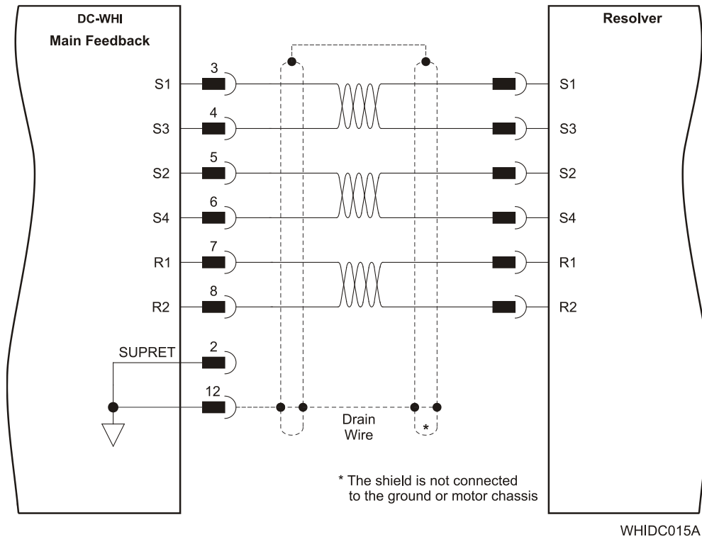
Figure 12: Main Feedback– Resolver Connection Diagram
