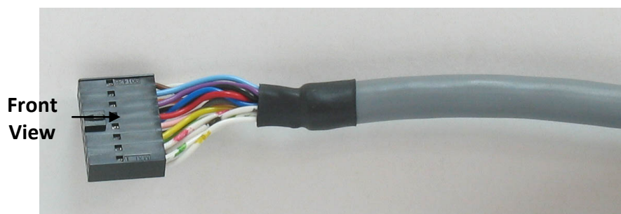
Figure 32: Single-Sided Auxiliary Feedback Cable (Part No. CBL-HDRAUX-001)
