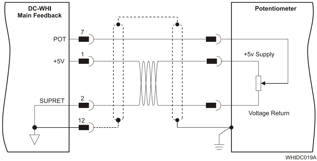
Figure 16: Main Feedback – Potentiometer Feedback Connection Diagram for Brush Motors and Voice Coils
