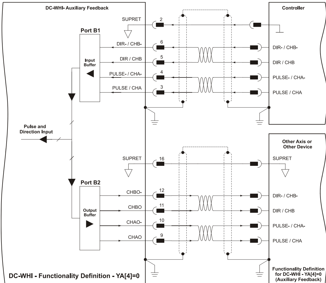
Figure 20: Pulse-and-Direction Input Option on Auxiliary Feedback - Connection Diagram
