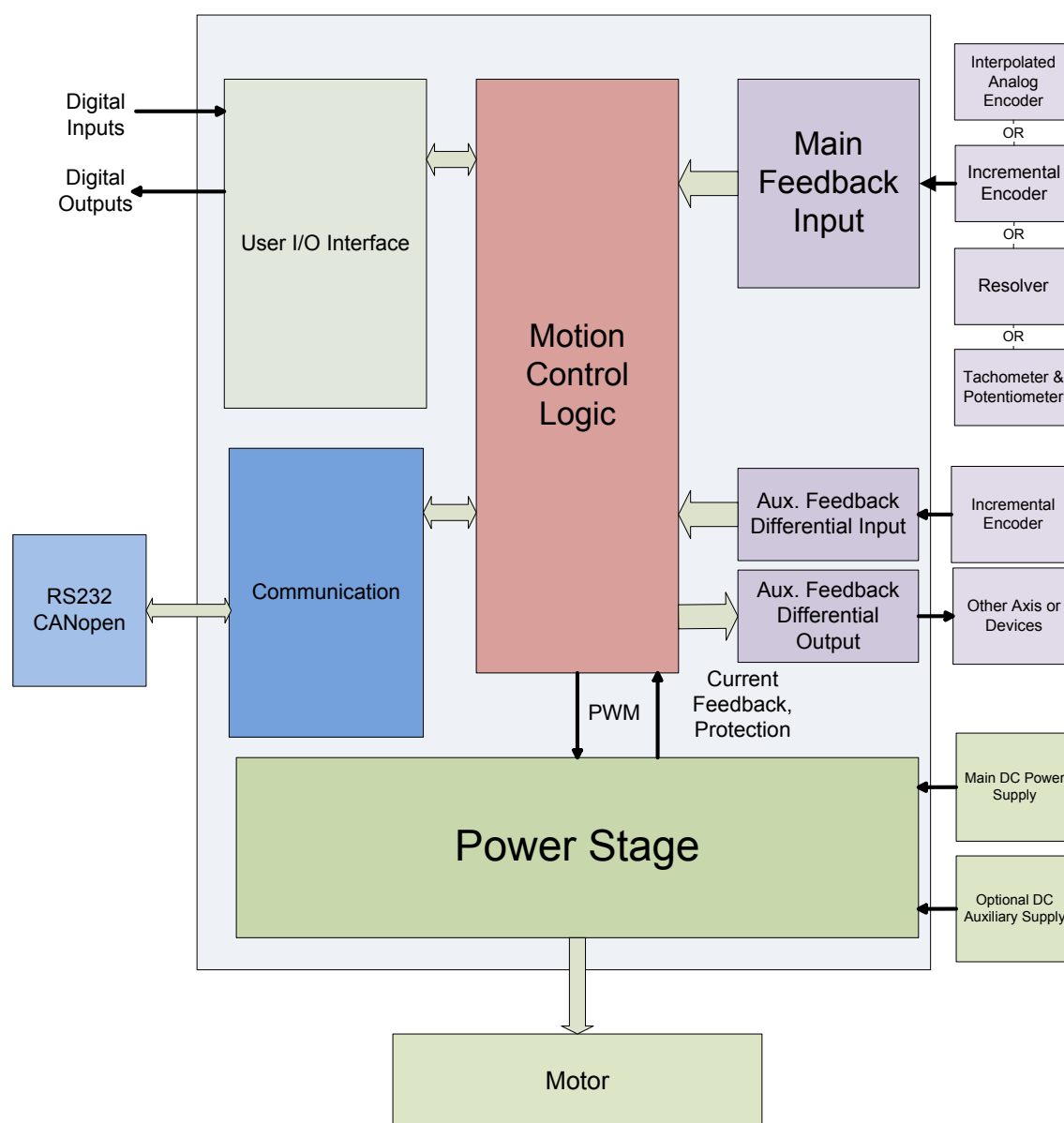
Figure 1: DC Whistle System Block Diagram
