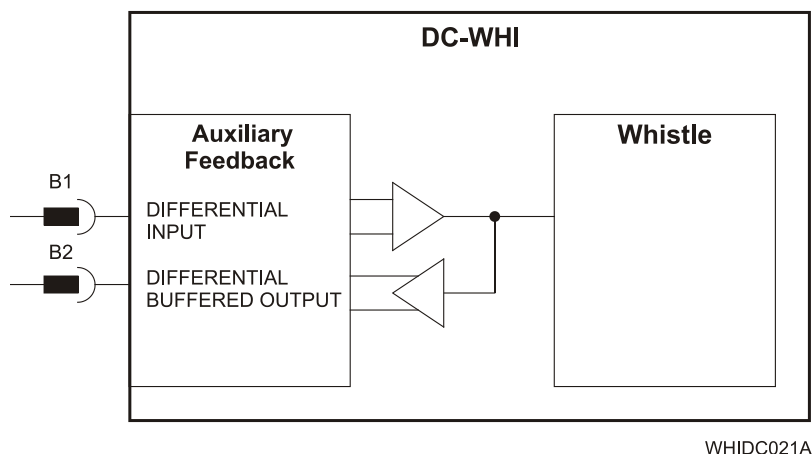
Figure 18: Differential Auxiliary Input Option - Block Diagram
