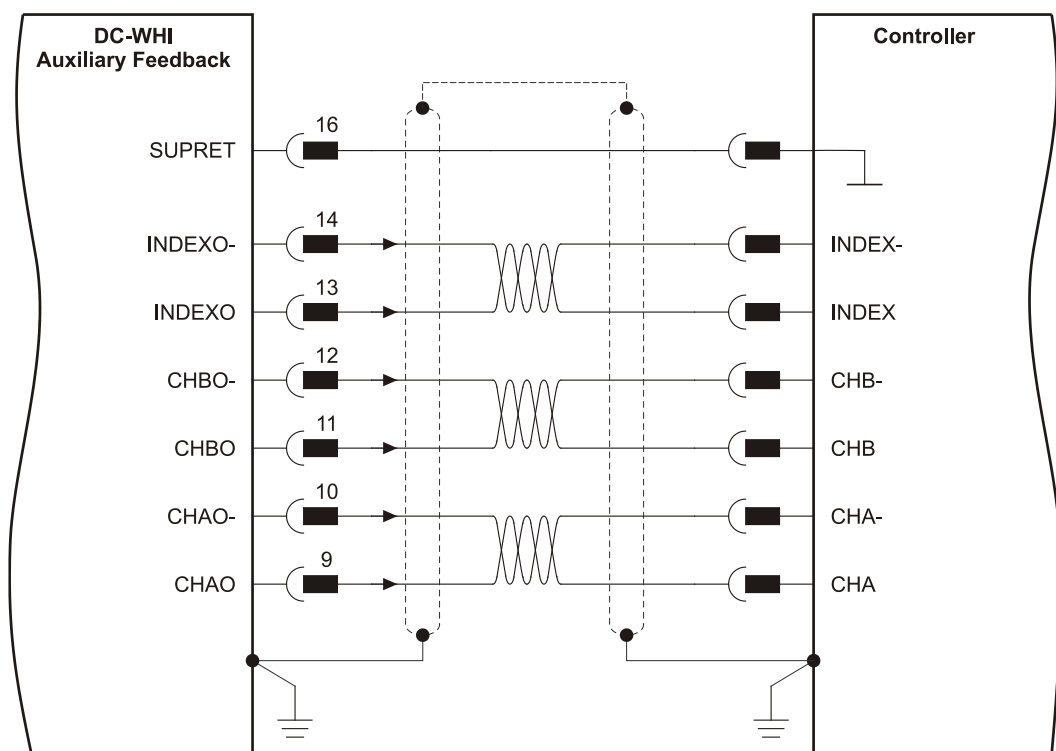
Figure 17: Emulated Encoder Outputs of the Resolver or Analog Encoder - Connection Diagram
