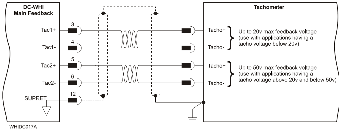
Figure 14: Main Feedback – Tachometer Feedback Connection Diagram for Brush Motors
