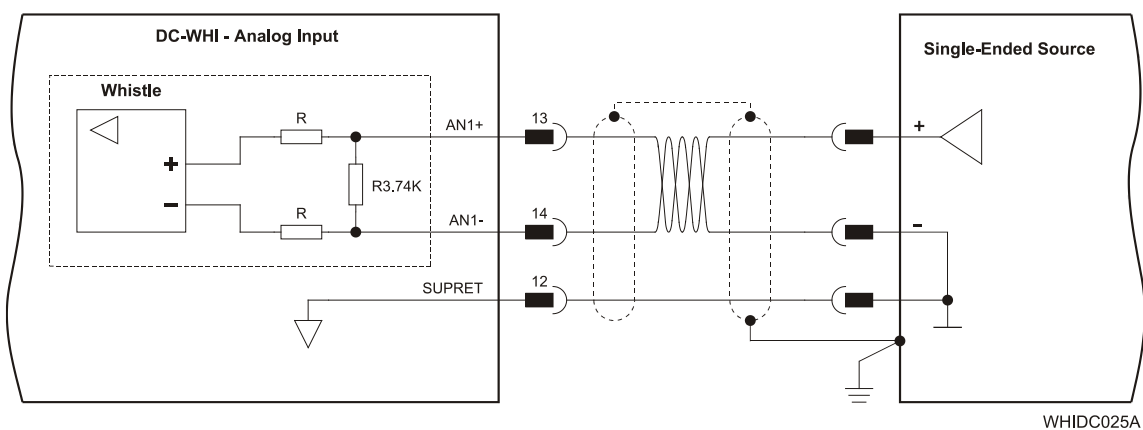
Figure 23: Analog Input with Single-Ended Source
