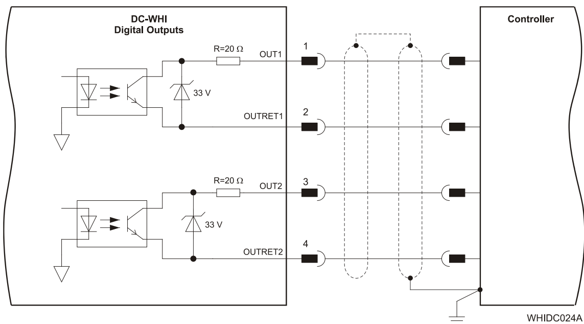
Figure 22: Digital Output Connection Diagram
