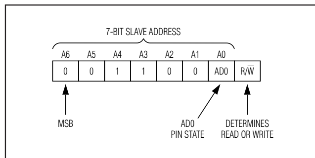
Figure 9. DS2482-101 Slave Address
