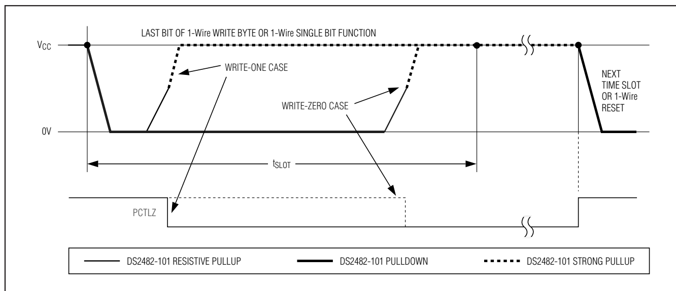
Figure 4. Low-Impedance Pullup Timing
