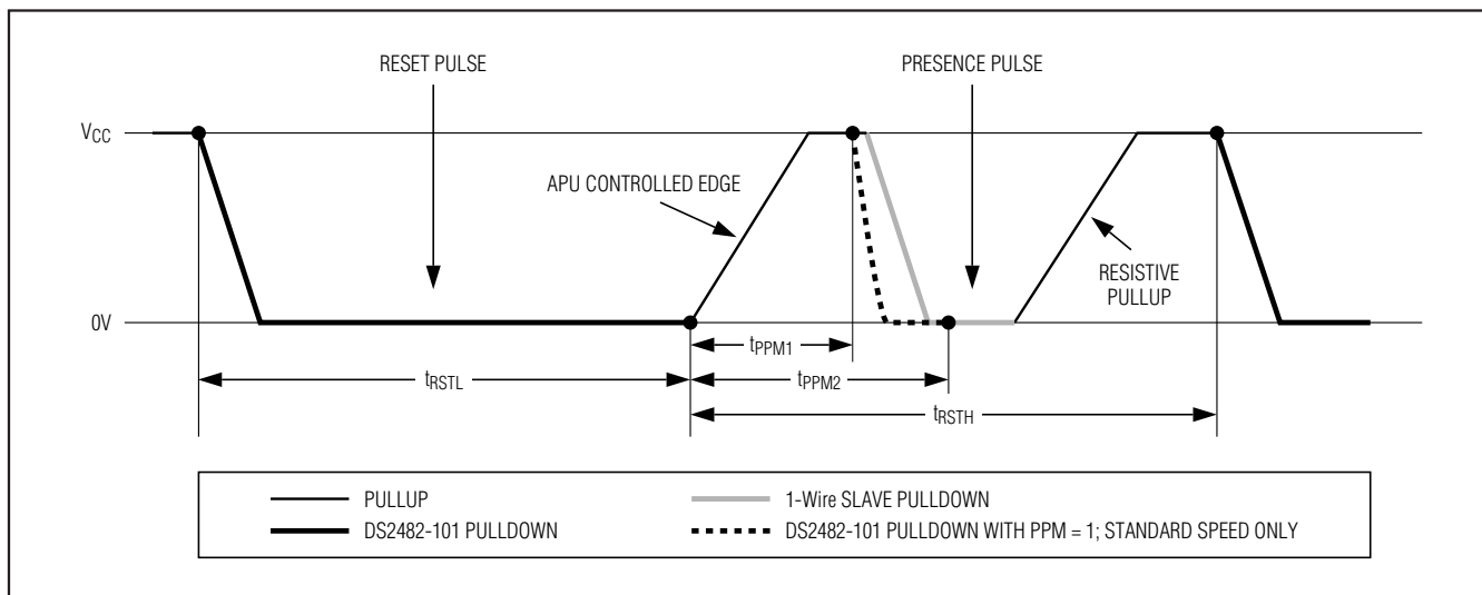
Figure 3. Presence-Pulse Masking
