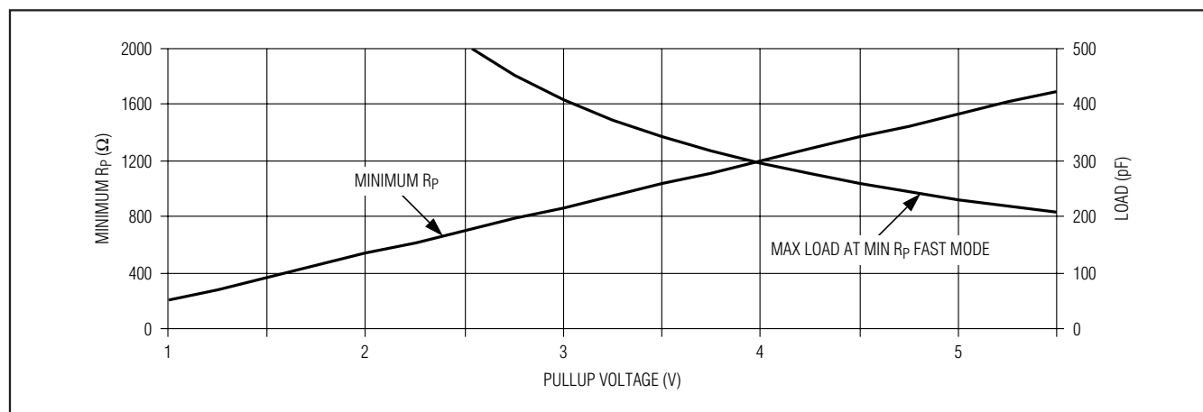
Figure 12. I 2 C Fast Speed Pullup Resistor Selection Chart
