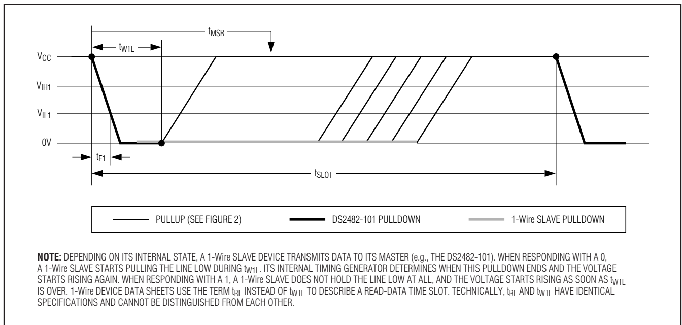
Figure 7. Write-One and Read-Data Time Slot
