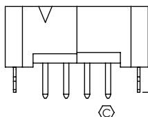
FIG. 5 T2M-104-01-XX-D-TH-WT SHOWN (SAME AS FIG. 1, EXCEPT AS SHOWN)
