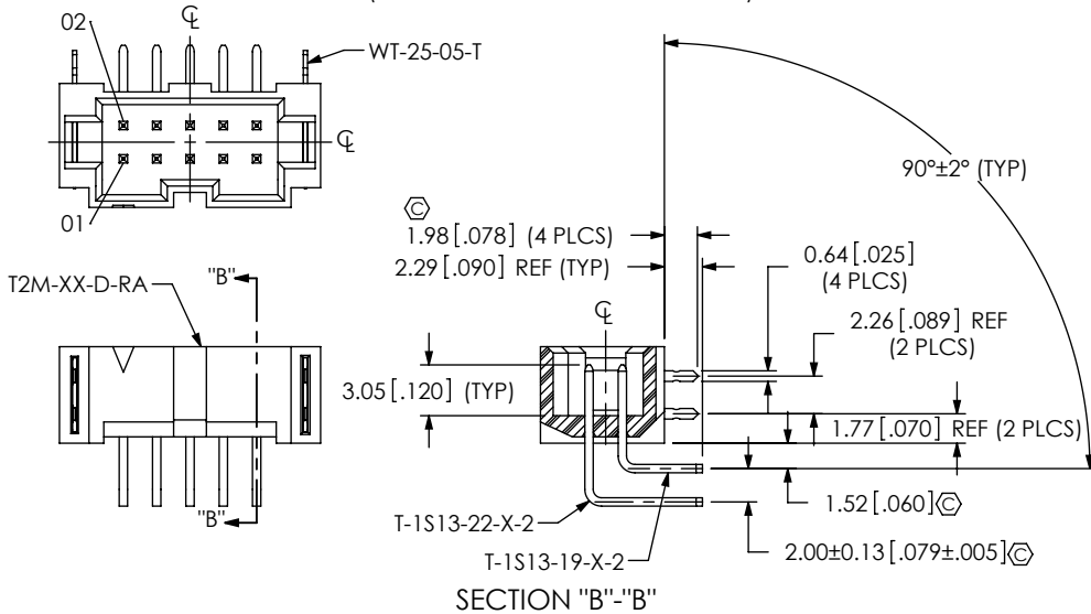
FIG. 2 T2M-105-01-XX-D-RA-WT (SAME AS FIG. 1, EXCEPT AS SHOWN)
