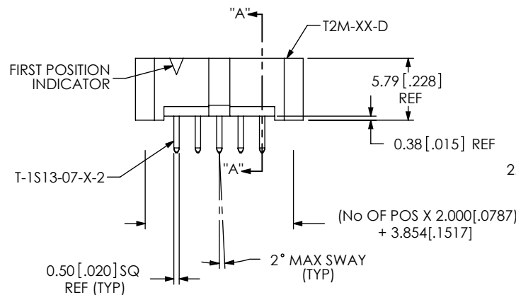
FIG. 2 T2M-105-01-XX-D-RA-WT (SAME AS FIG. 1, EXCEPT AS SHOWN)
