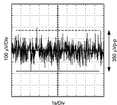
0.1 - 10 Hz Noise
