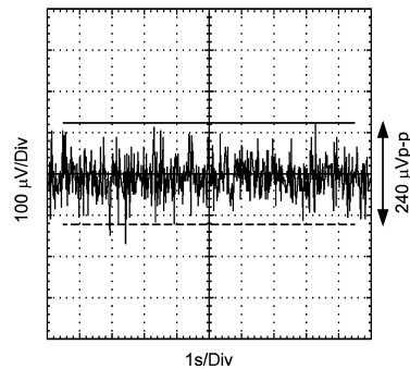
0.1 - 10 Hz Noise
