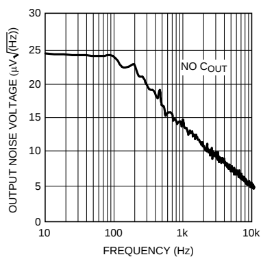
Output Voltage Noise Spectrum
