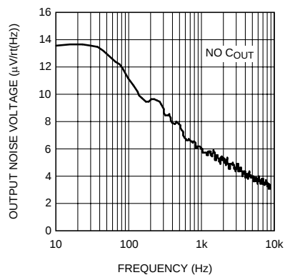
Output Voltage Noise Spectrum
