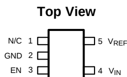
Figure 1. SOT23-5 Package
