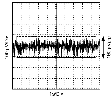
0.1 - 10 Hz Noise
