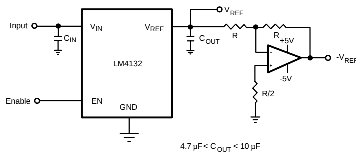
Figure 4. Voltage Reference with Complimentary Output
