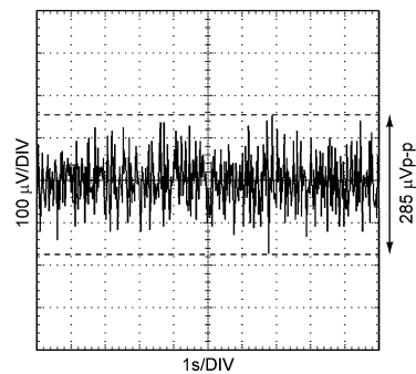
0.1-10 Hz Noise Spectrum
