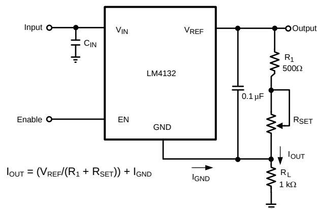
Figure 6. Programmable Current Source
