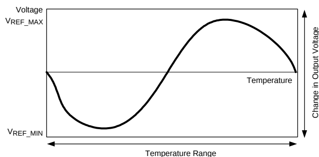
Figure 3. Illustrative V_{REF} vs Temperature Profile
