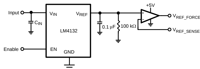
Figure 5. Precision Voltage Reference with Force and Sense Output
