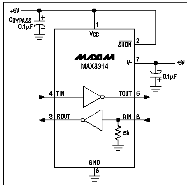
Figure 11. The MAX3314E runs off of \pm 5V supplies, but does not have charge-pump doublers and inverters. This makes the part smaller, cheaper, and RS-232-compatible, but not RS-232-compliant.
