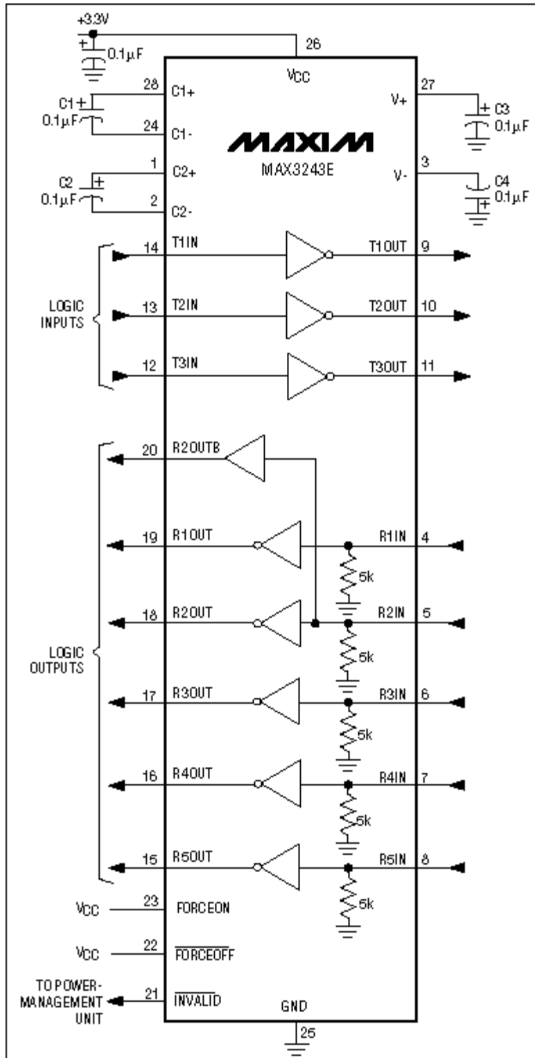
Figure 9. The MAX3243 has an extra receiver, R2OUTB, which remains active even while the other receivers are put into a high-Z output state.
