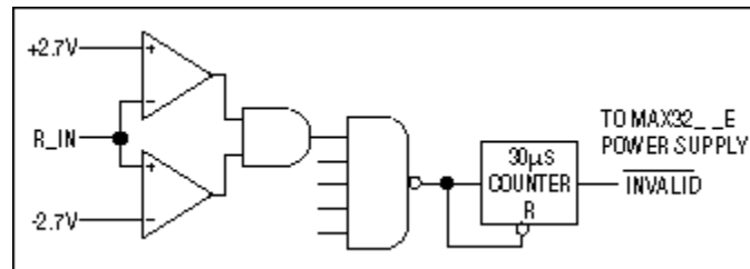
Figure 4. Autoshtutdown is exited if any receiver exceeds \pm 2.7V .
