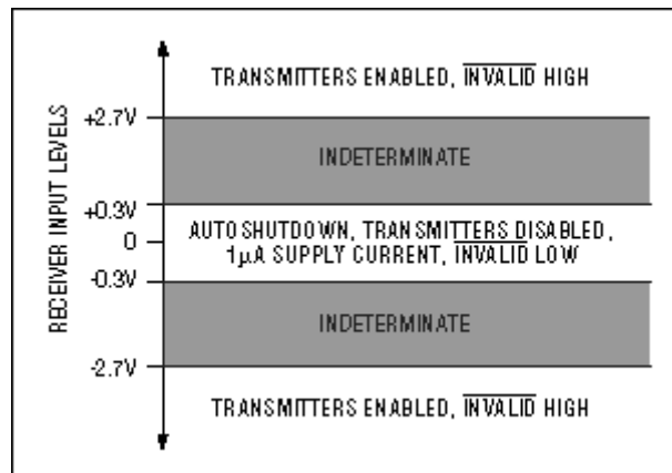
Figure 5. The trip levels for entering and exiting Autoshtutdown
