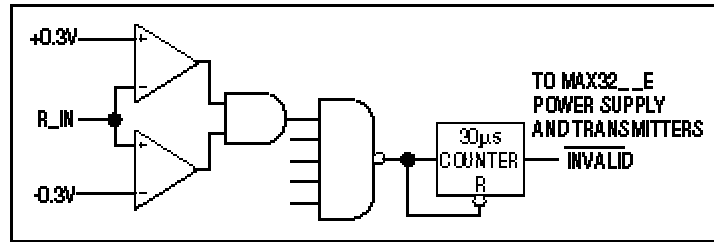
Figure 3. Autoshtutdown is entered if all receivers' inputs are between \pm 0.3V for at least 30\mu S .
