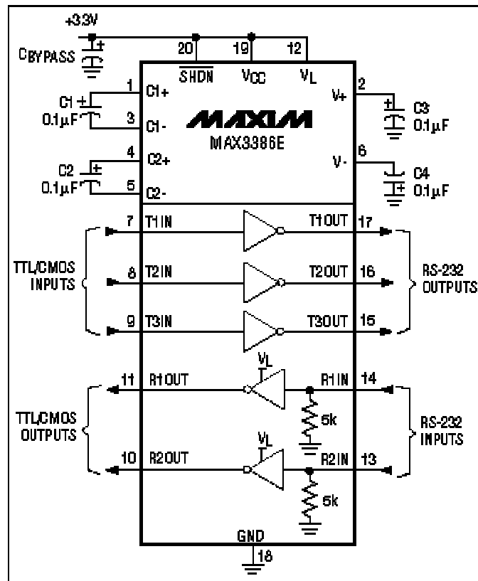
Figure 10. The MAX3386E includes a VI pin that allows the logic thresholds to be programmed for mixed-voltage systems.
